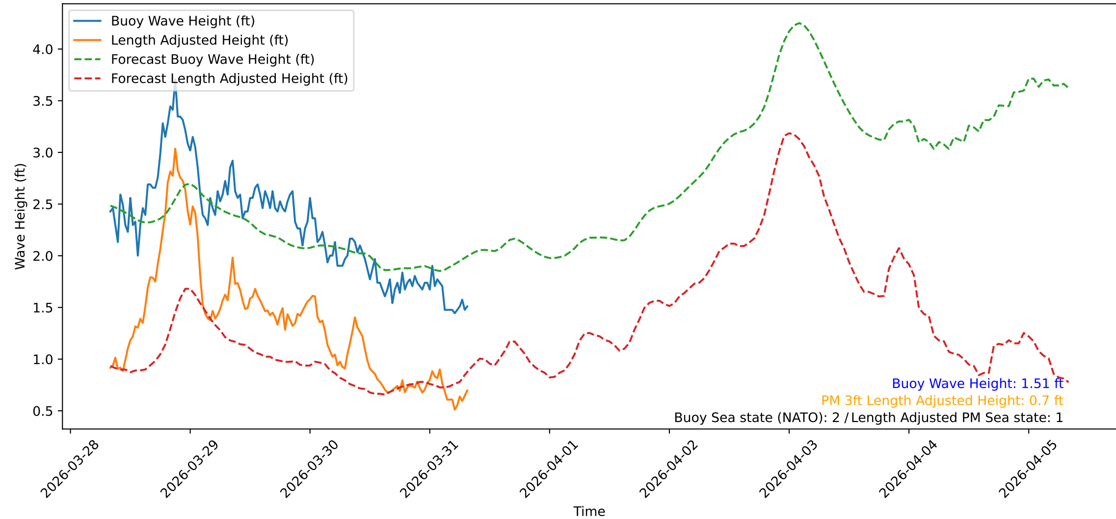
Wave Heights over Time for Green Beach at 2026-03-31 08:11:12
