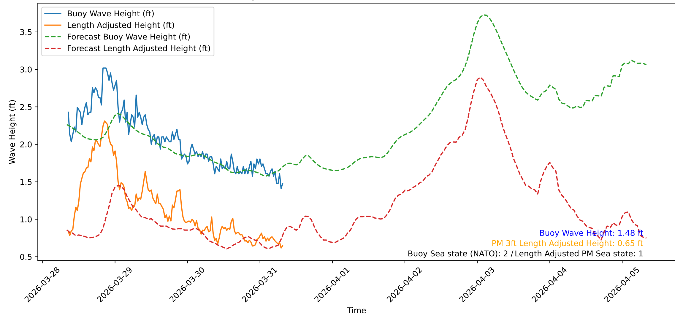
Wave Heights over Time for Red Beach at 2026-03-31 08:10:47
