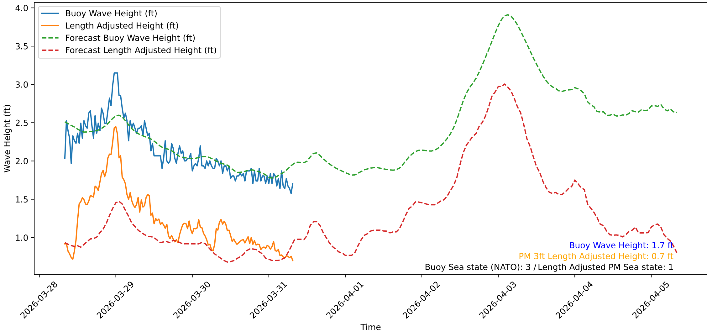
Wave Heights over Time for Oceanside Harbor at 2026-03-31 08:10:31
