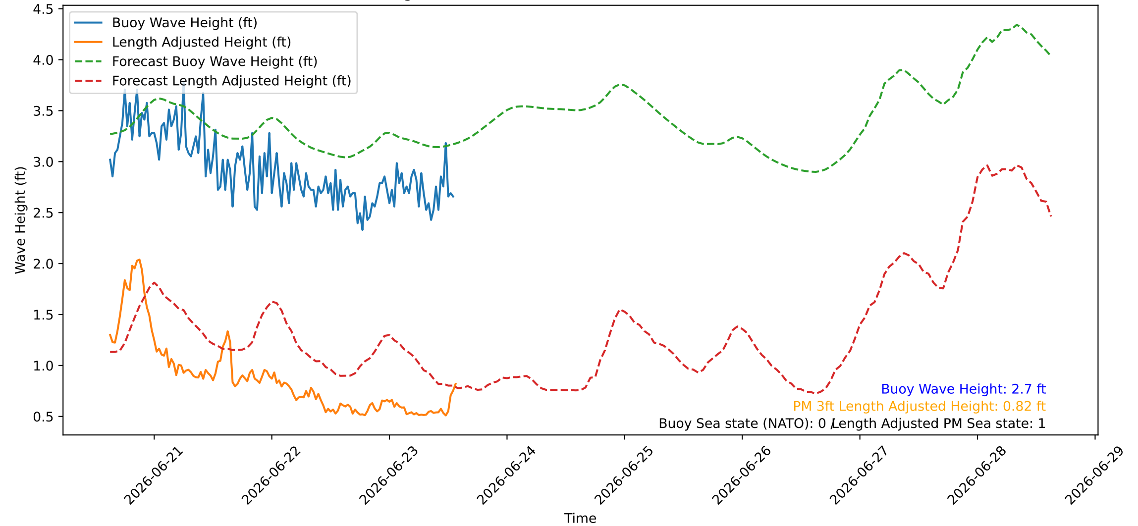
Wave Heights over Time for Red Beach at 2026-06-23 14:50:46
