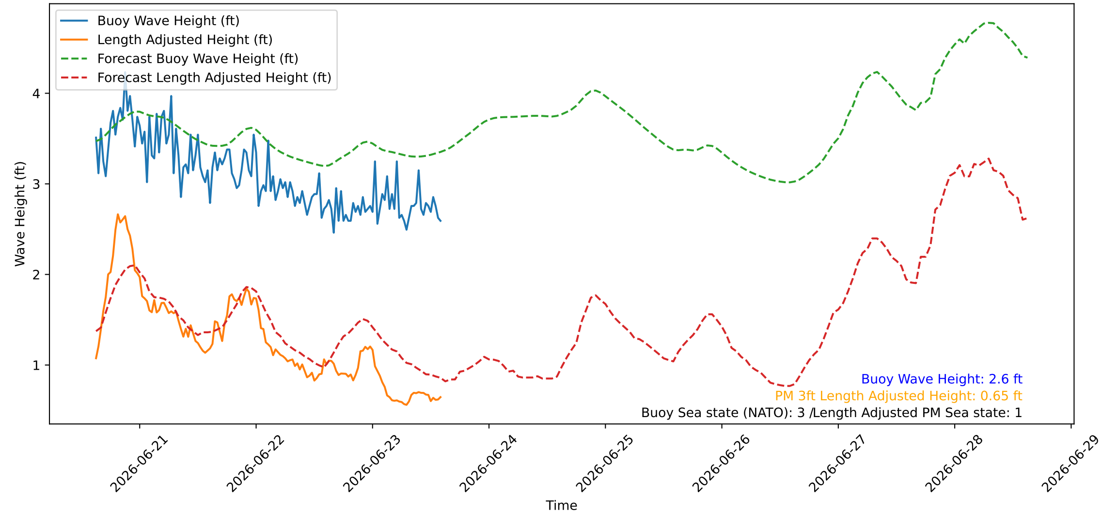
Wave Heights over Time for Green Beach at 2026-06-23 14:51:08
