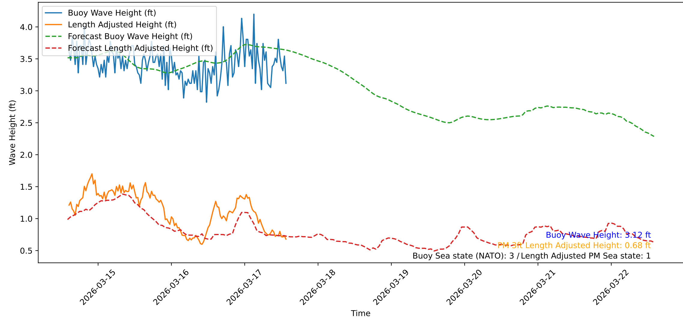
Wave Heights over Time for Green Beach at 2026-03-17 14:21:42
