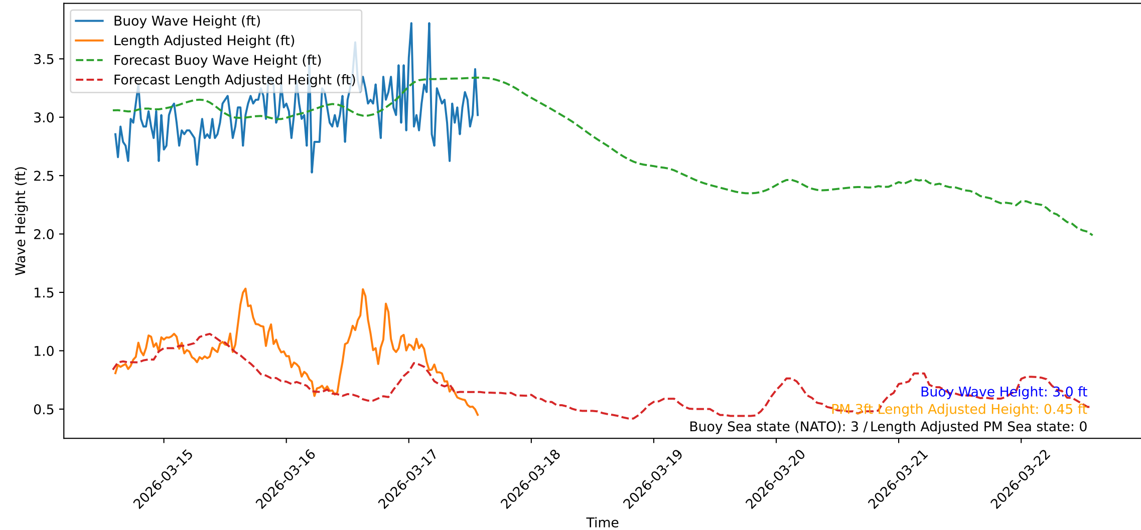
Wave Heights over Time for Red Beach at 2026-03-17 14:21:07
