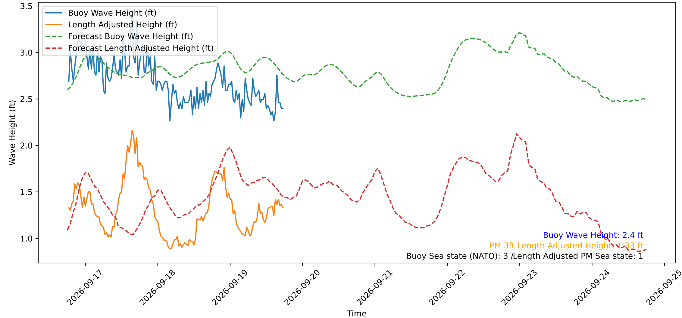
Wave Heights over Time for Red Beach at 2026-09-19 18:20:50
