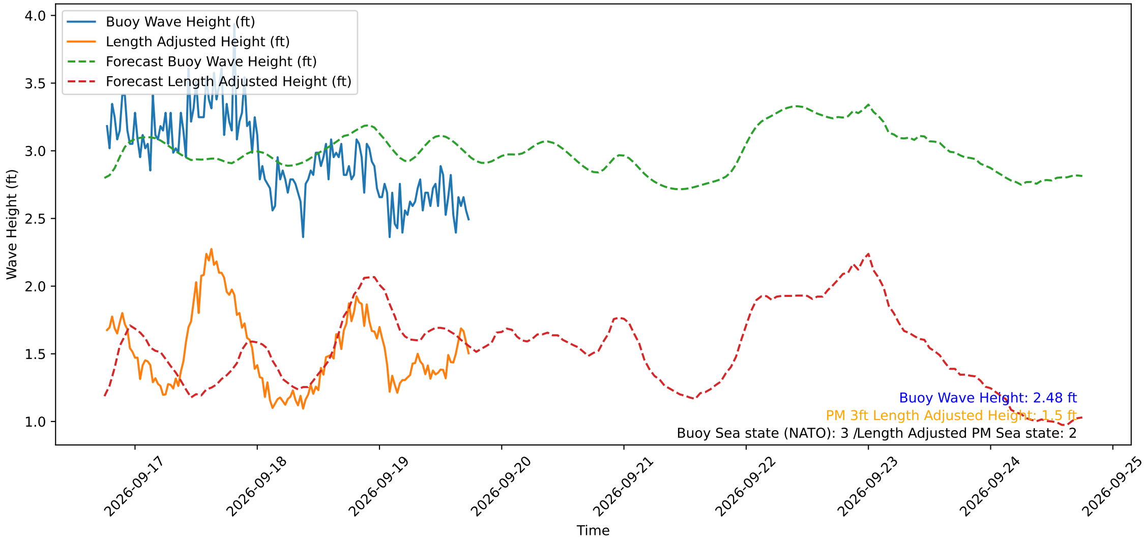
Wave Heights over Time for Oceanside Harbor at 2026-09-19 18:20:29
