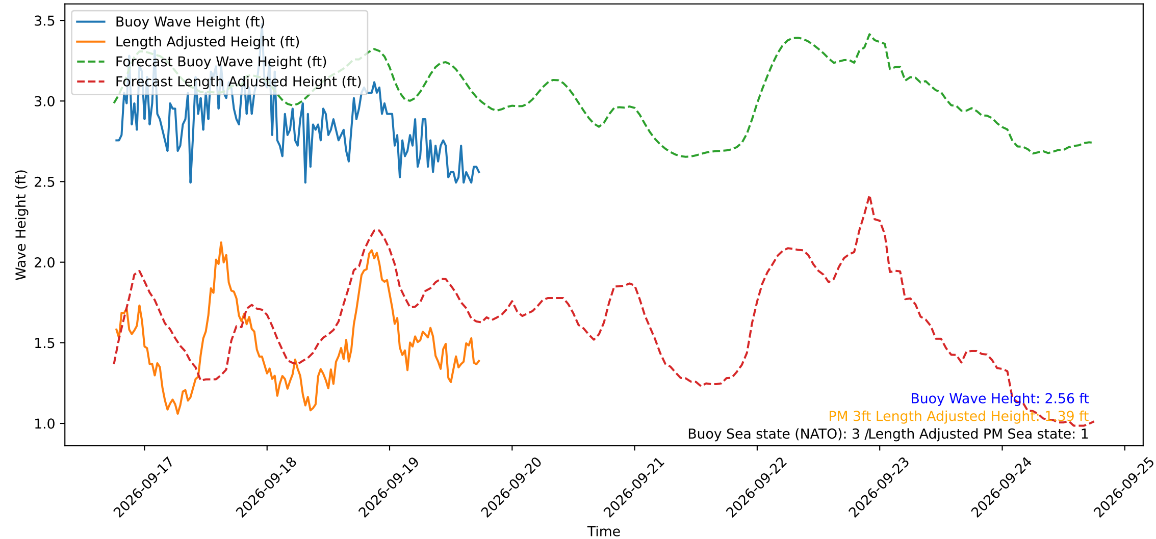
Wave Heights over Time for Green Beach at 2026-09-19 18:21:15
