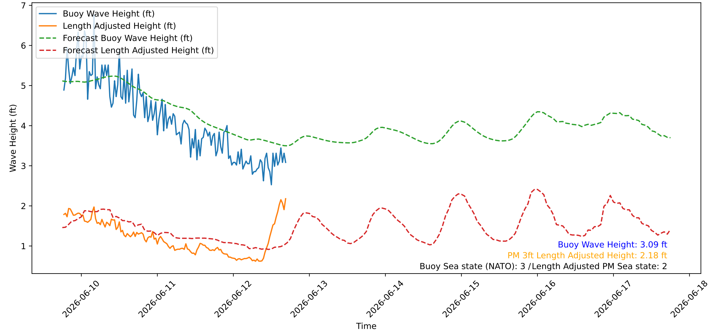
Wave Heights over Time for Red Beach at 2026-06-12 18:00:46
