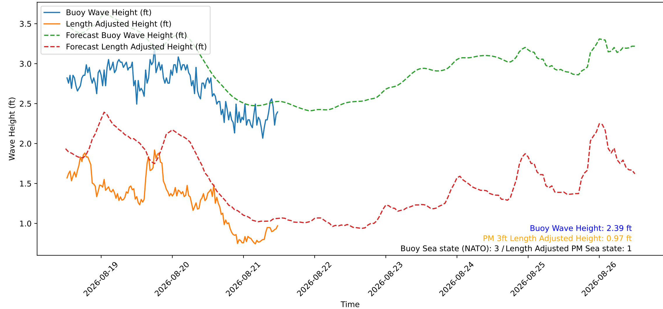
Wave Heights over Time for Red Beach at 2026-08-21 12:20:47
