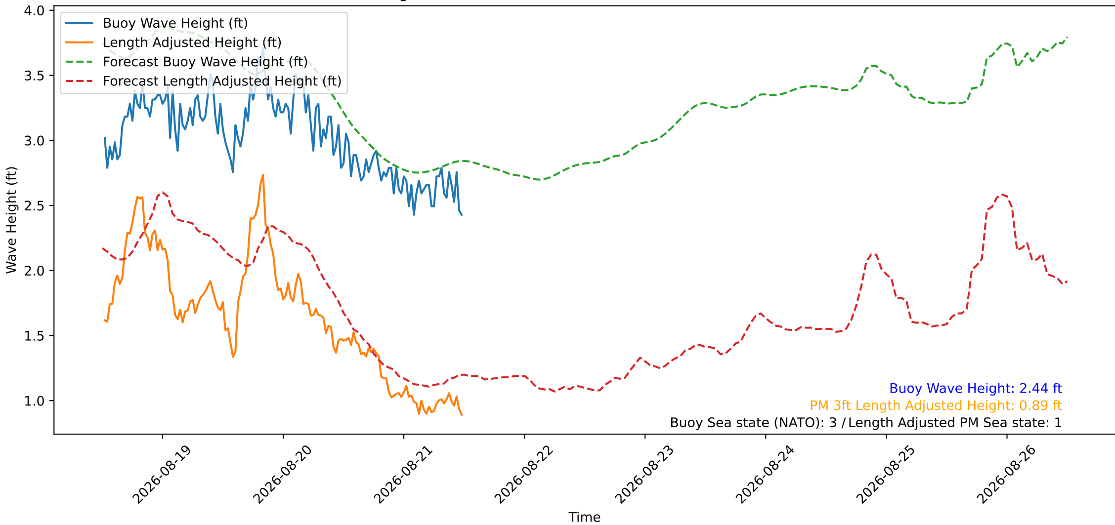
Wave Heights over Time for Green Beach at 2026-08-21 12:21:10
