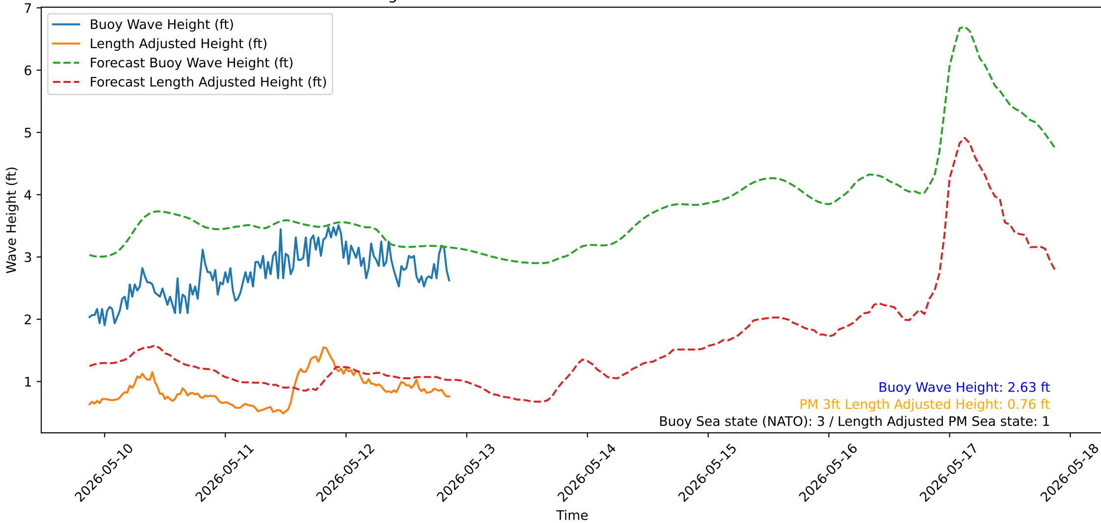
Wave Heights over Time for Green Beach at 2026-05-12 21:11:14
