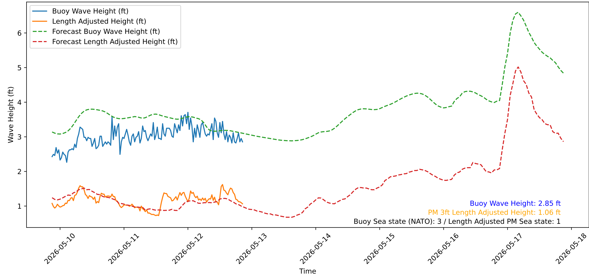
Wave Heights over Time for Oceanside Harbor at 2026-05-12 21:10:32
