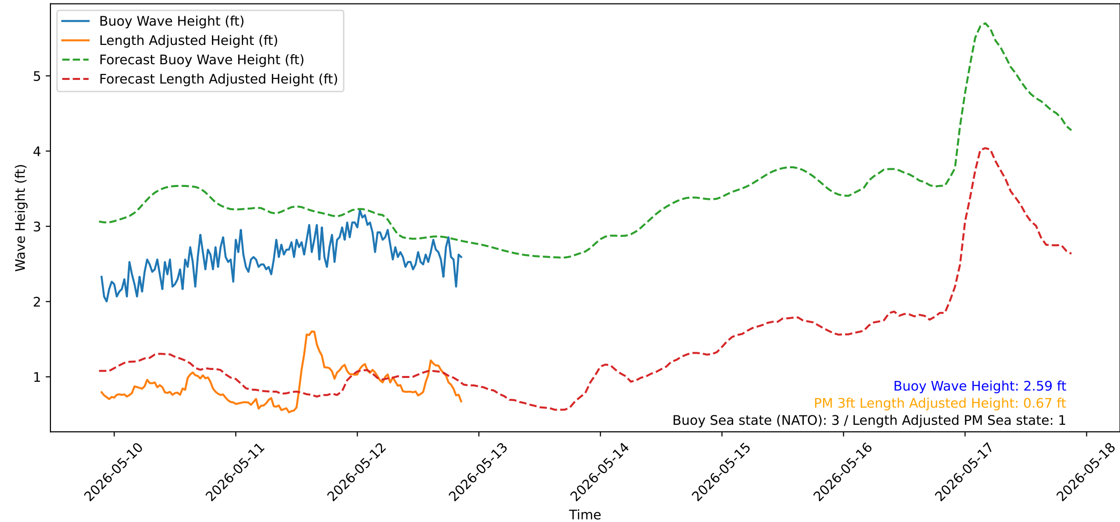
Wave Heights over Time for Red Beach at 2026-05-12 21:10:51
