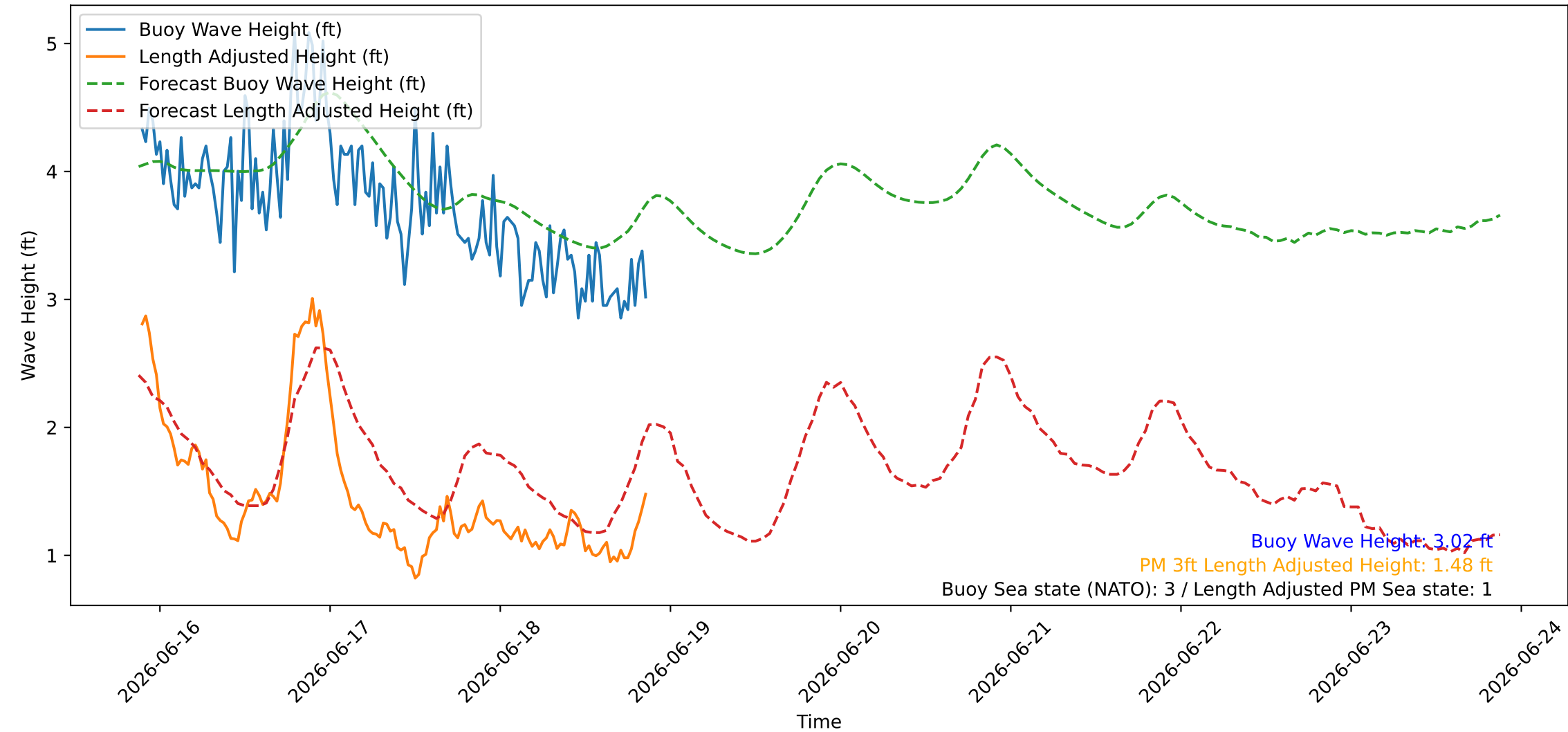
Wave Heights over Time for Green Beach at 2026-06-18 21:21:09
