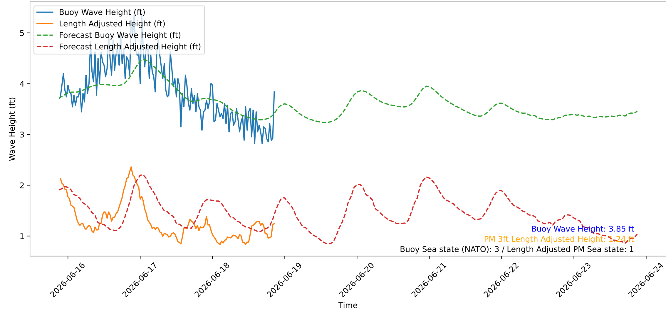
Wave Heights over Time for Red Beach at 2026-06-18 21:20:46
