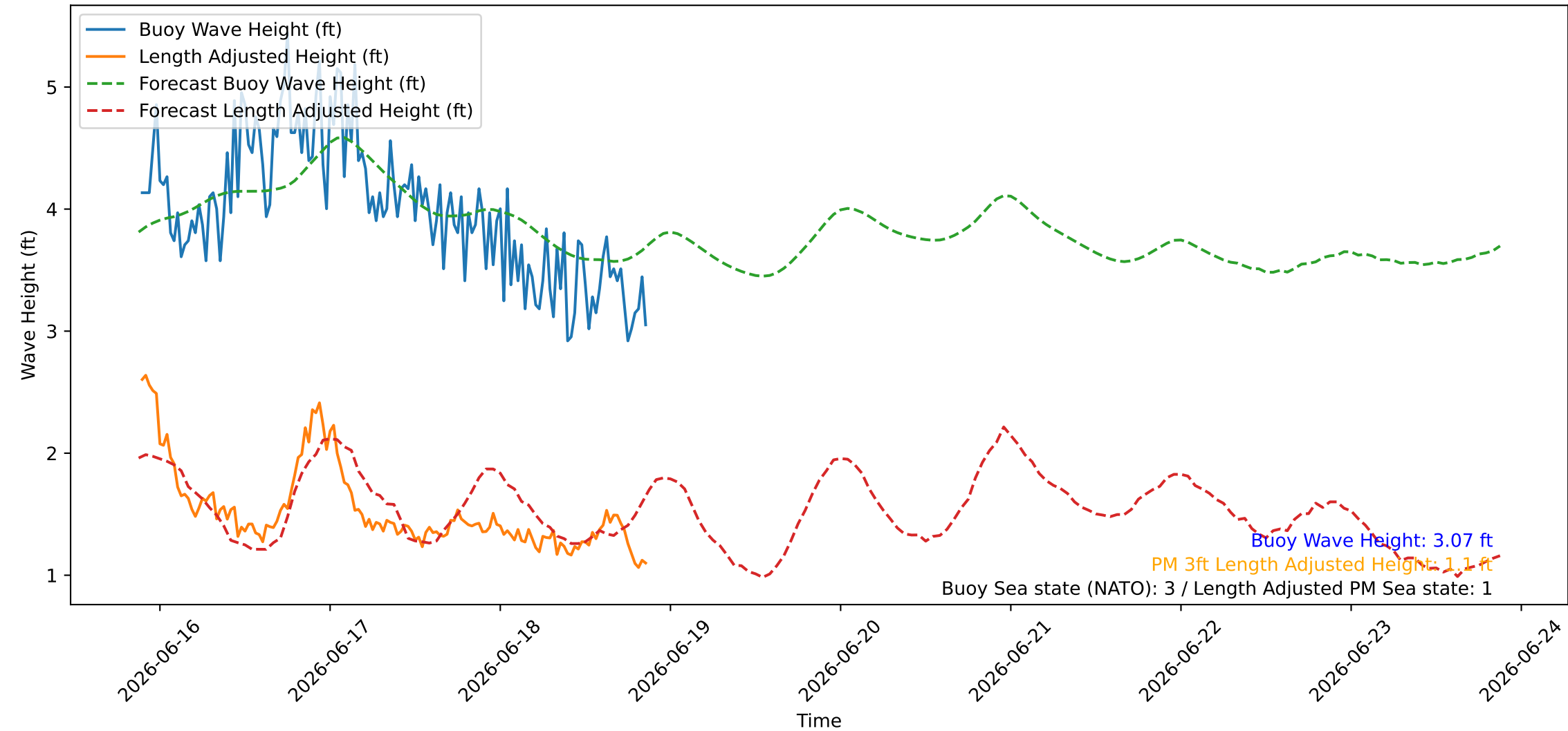
Wave Heights over Time for Oceanside Harbor at 2026-06-18 21:20:26
