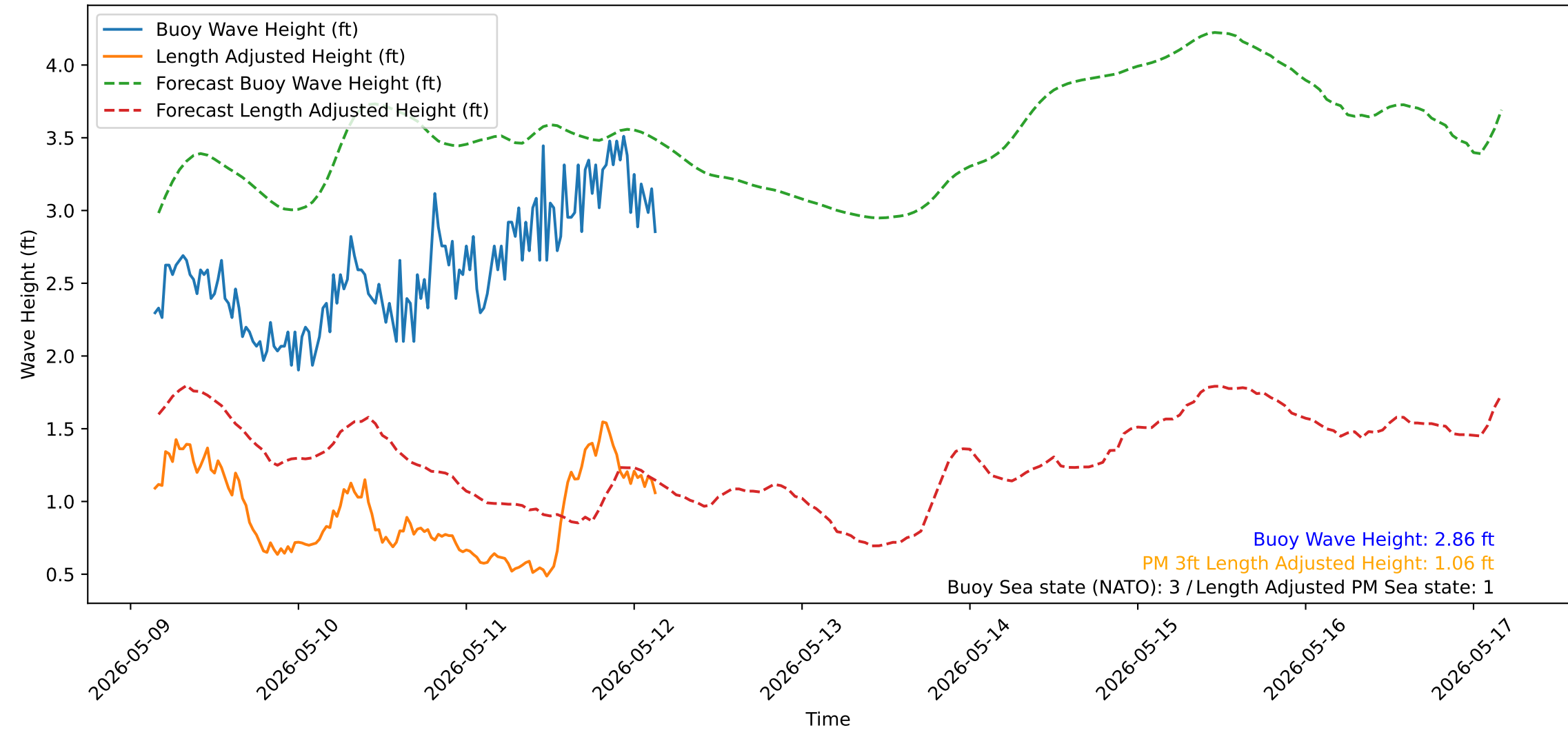
Wave Heights over Time for Green Beach at 2026-05-12 03:41:13
