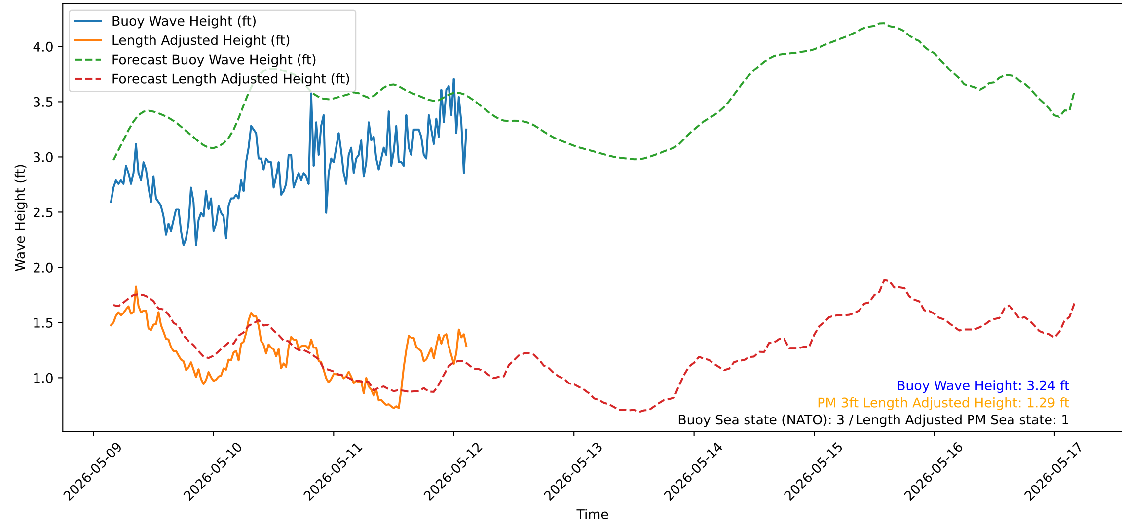
Wave Heights over Time for Oceanside Harbor at 2026-05-12 03:40:31
