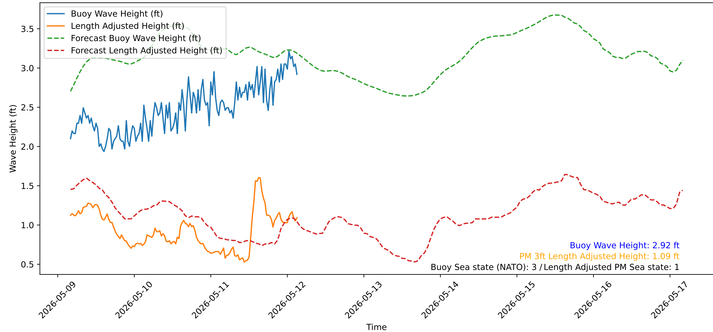
Wave Heights over Time for Red Beach at 2026-05-12 03:40:51
