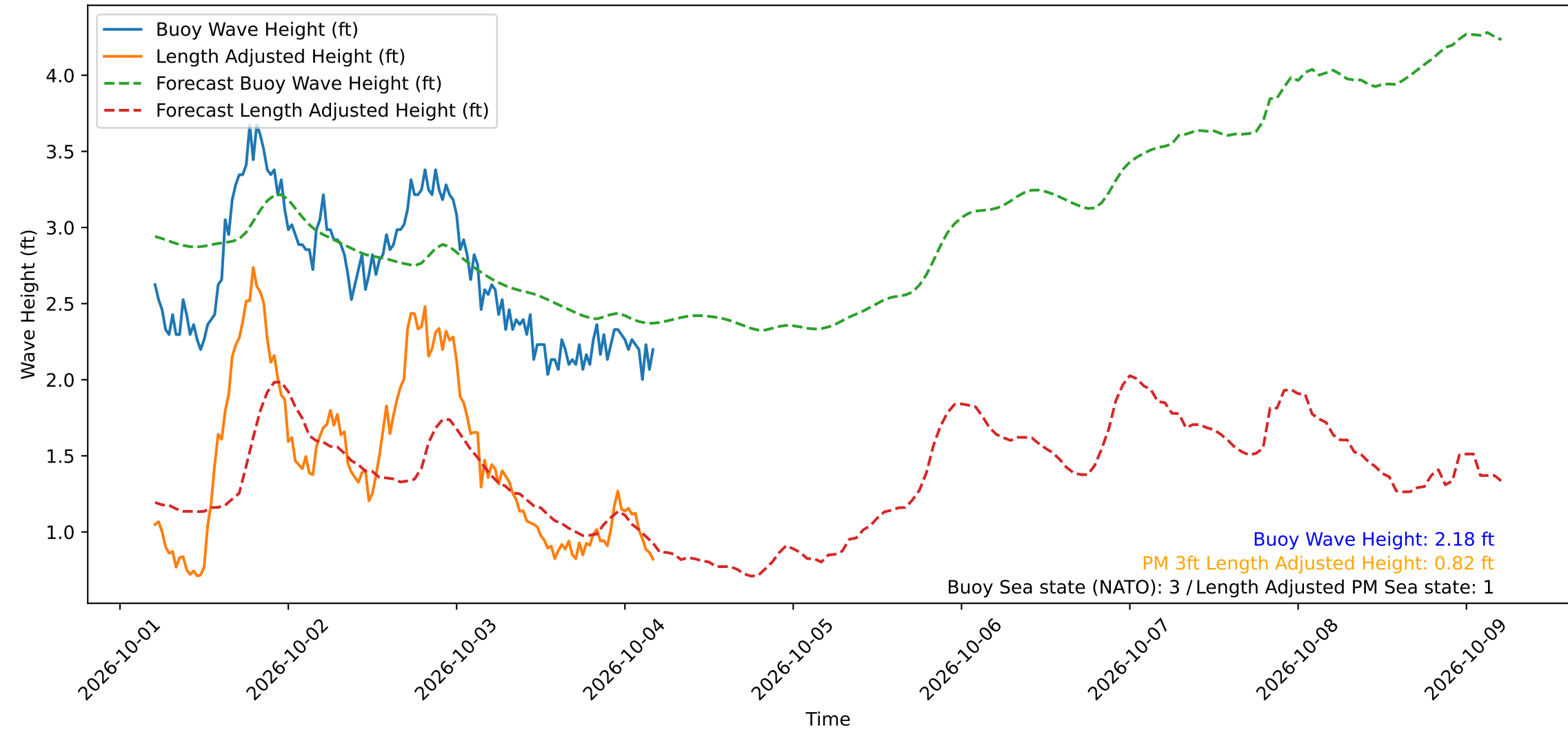
Wave Heights over Time for Green Beach at 2026-10-04 04:51:15
