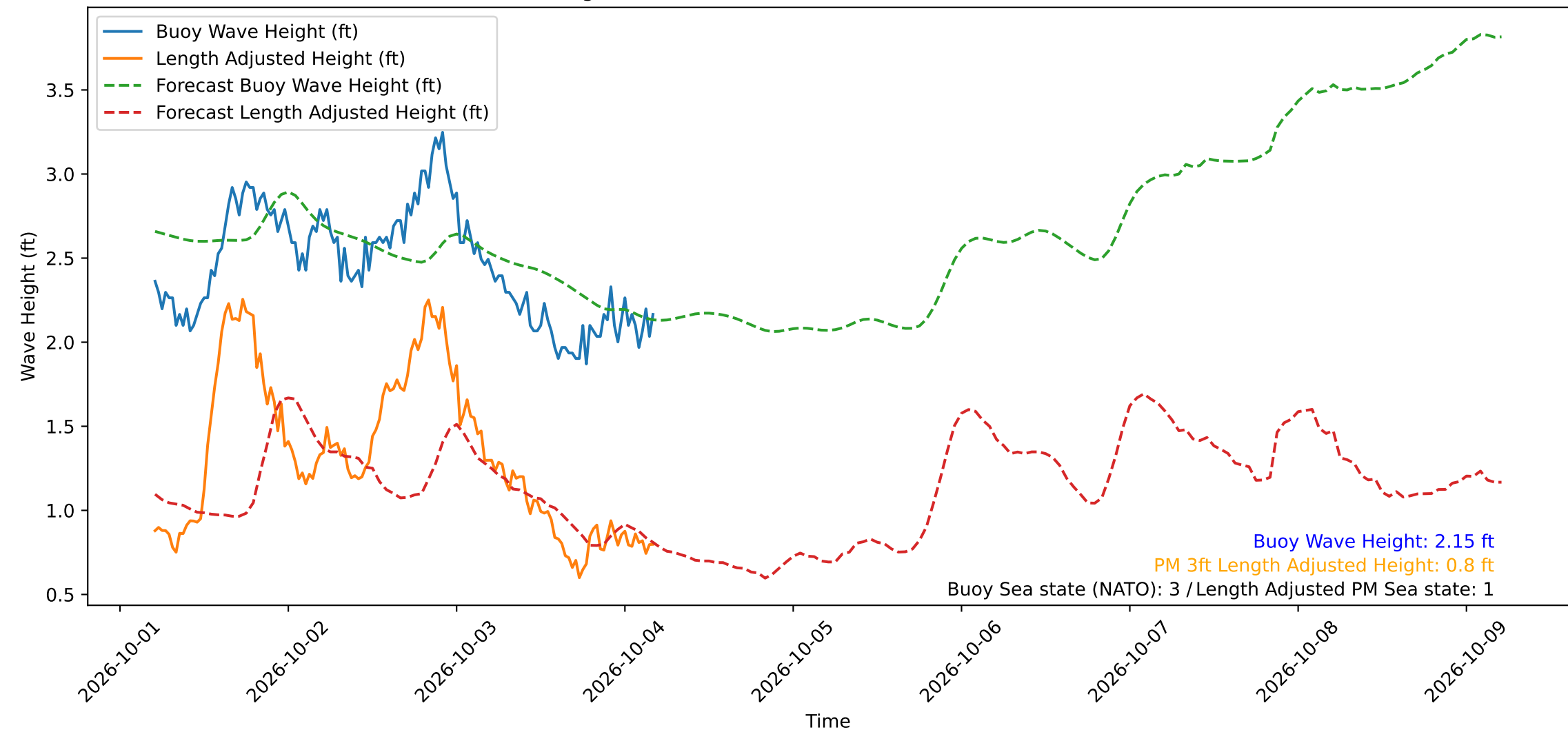
Wave Heights over Time for Red Beach at 2026-10-04 04:50:51
