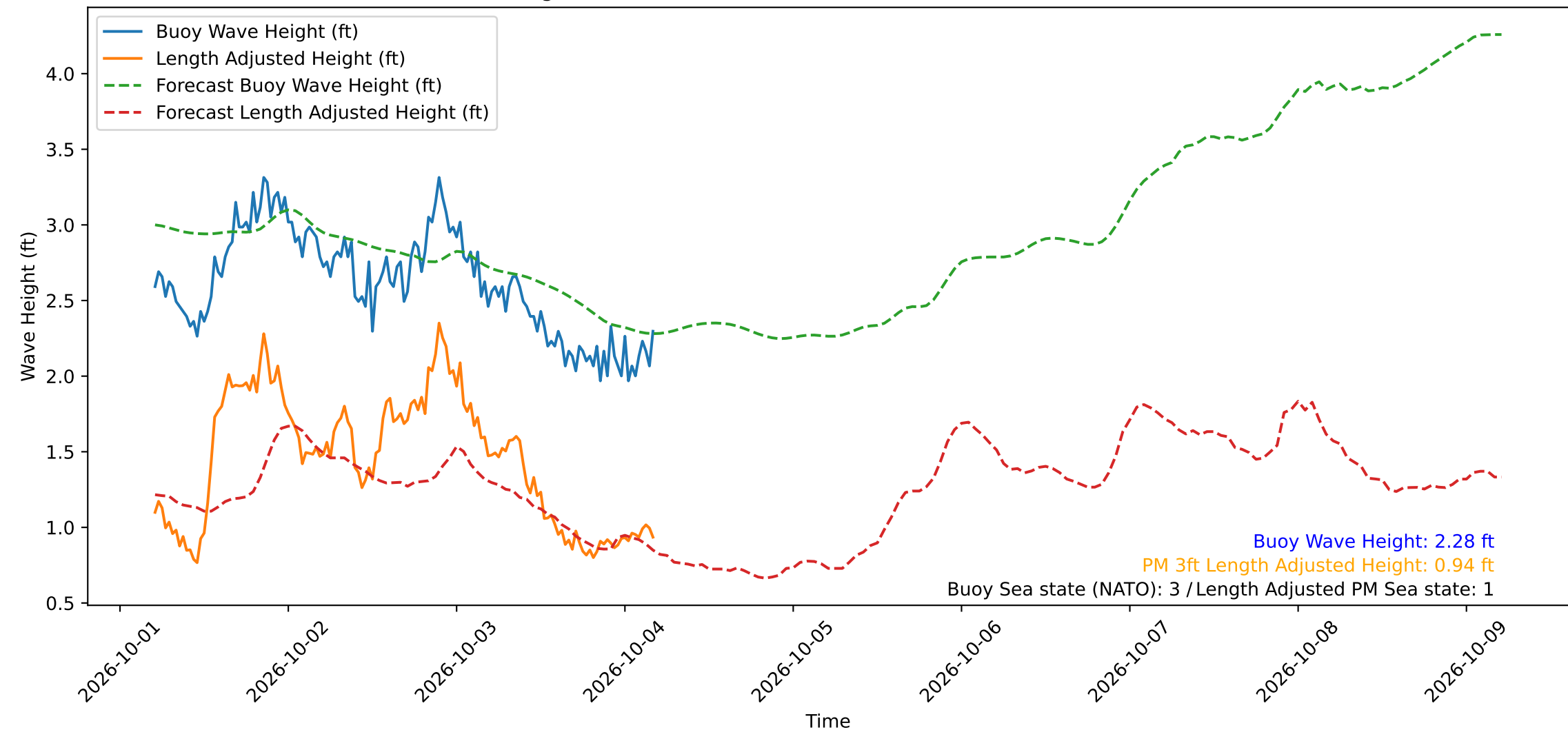
Wave Heights over Time for Oceanside Harbor at 2026-10-04 04:50:30
