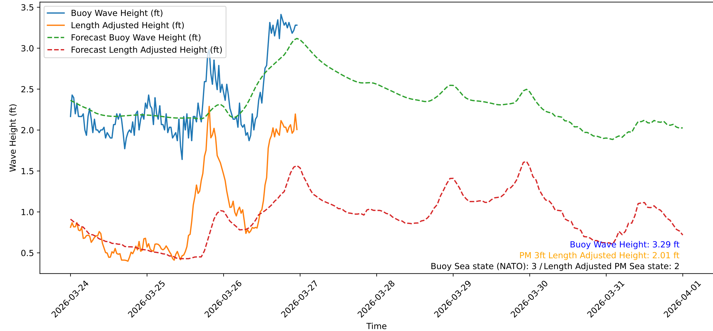
Wave Heights over Time for Green Beach at 2026-03-26 23:51:09
