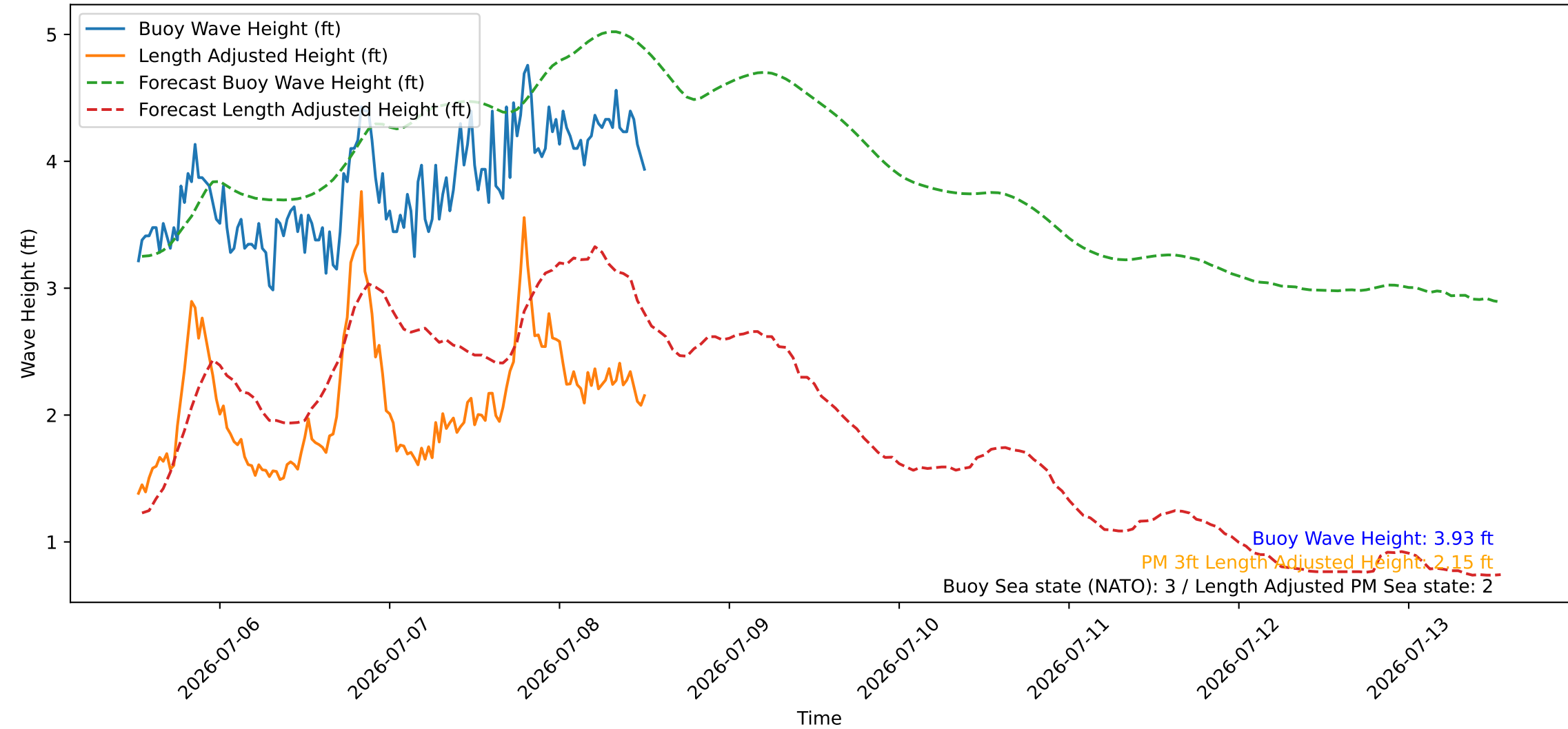
Wave Heights over Time for Green Beach at 2026-07-08 12:41:08
