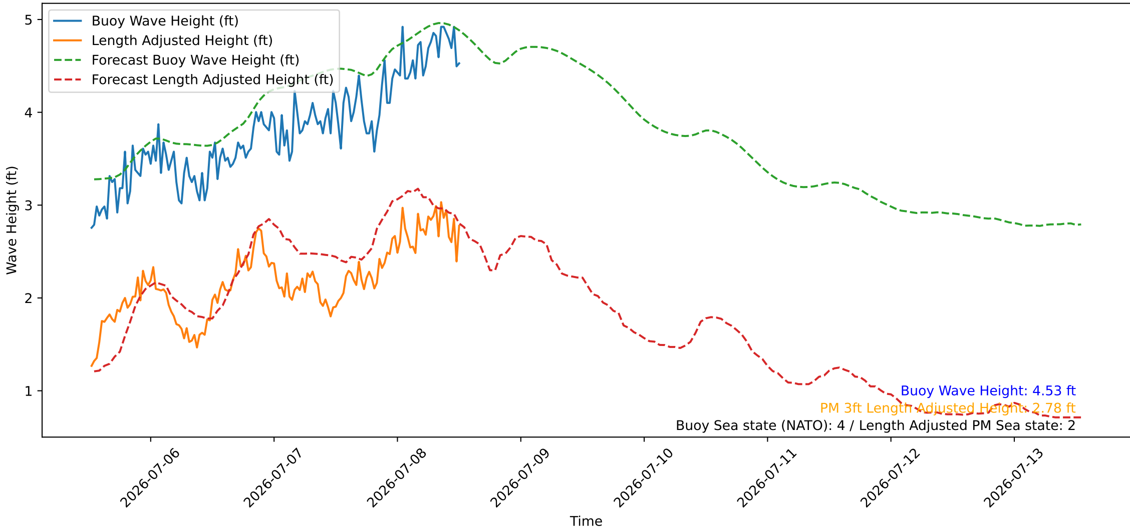
Wave Heights over Time for Oceanside Harbor at 2026-07-08 12:40:26
