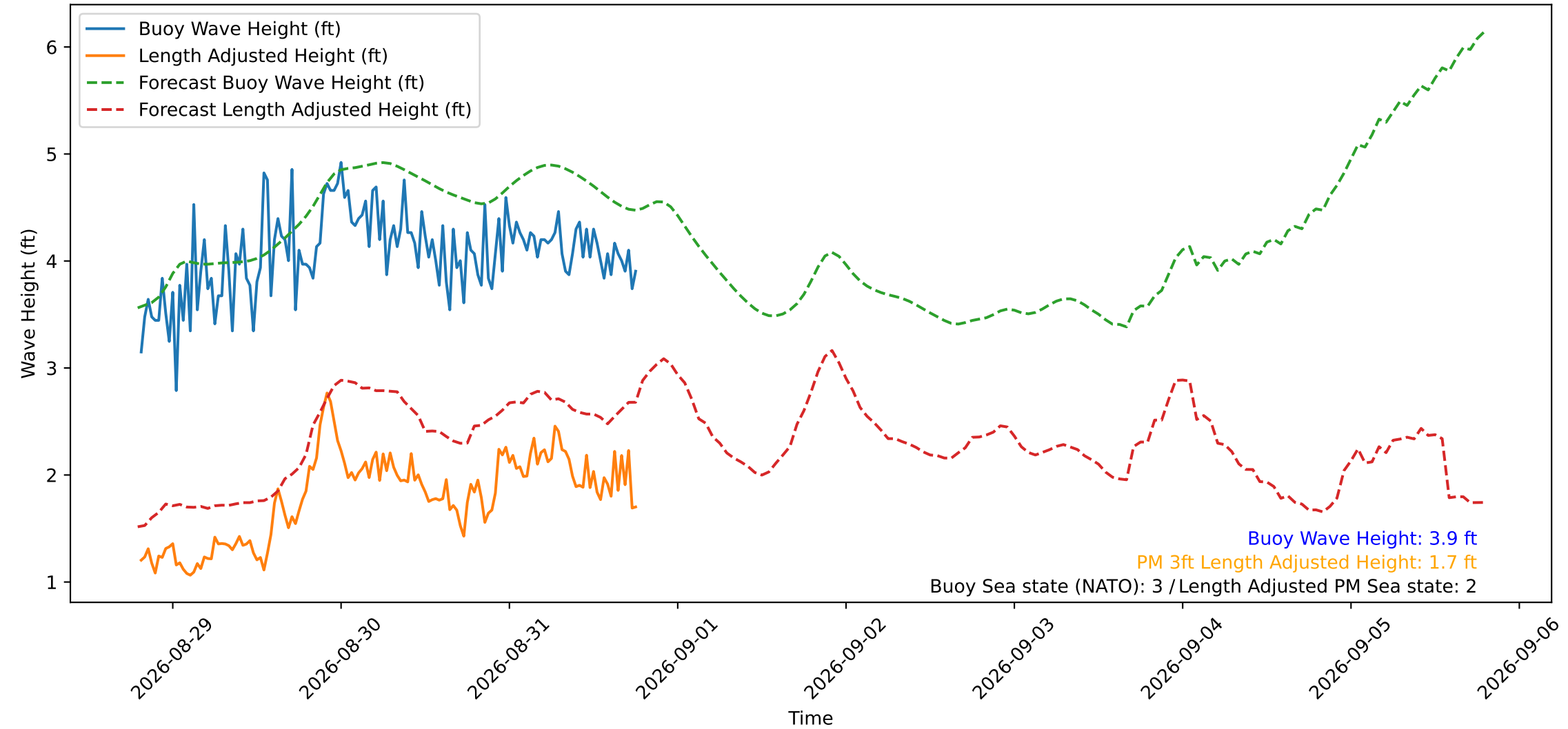
Wave Heights over Time for Green Beach at 2026-08-31 19:01:12
