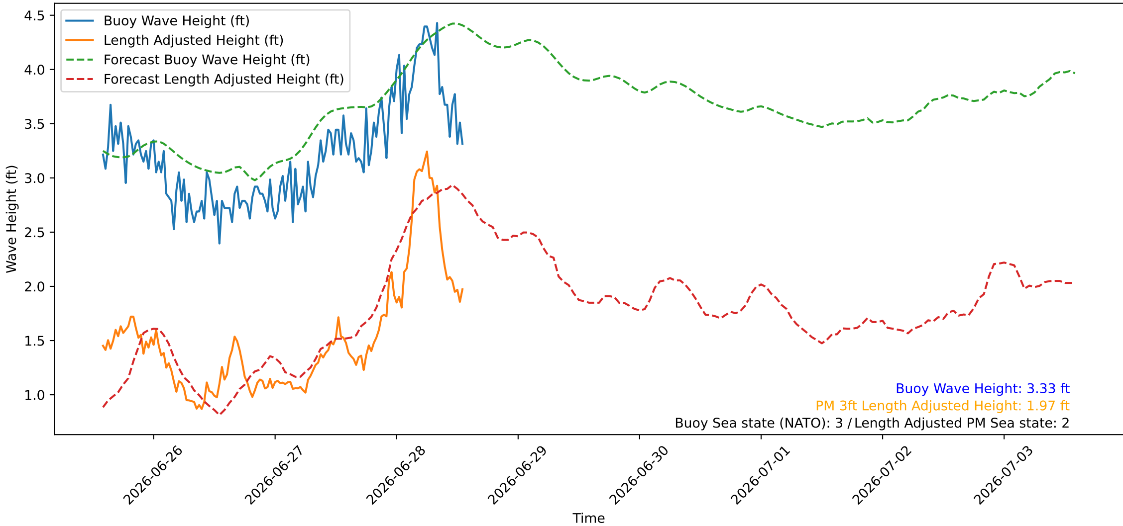
Wave Heights over Time for Oceanside Harbor at 2026-06-28 13:50:26
