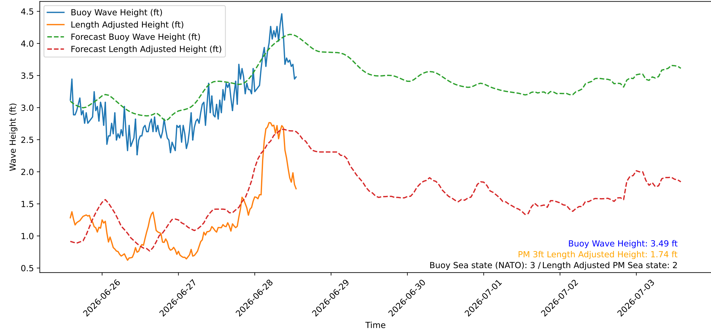
Wave Heights over Time for Red Beach at 2026-06-28 13:50:47
