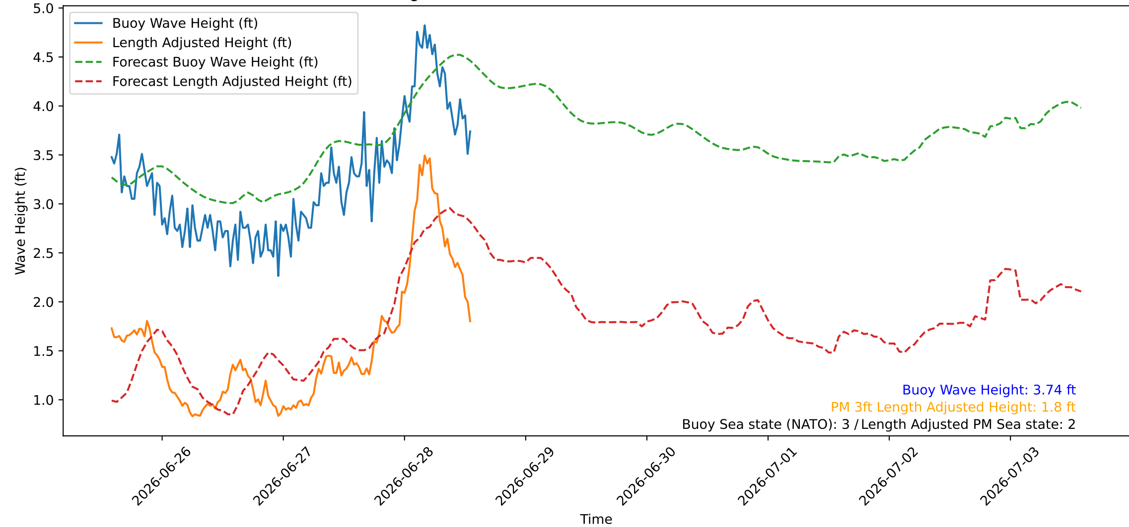
Wave Heights over Time for Green Beach at 2026-06-28 13:51:09
