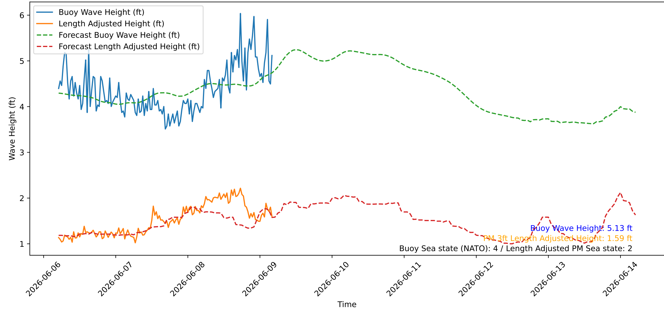
Wave Heights over Time for Oceanside Harbor at 2026-06-09 05:00:26
