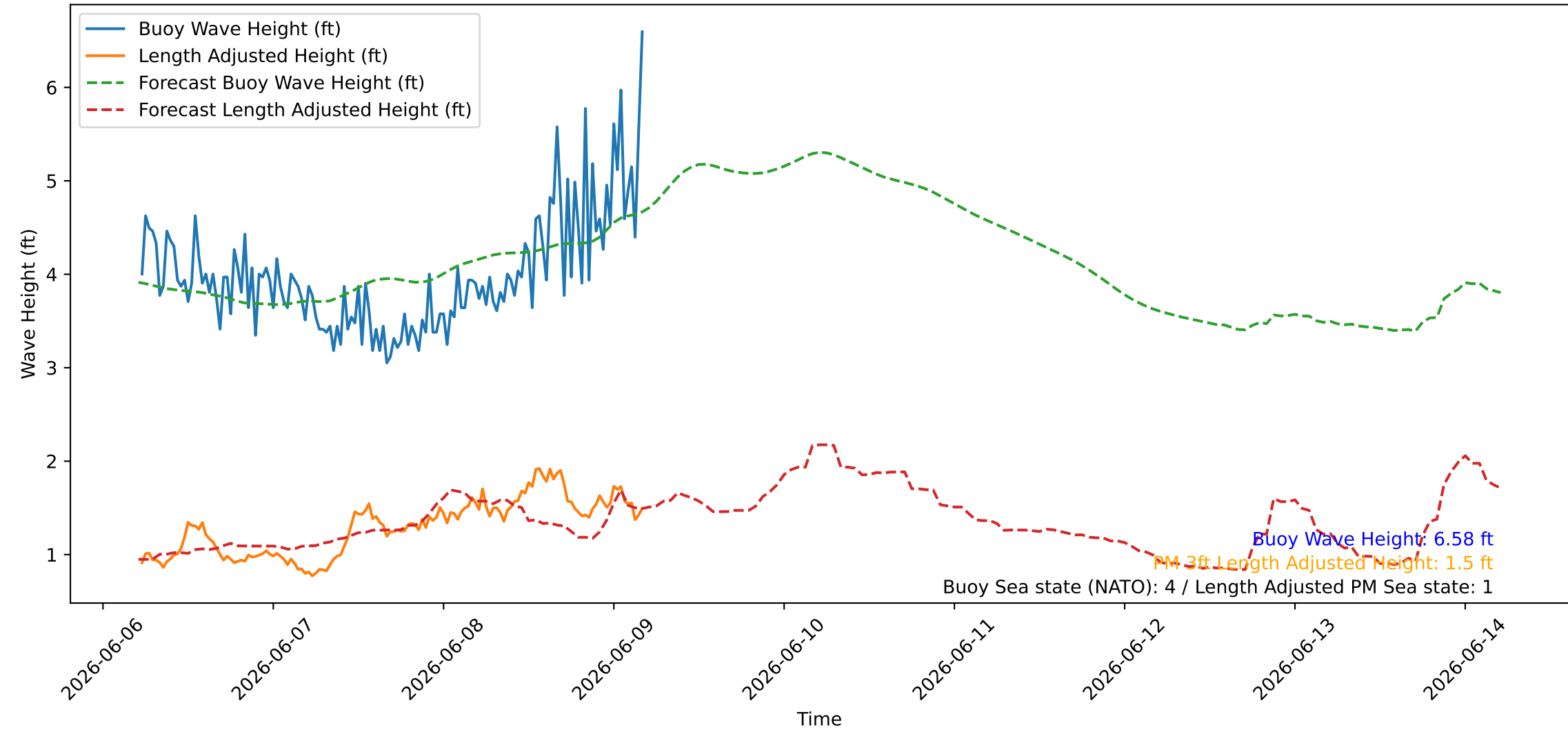
Wave Heights over Time for Red Beach at 2026-06-09 05:00:45
