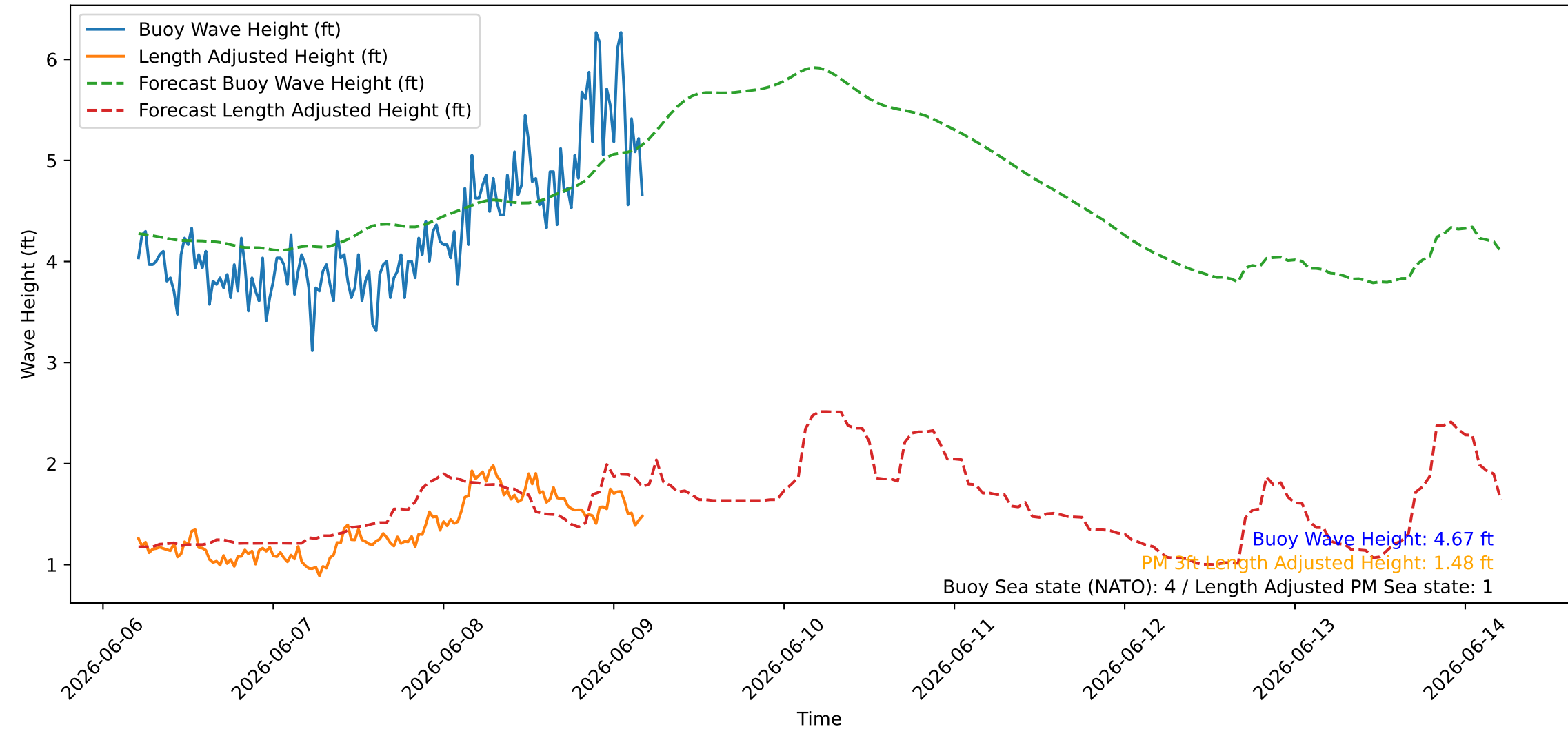
Wave Heights over Time for Green Beach at 2026-06-09 05:01:08
