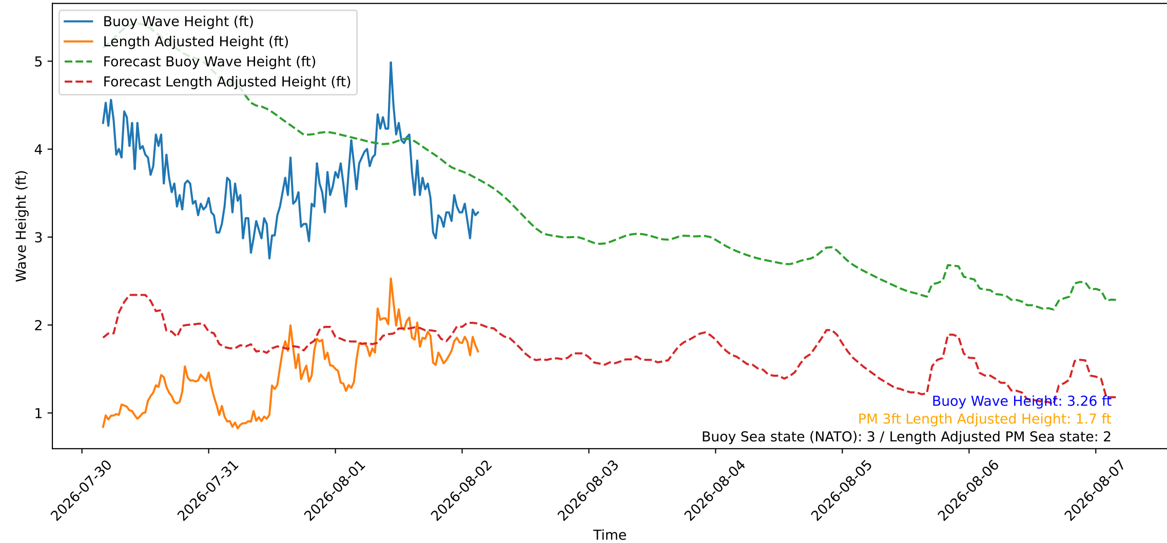
Wave Heights over Time for Green Beach at 2026-08-02 04:01:08
