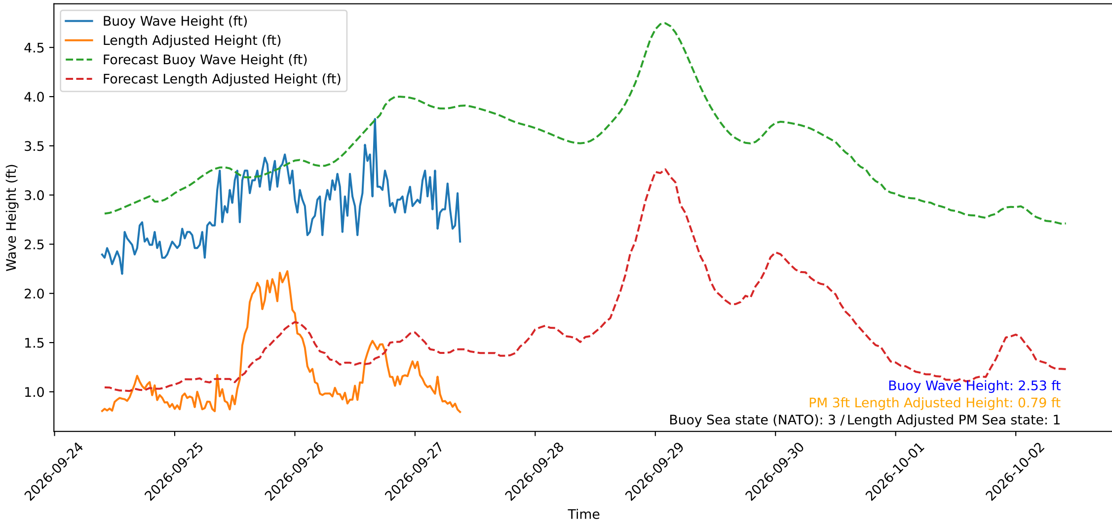
Wave Heights over Time for Oceanside Harbor at 2026-09-27 09:30:30
