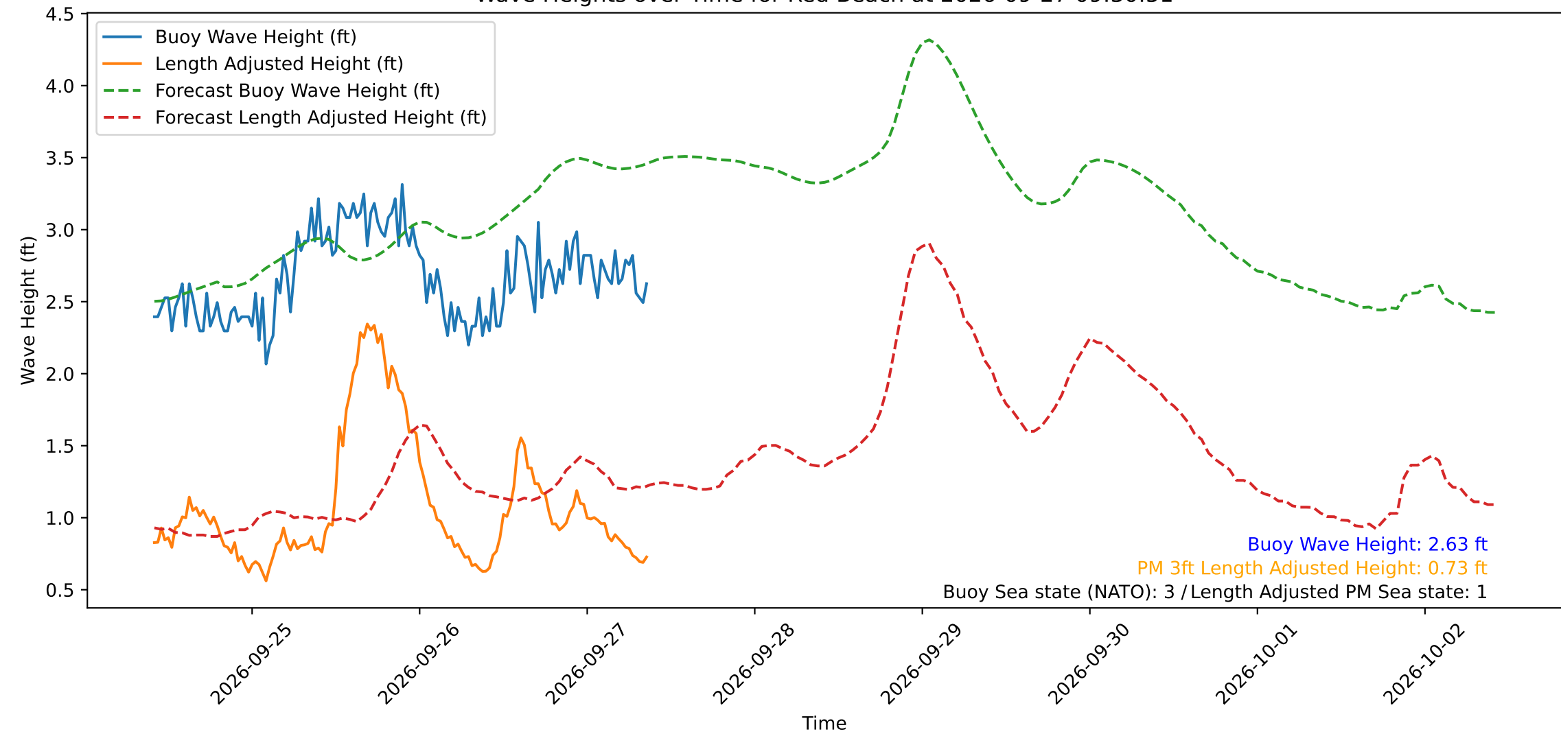
Wave Heights over Time for Red Beach at 2026-09-27 09:30:51
