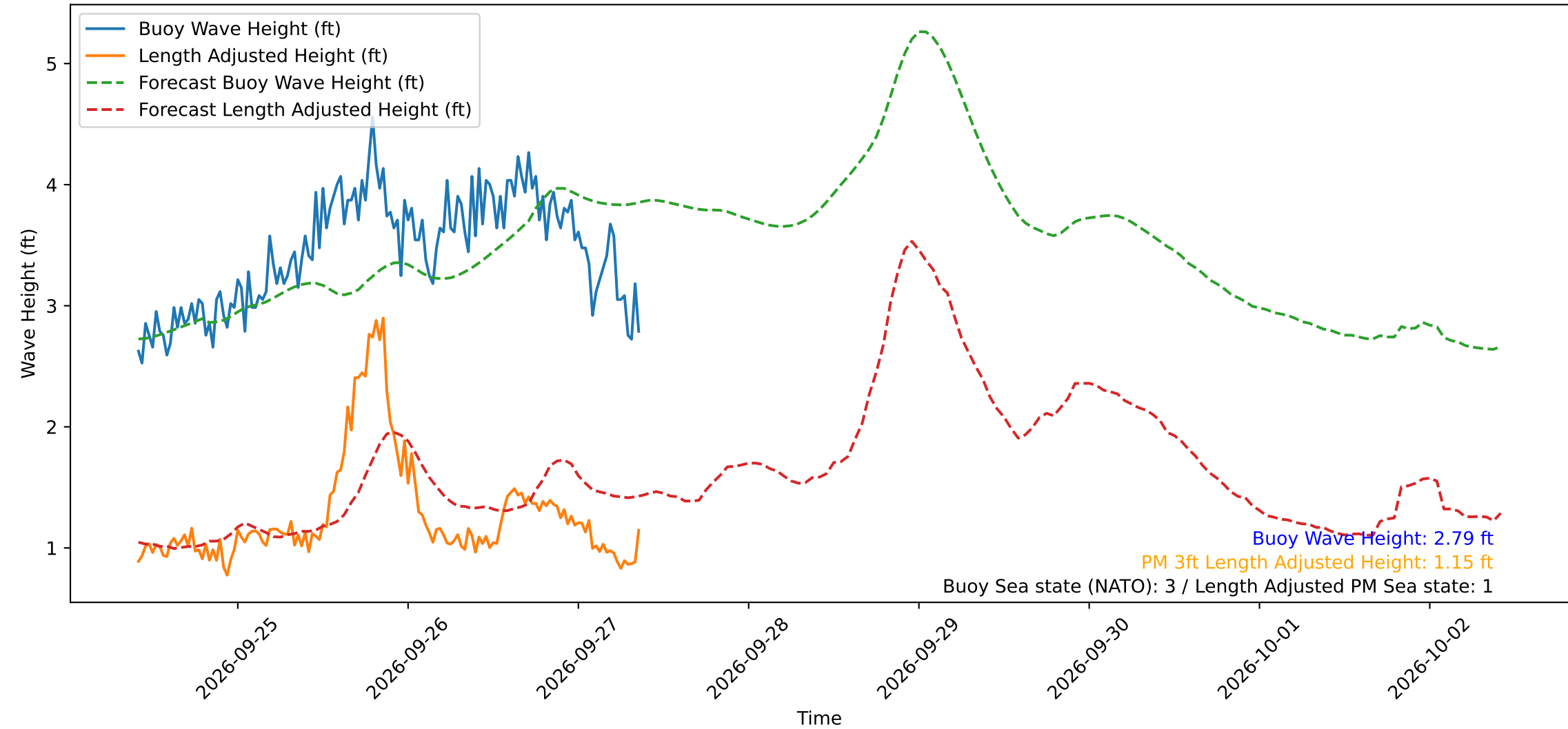
Wave Heights over Time for Green Beach at 2026-09-27 09:31:14
