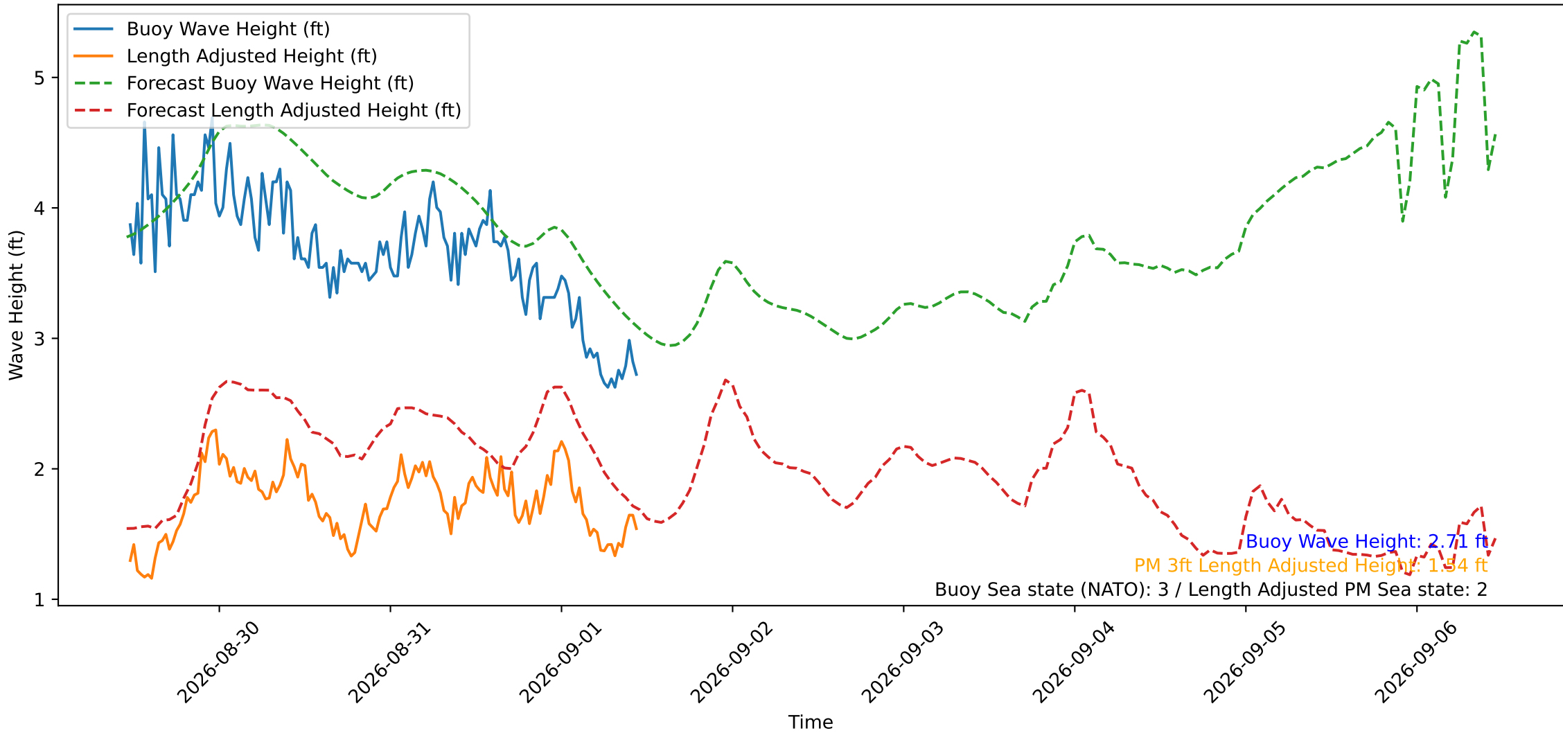
Wave Heights over Time for Red Beach at 2026-09-01 11:10:49
