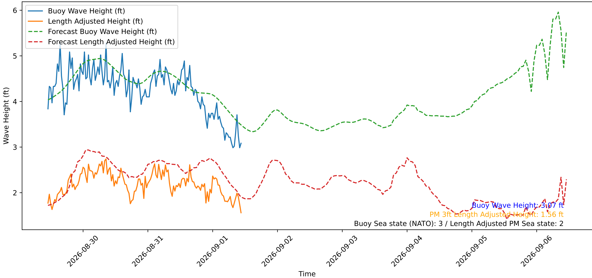
Wave Heights over Time for Oceanside Harbor at 2026-09-01 11:10:29
