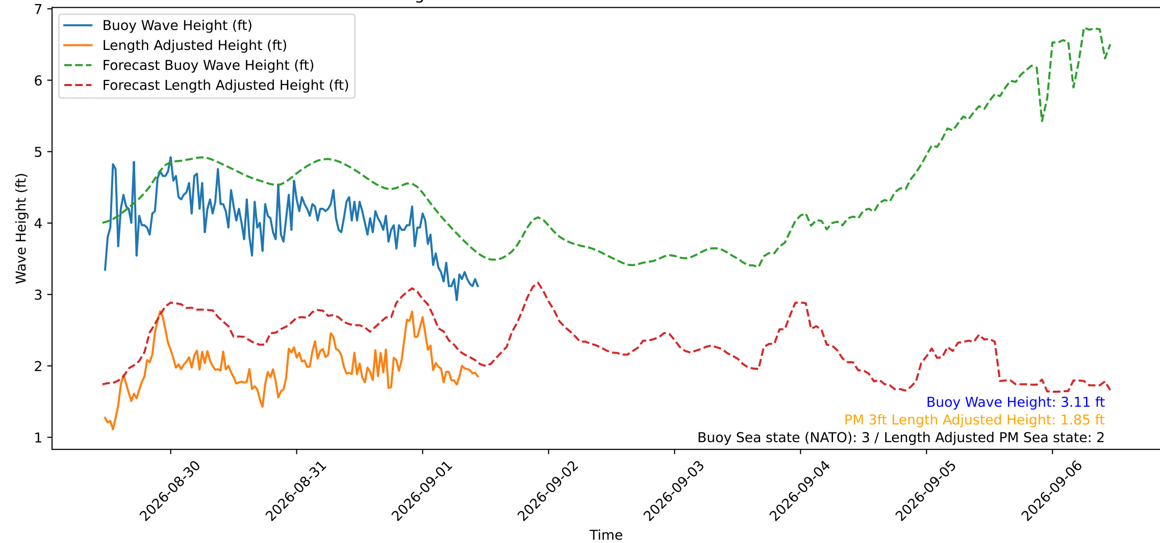
Wave Heights over Time for Green Beach at 2026-09-01 11:11:12
