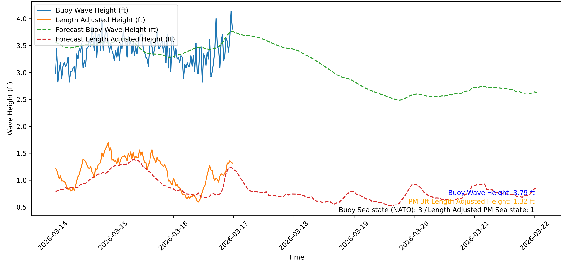
Wave Heights over Time for Green Beach at 2026-03-17 01:01:43
