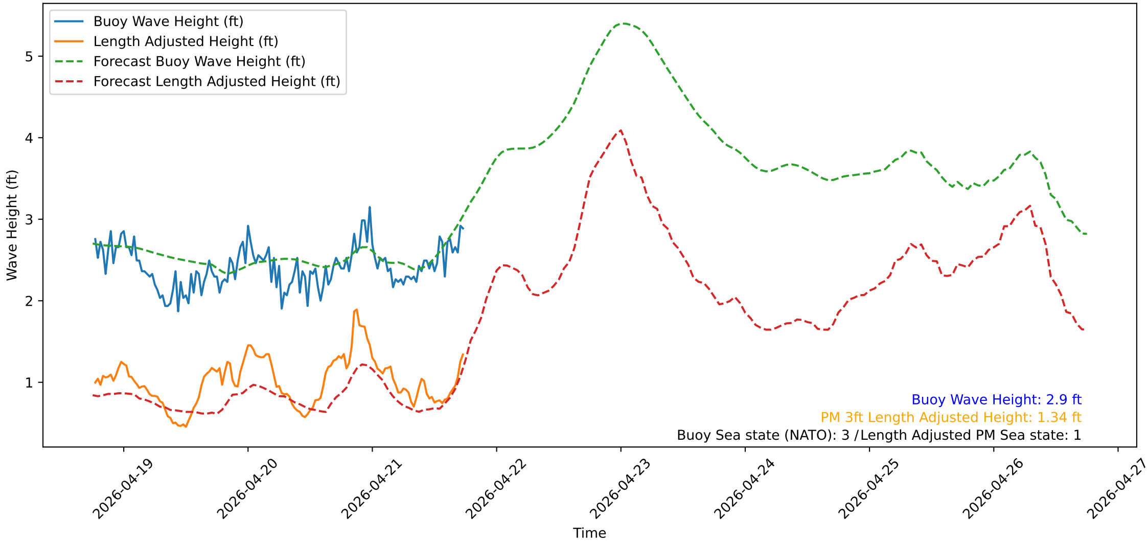
Wave Heights over Time for Green Beach at 2026-04-21 18:21:14
