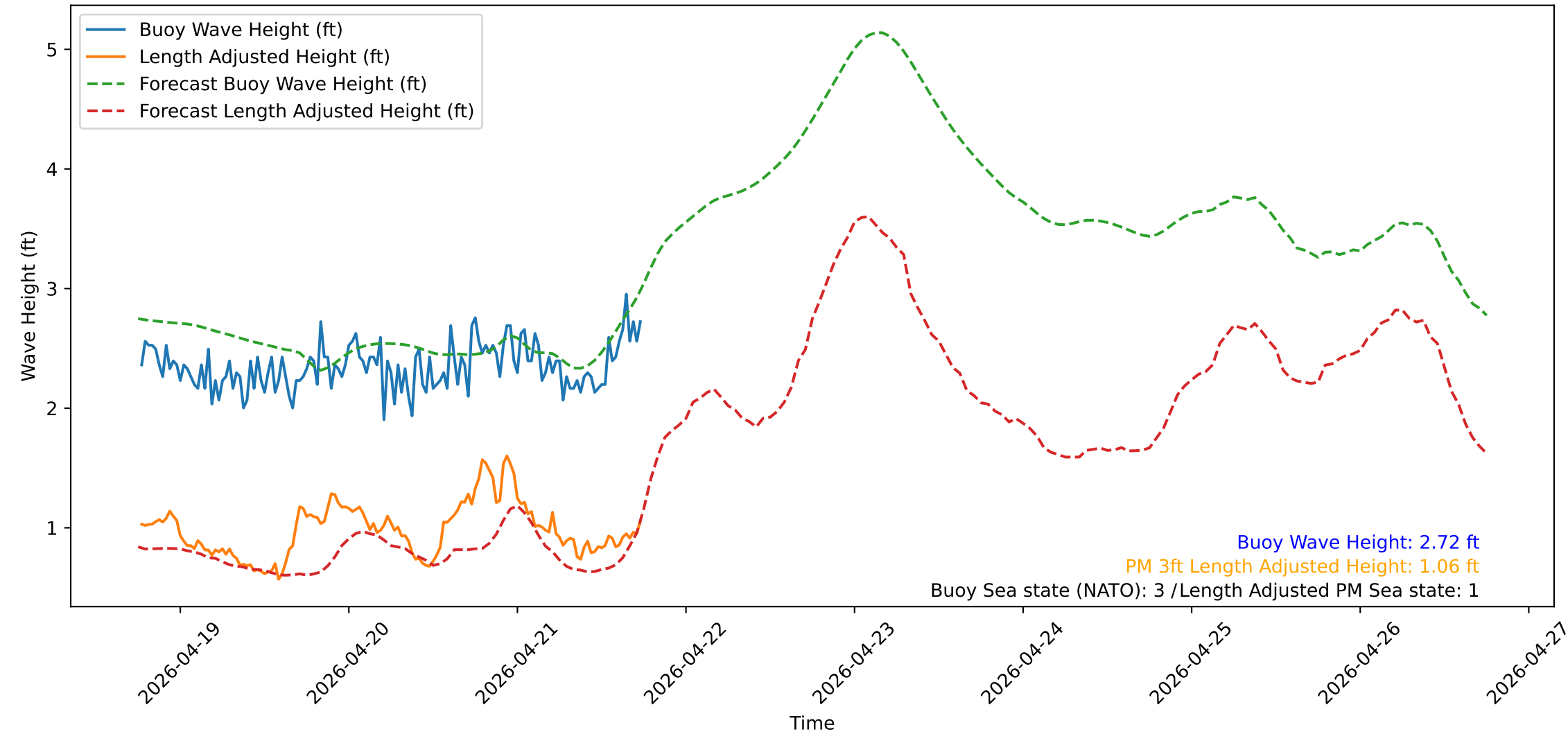
Wave Heights over Time for Oceanside Harbor at 2026-04-21 18:20:31
