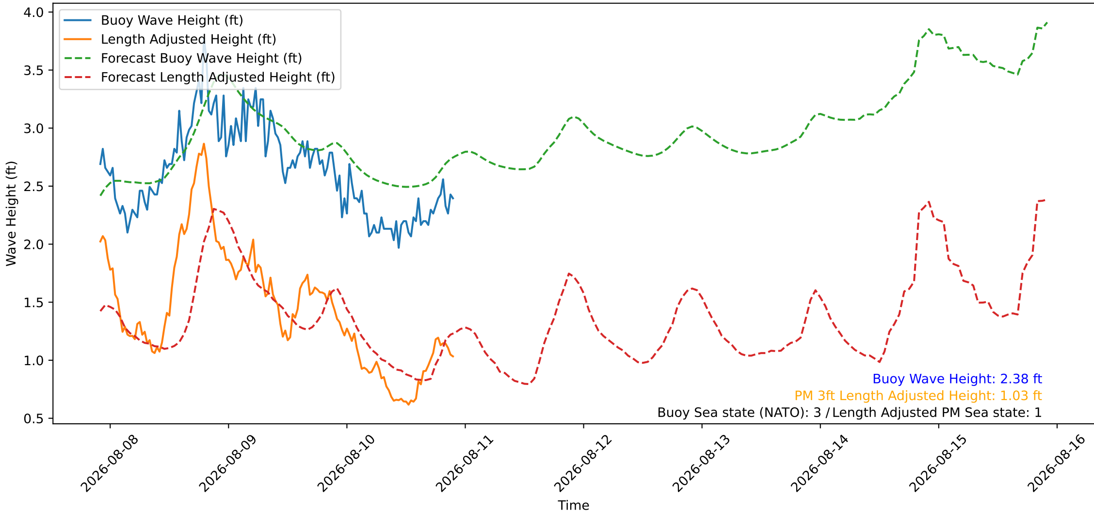
Wave Heights over Time for Green Beach at 2026-08-10 22:11:10
