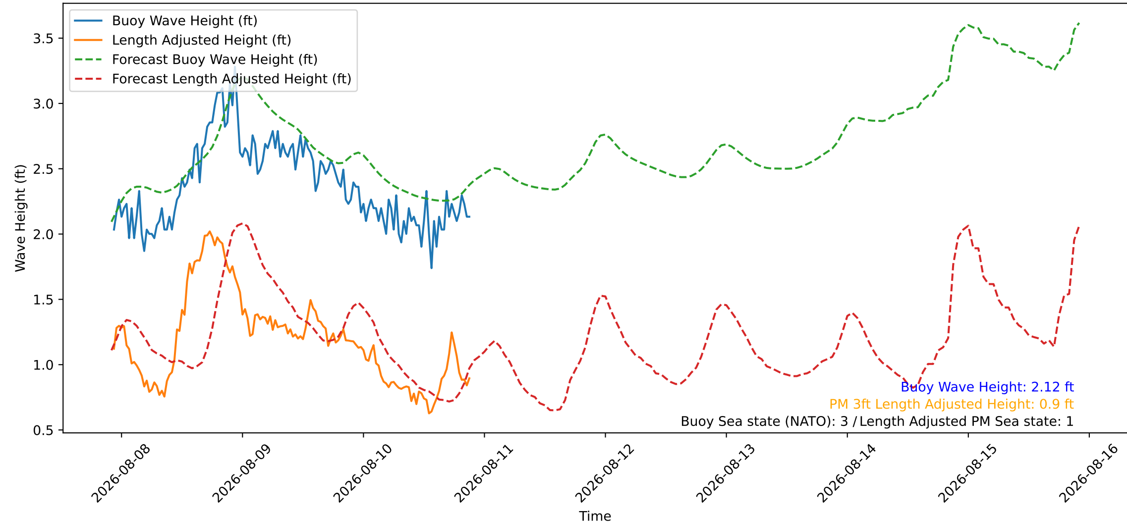
Wave Heights over Time for Red Beach at 2026-08-10 22:10:47
