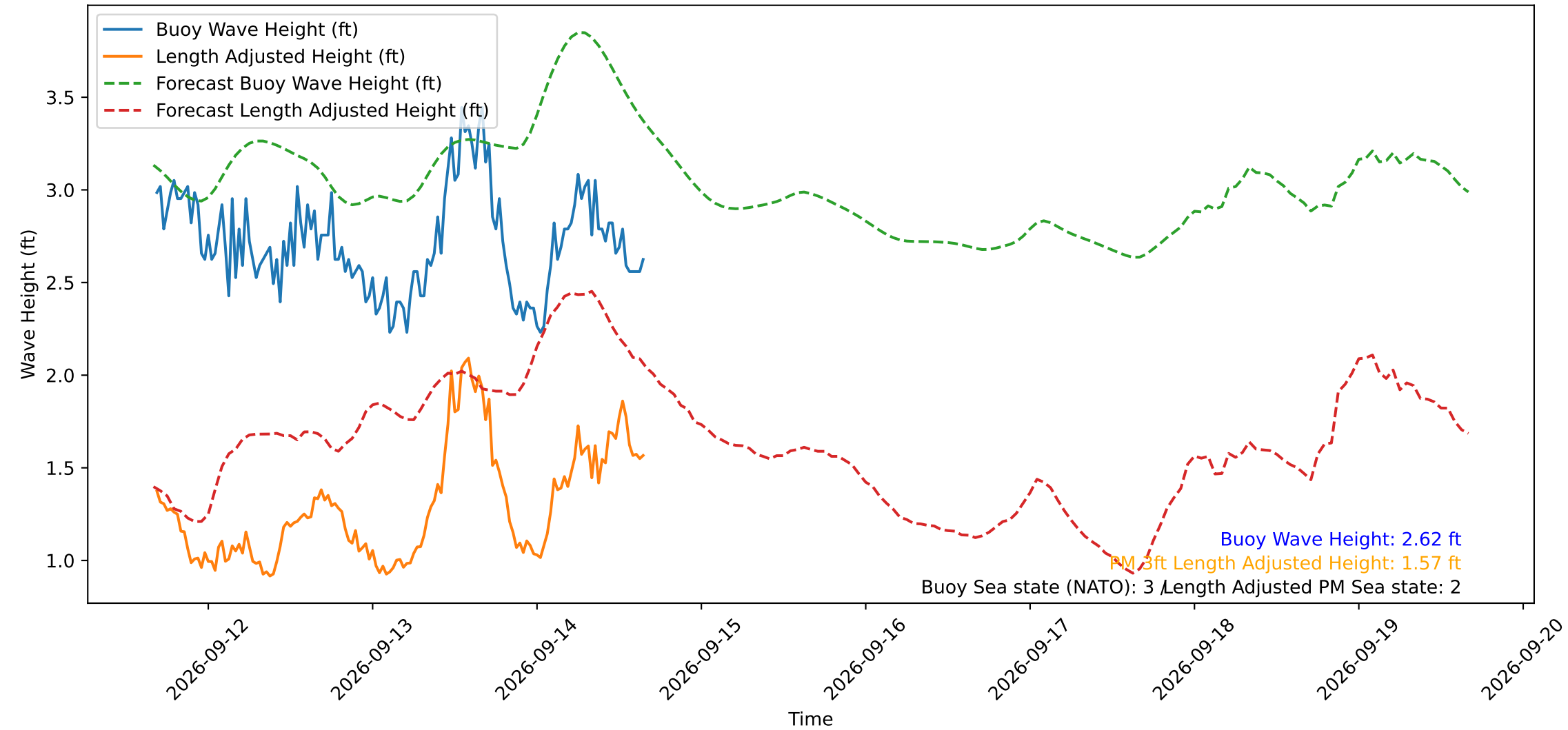
Wave Heights over Time for Red Beach at 2026-09-14 16:20:51
