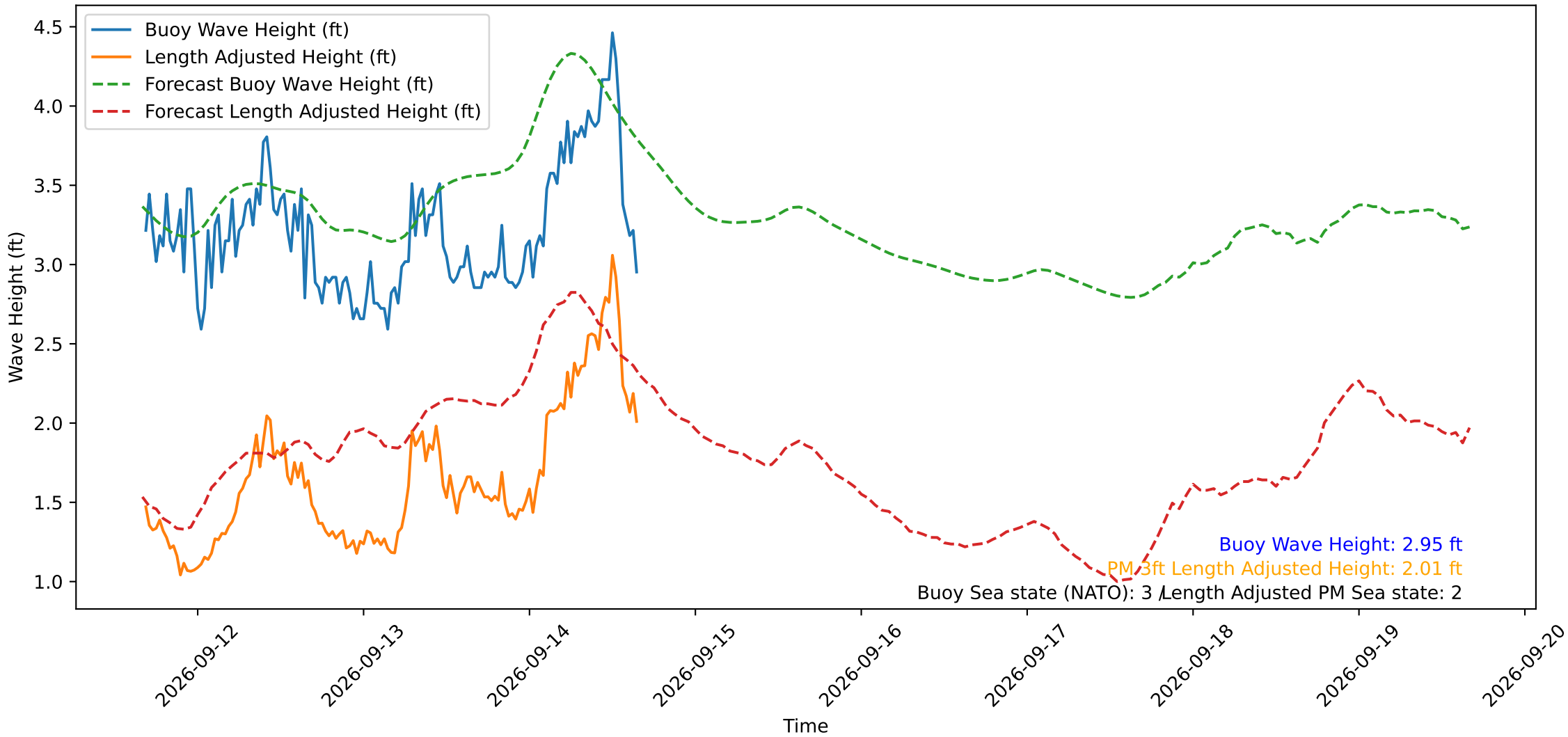
Wave Heights over Time for Oceanside Harbor at 2026-09-14 16:20:30
