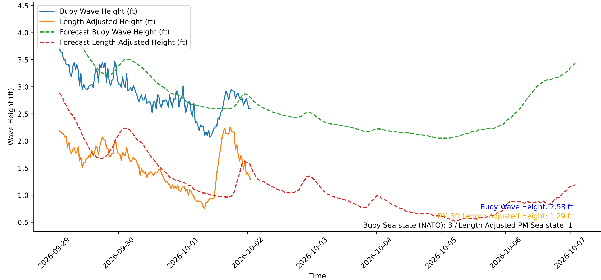
Wave Heights over Time for Red Beach at 2026-10-02 01:40:49
