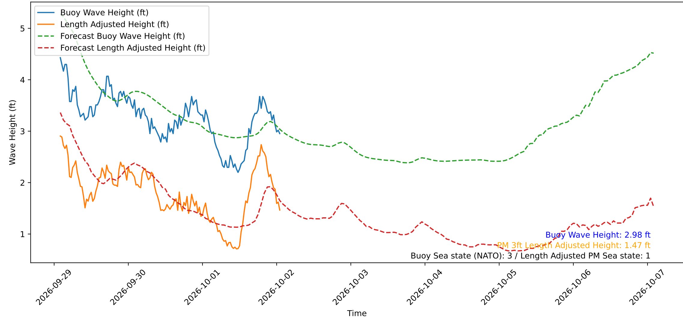
Wave Heights over Time for Green Beach at 2026-10-02 01:41:12
