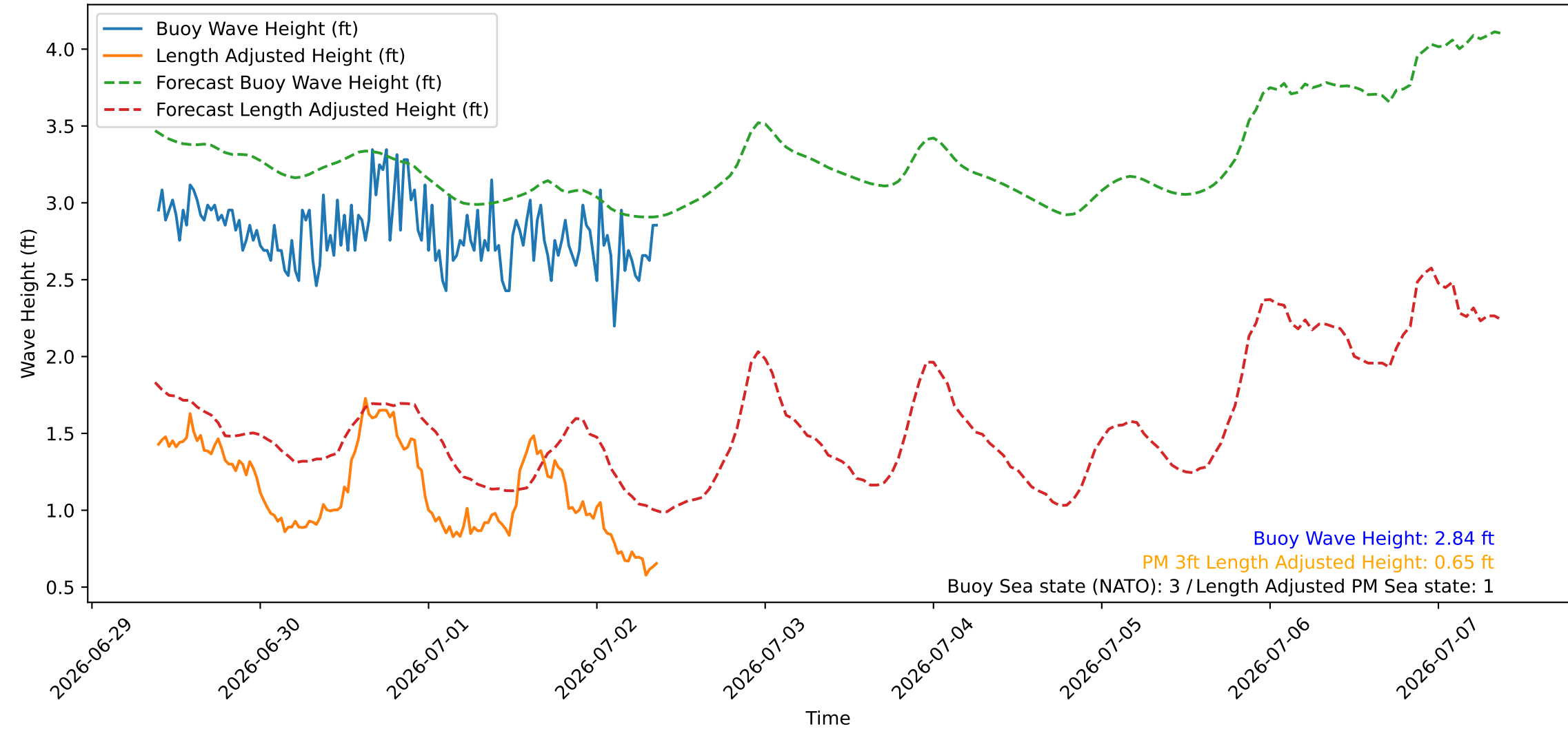
Wave Heights over Time for Red Beach at 2026-07-02 09:10:46
