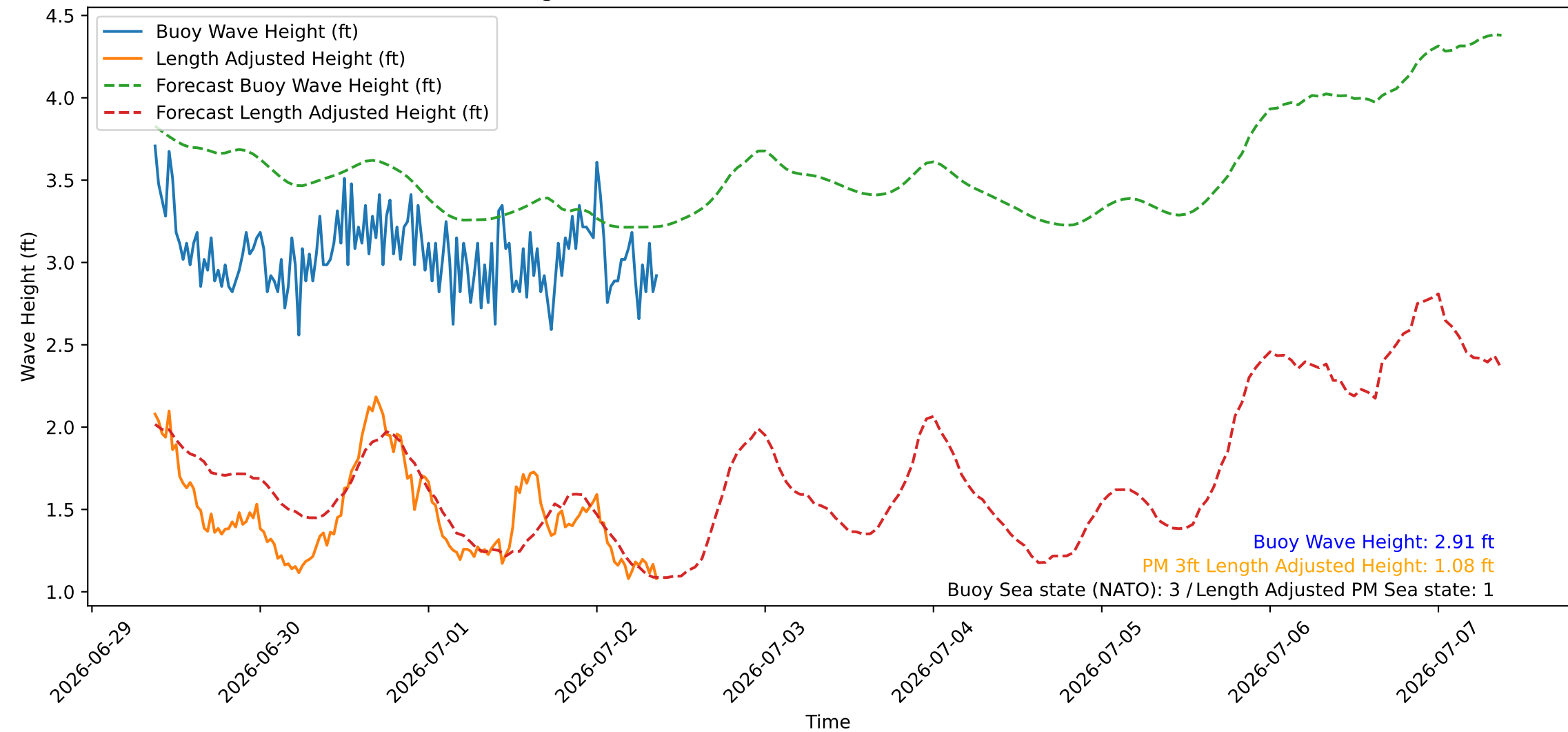
Wave Heights over Time for Oceanside Harbor at 2026-07-02 09:10:26
