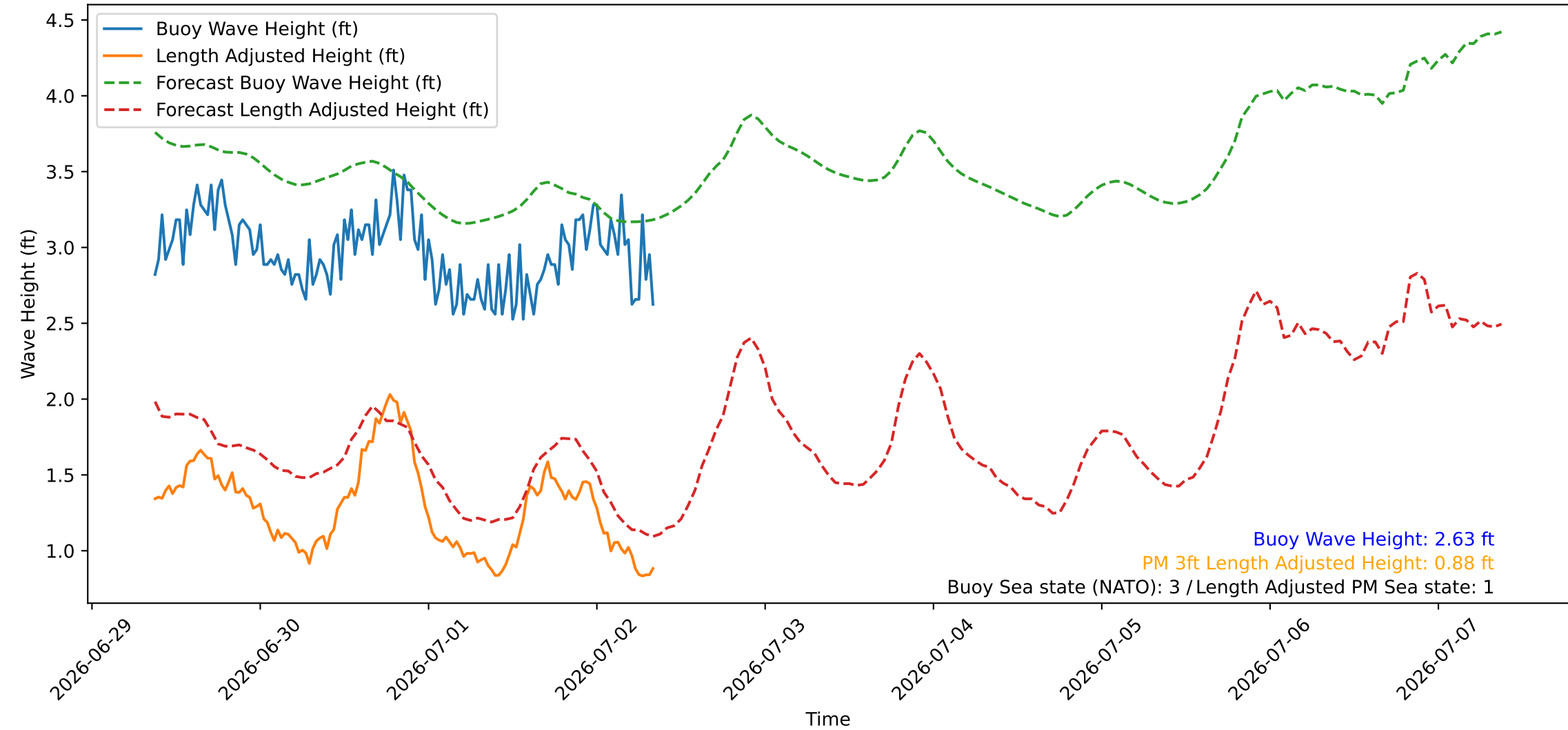
Wave Heights over Time for Green Beach at 2026-07-02 09:11:08
