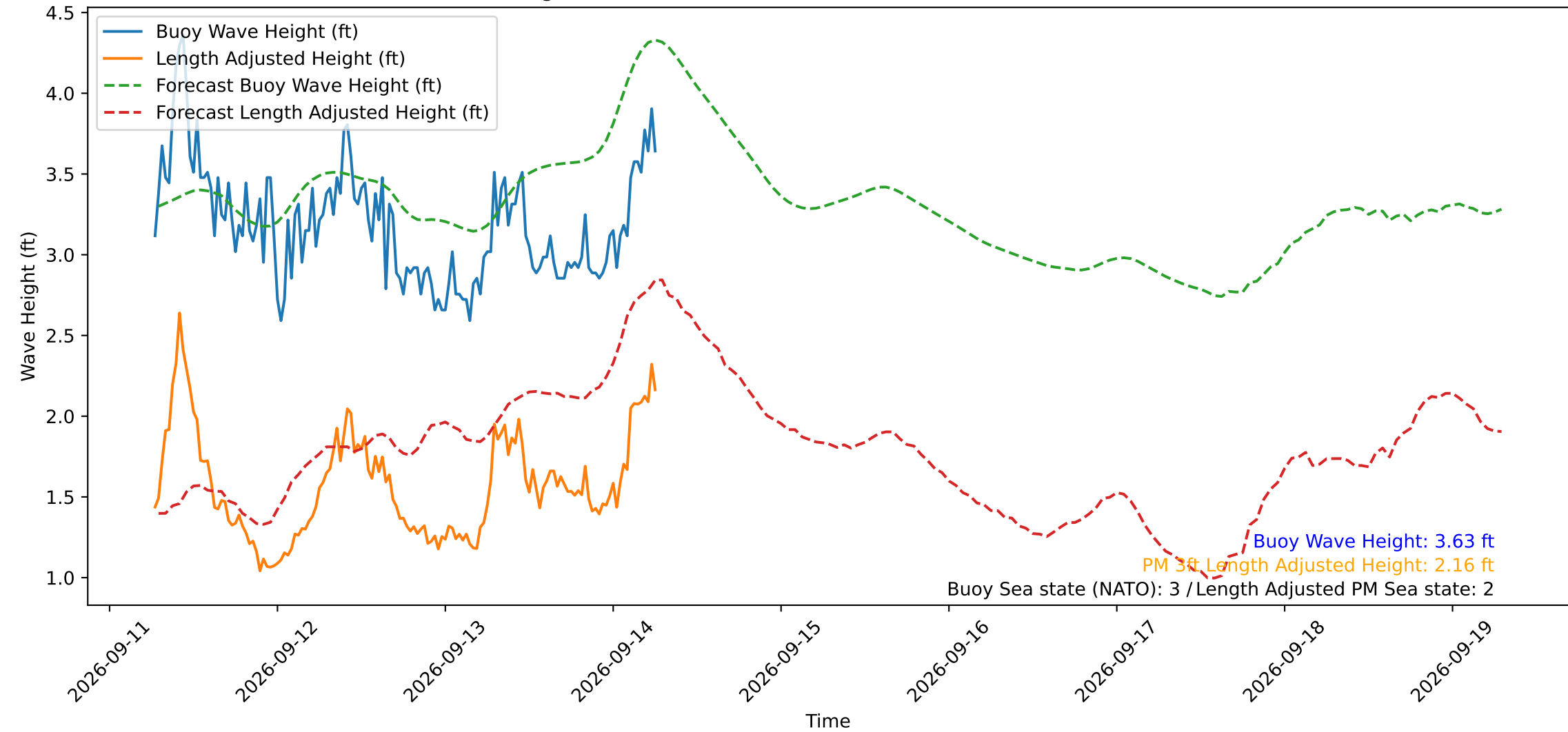
Wave Heights over Time for Oceanside Harbor at 2026-09-14 06:40:30
