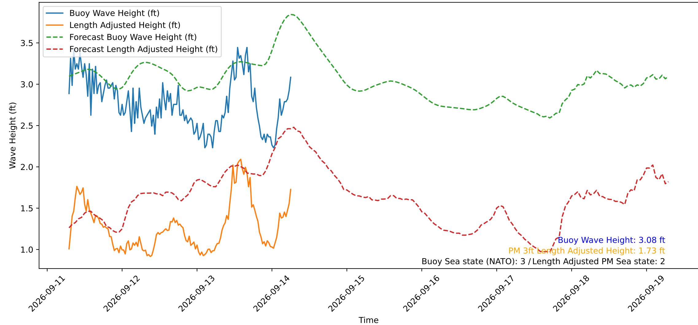
Wave Heights over Time for Red Beach at 2026-09-14 06:40:49
