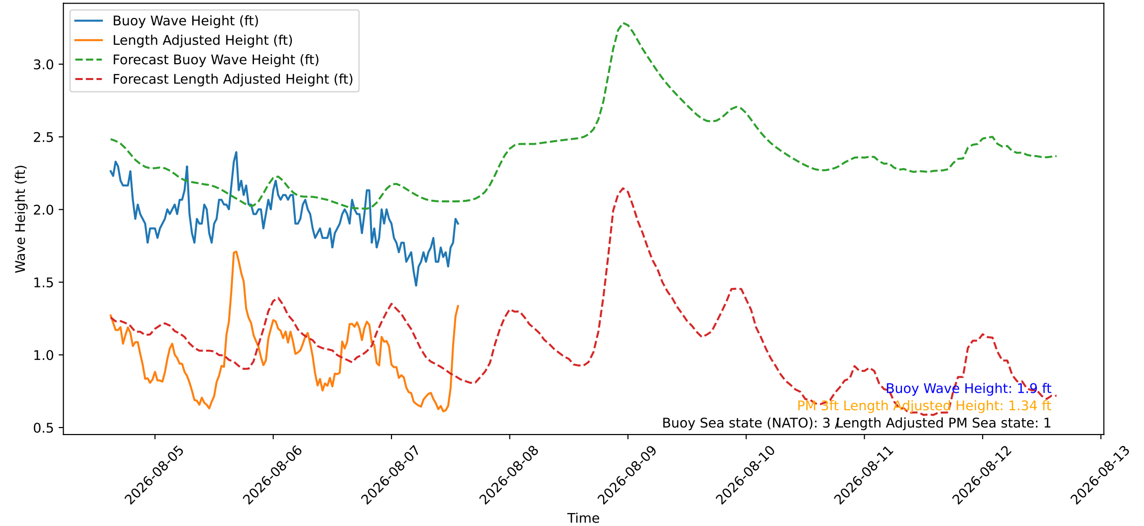
Wave Heights over Time for Red Beach at 2026-08-07 14:30:46
