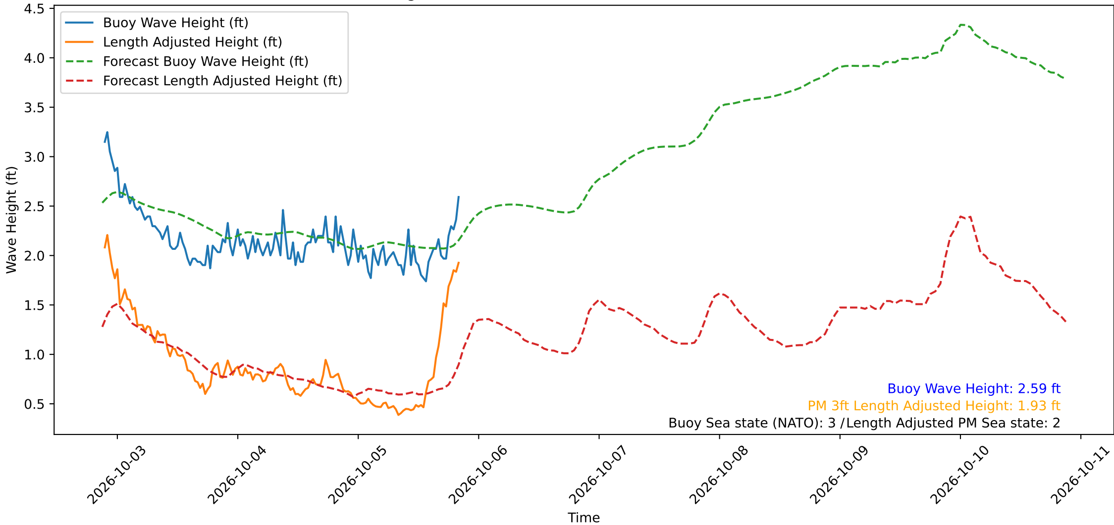
Wave Heights over Time for Red Beach at 2026-10-05 21:00:50
