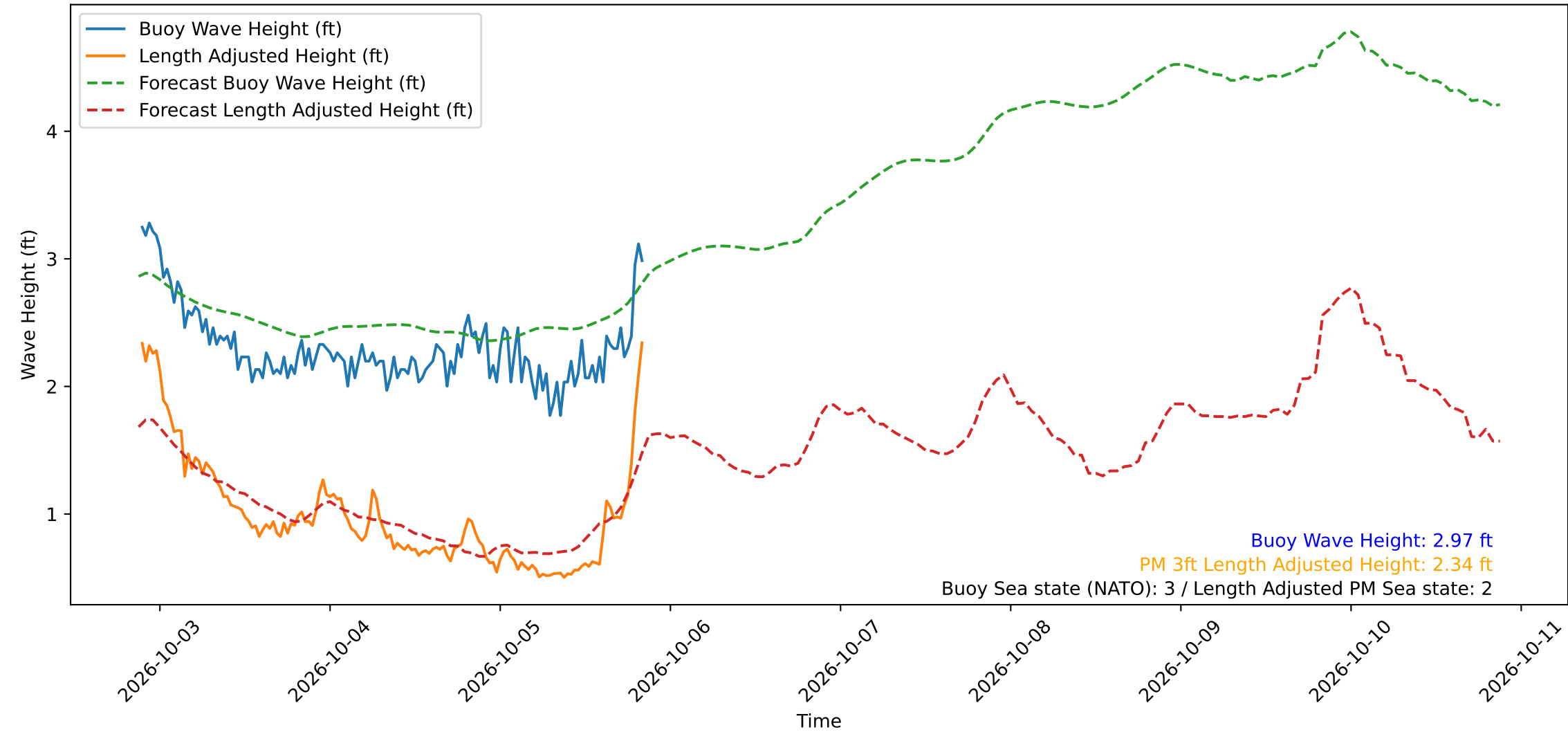
Wave Heights over Time for Green Beach at 2026-10-05 21:01:13
