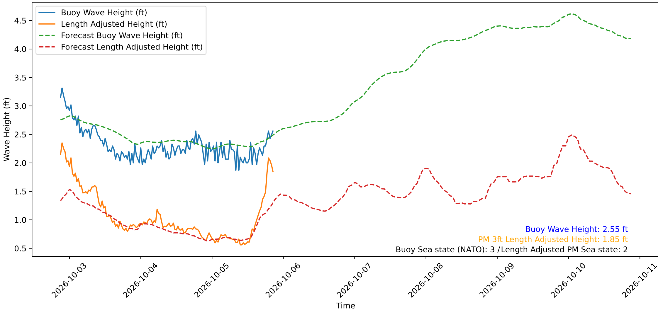
Wave Heights over Time for Oceanside Harbor at 2026-10-05 21:00:30
