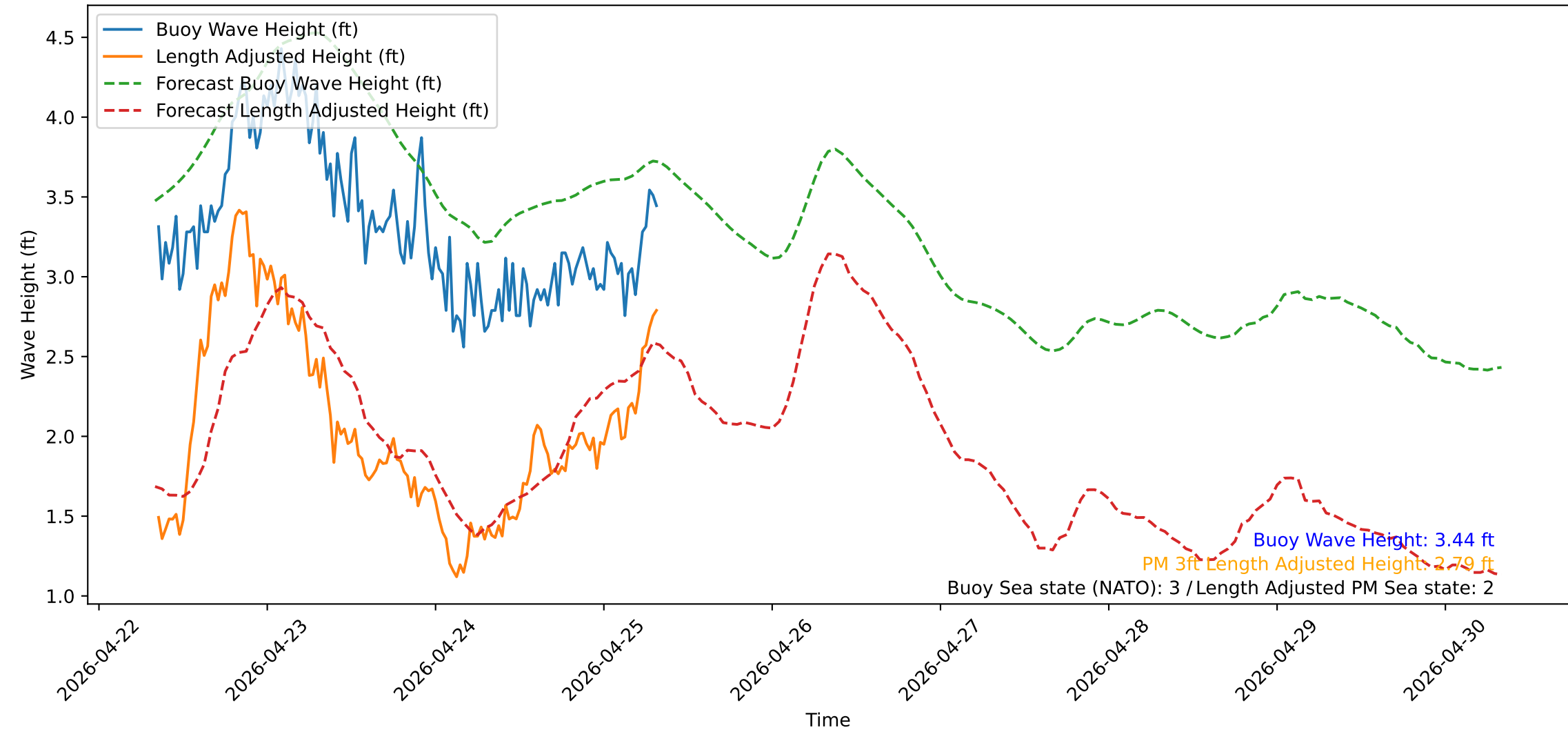
Wave Heights over Time for Oceanside Harbor at 2026-04-25 08:20:31
