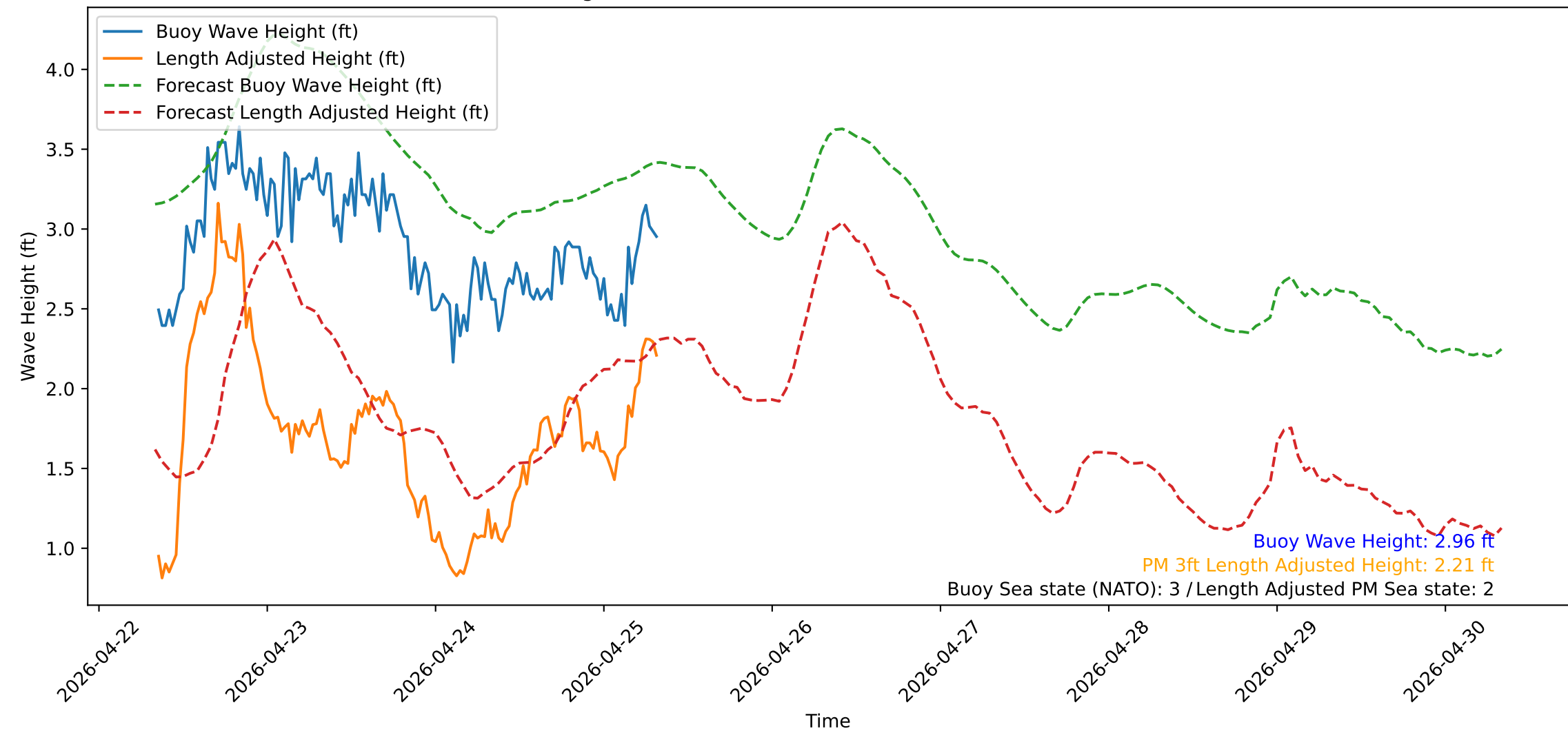
Wave Heights over Time for Red Beach at 2026-04-25 08:20:51
