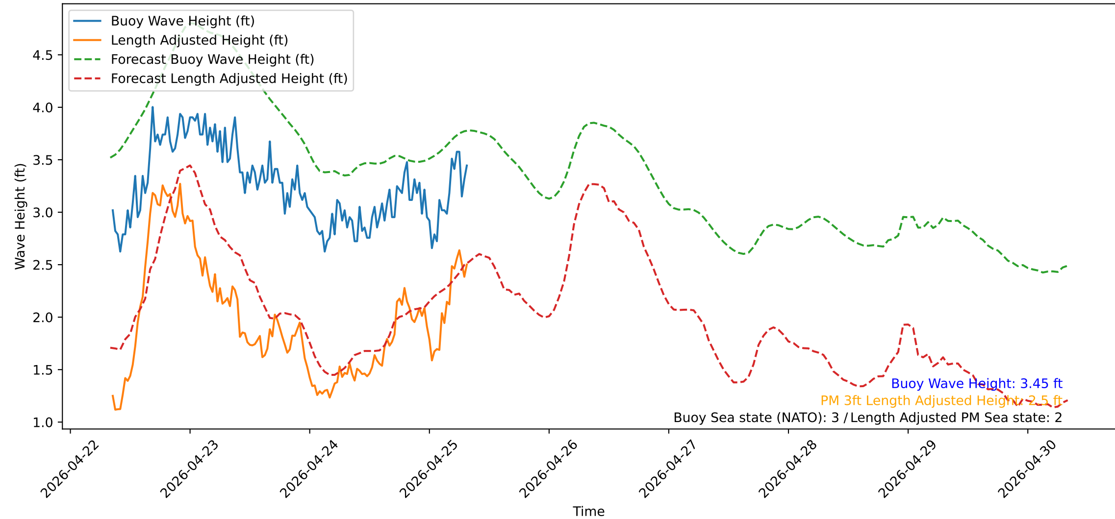
Wave Heights over Time for Green Beach at 2026-04-25 08:21:14
