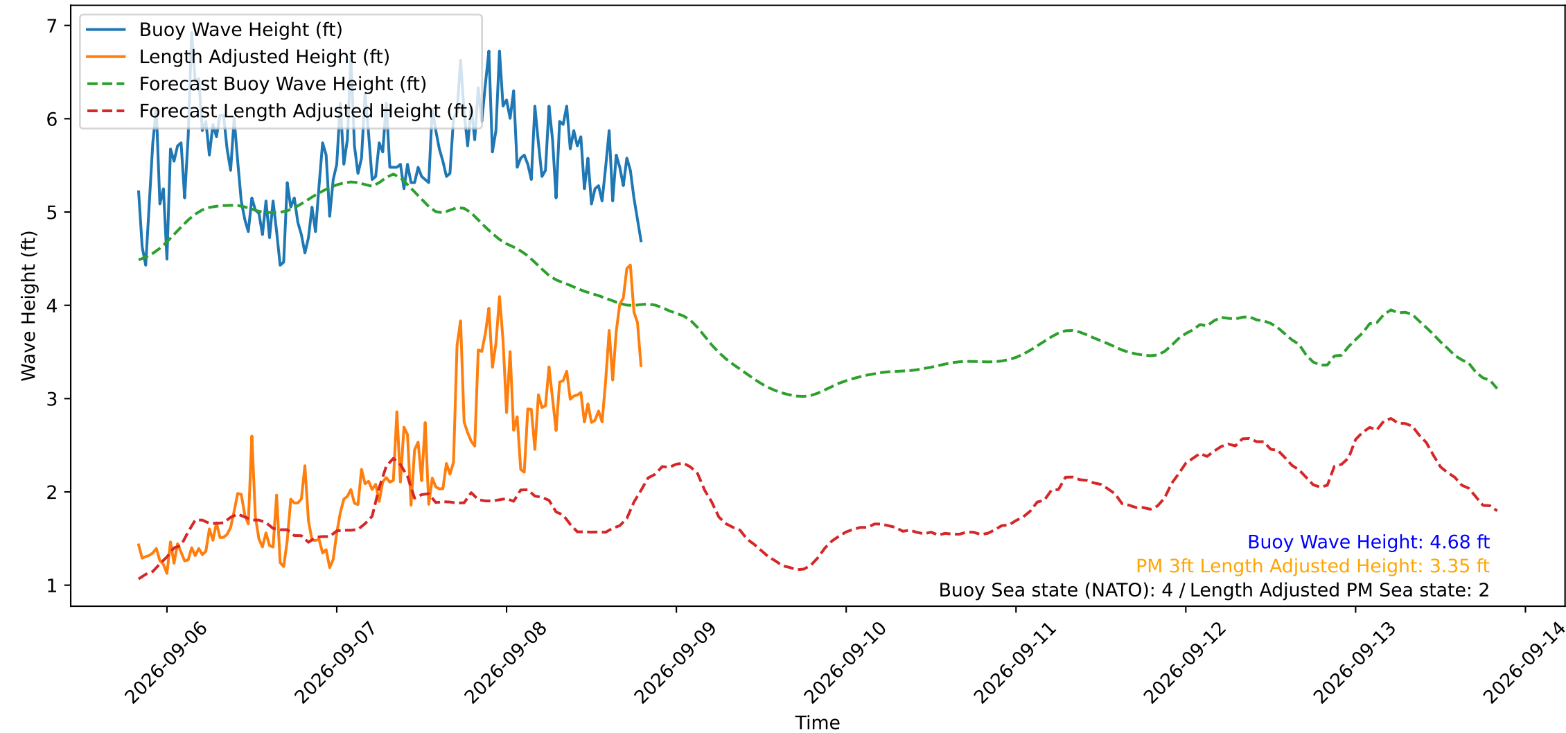
Wave Heights over Time for Red Beach at 2026-09-08 19:40:51
