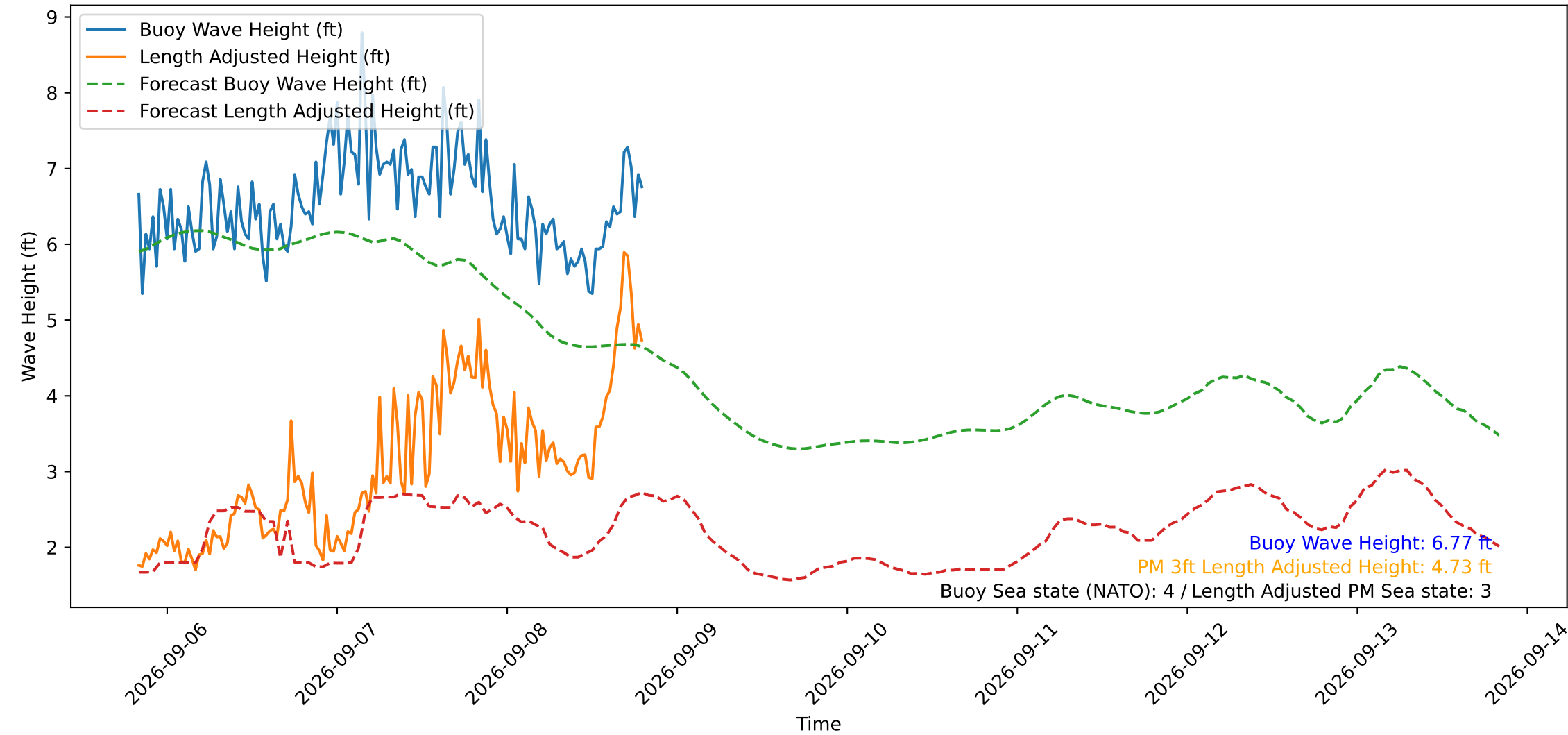
Wave Heights over Time for Green Beach at 2026-09-08 19:41:13
