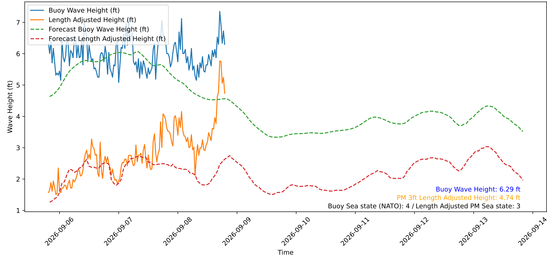
Wave Heights over Time for Oceanside Harbor at 2026-09-08 19:40:30
