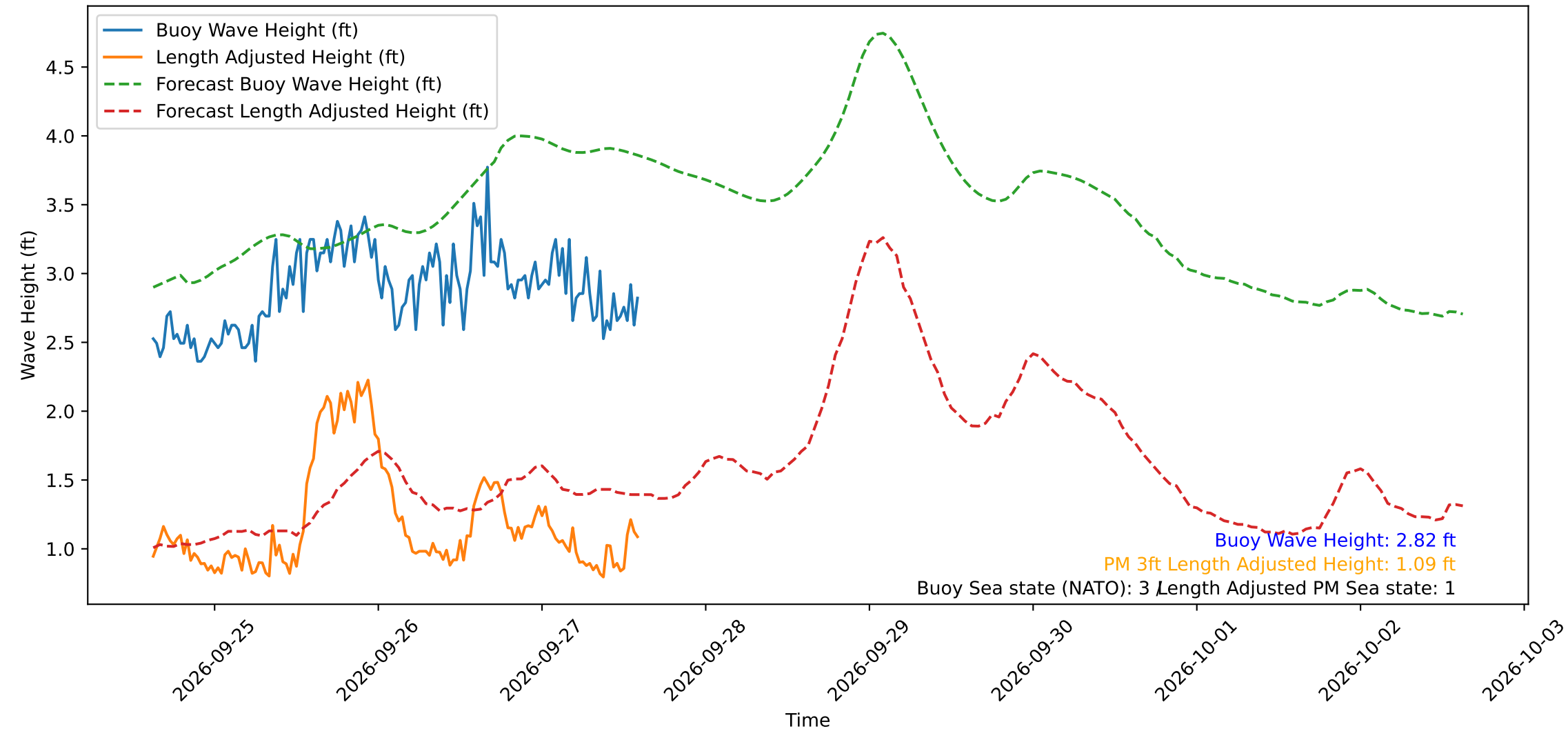
Wave Heights over Time for Oceanside Harbor at 2026-09-27 15:00:30
