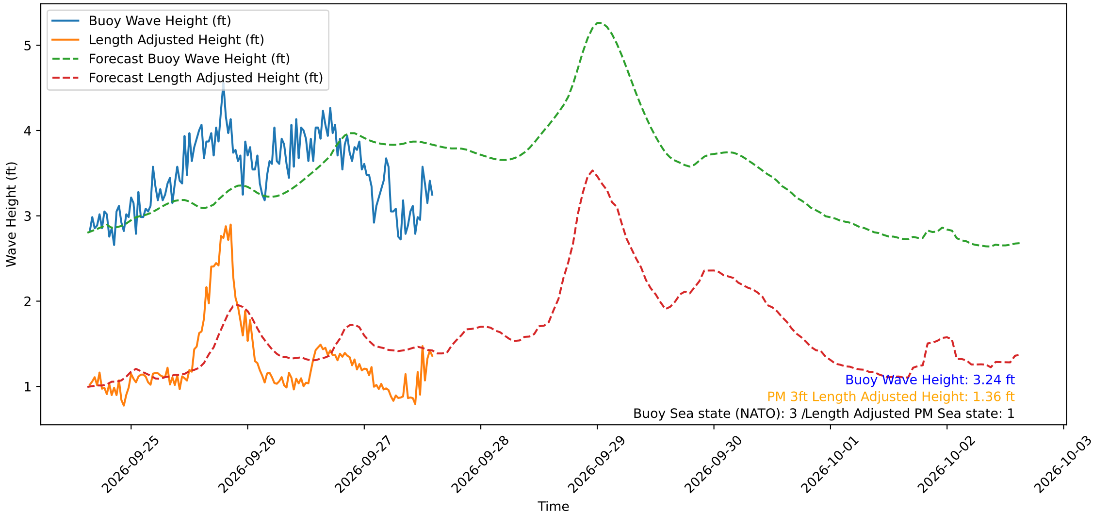
Wave Heights over Time for Green Beach at 2026-09-27 15:01:11
