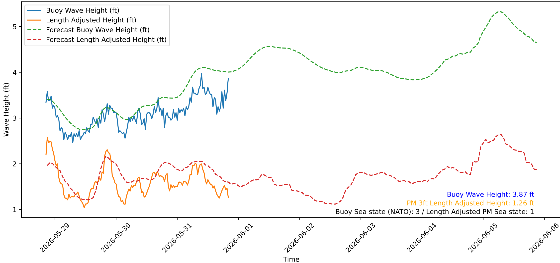
Wave Heights over Time for Green Beach at 2026-05-31 20:41:08
