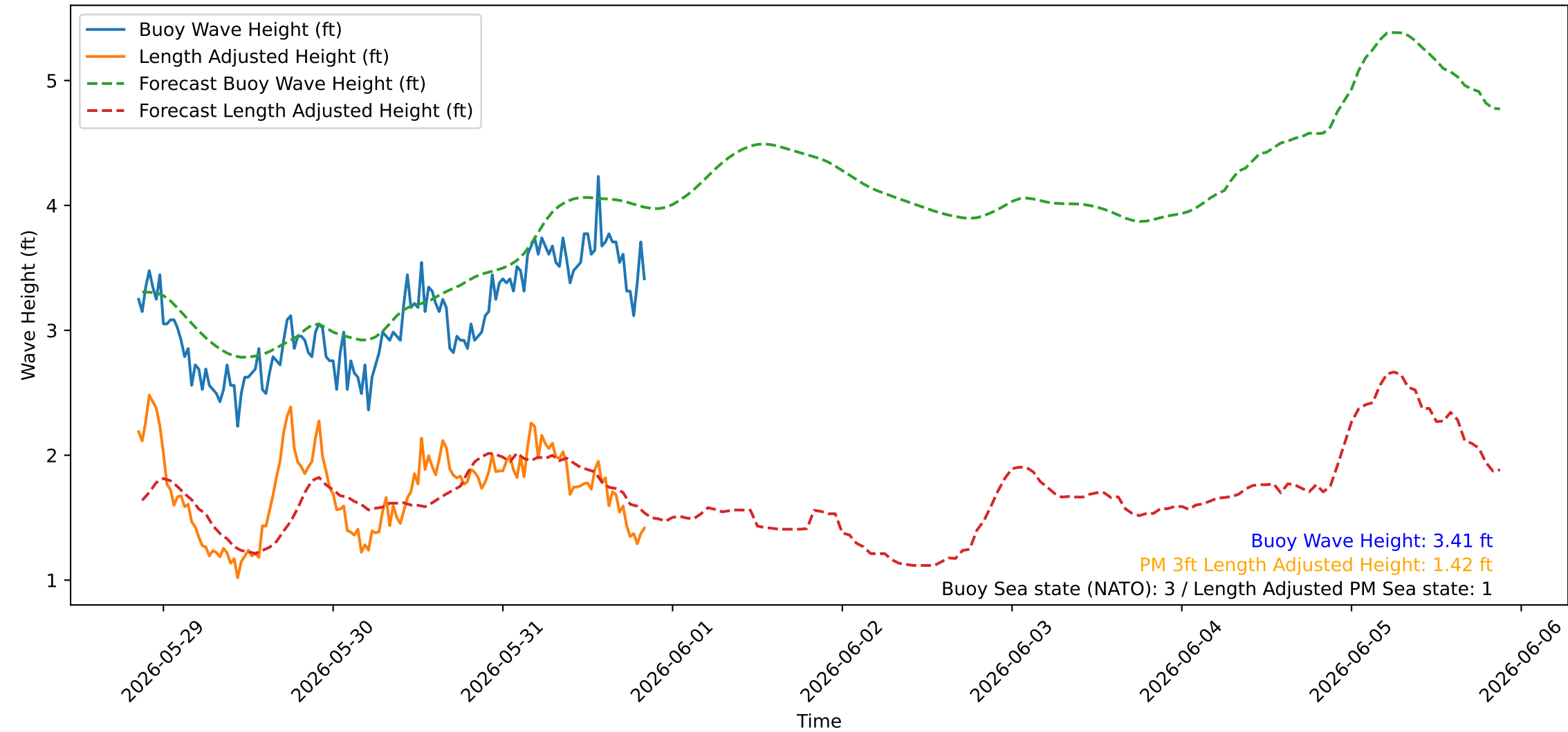
Wave Heights over Time for Oceanside Harbor at 2026-05-31 20:40:26
