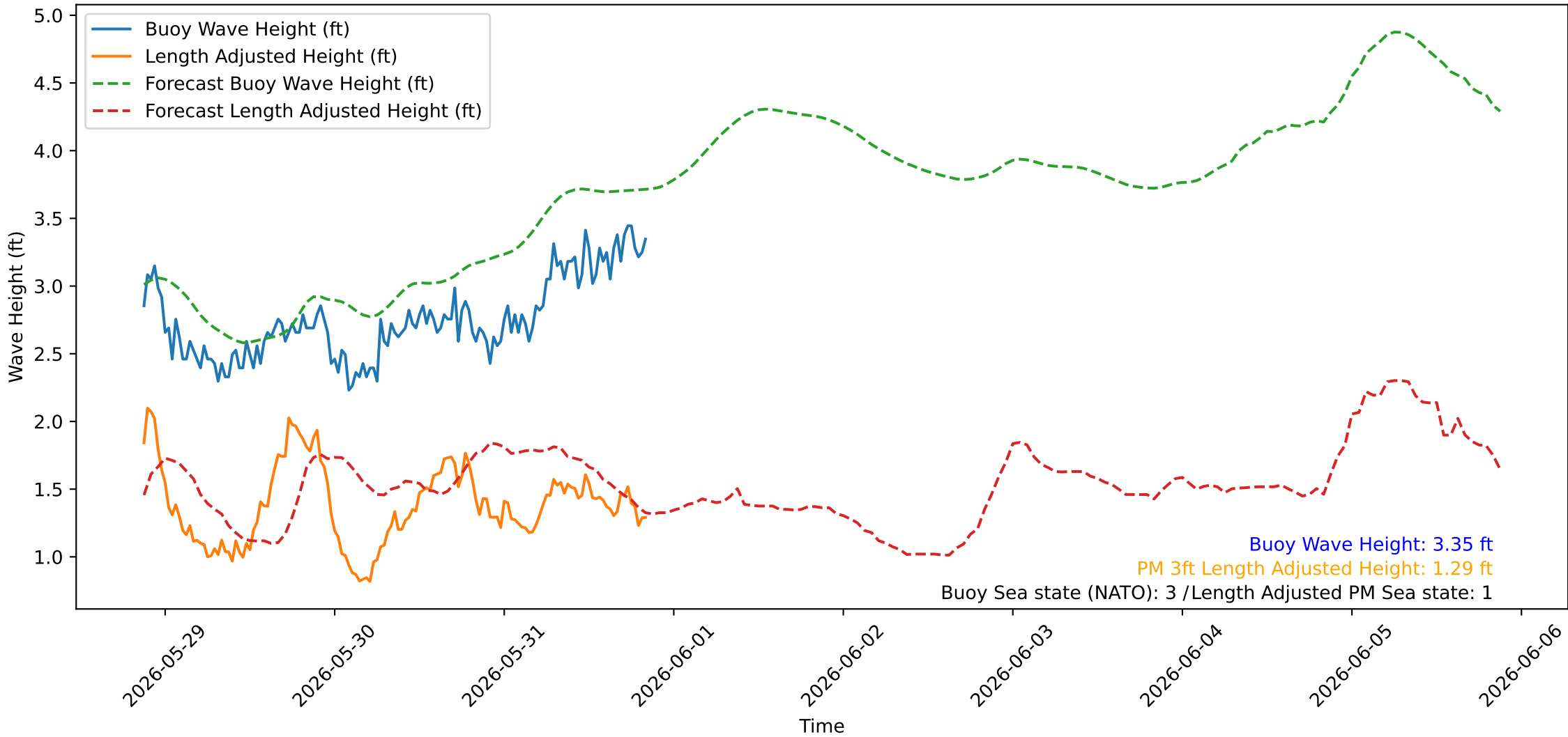
Wave Heights over Time for Red Beach at 2026-05-31 20:40:45
