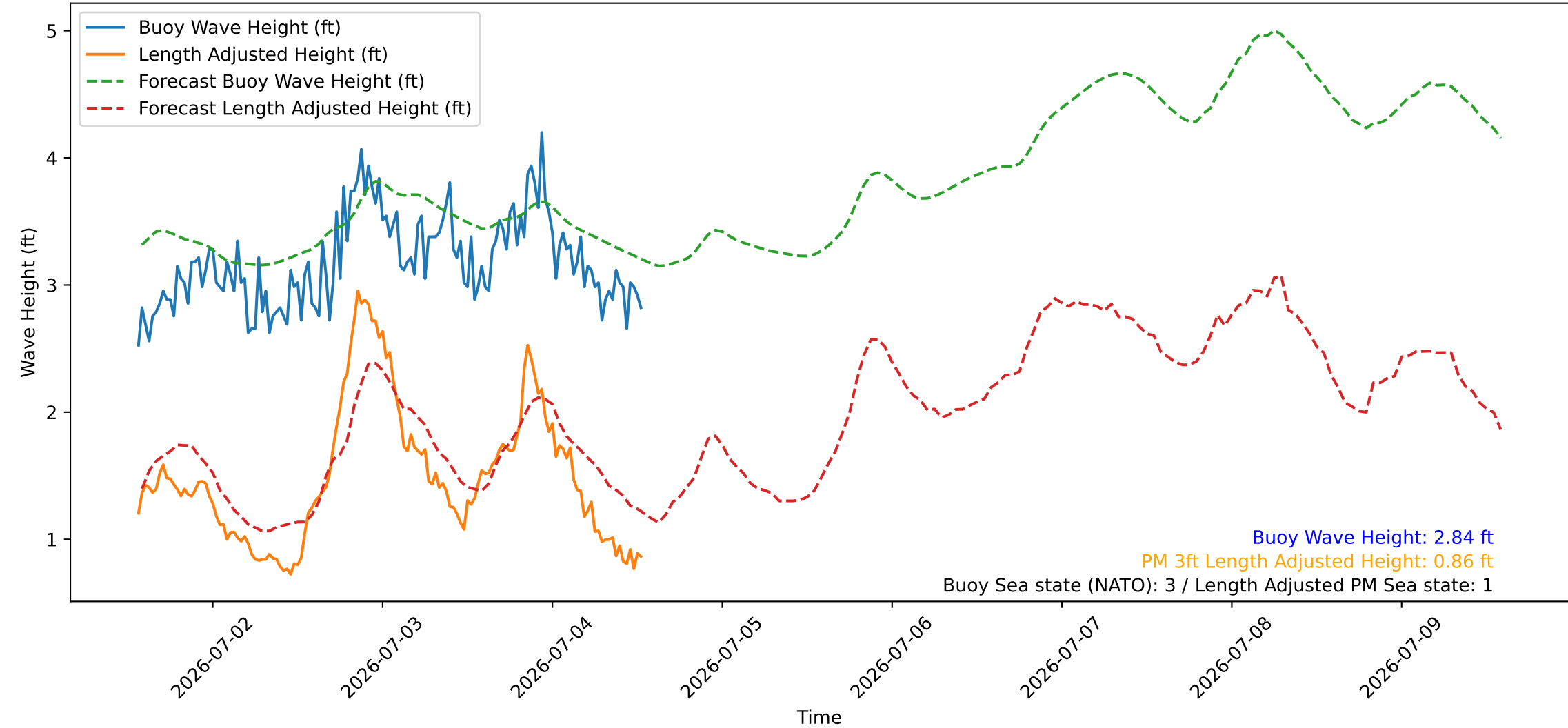
Wave Heights over Time for Green Beach at 2026-07-04 13:41:09
