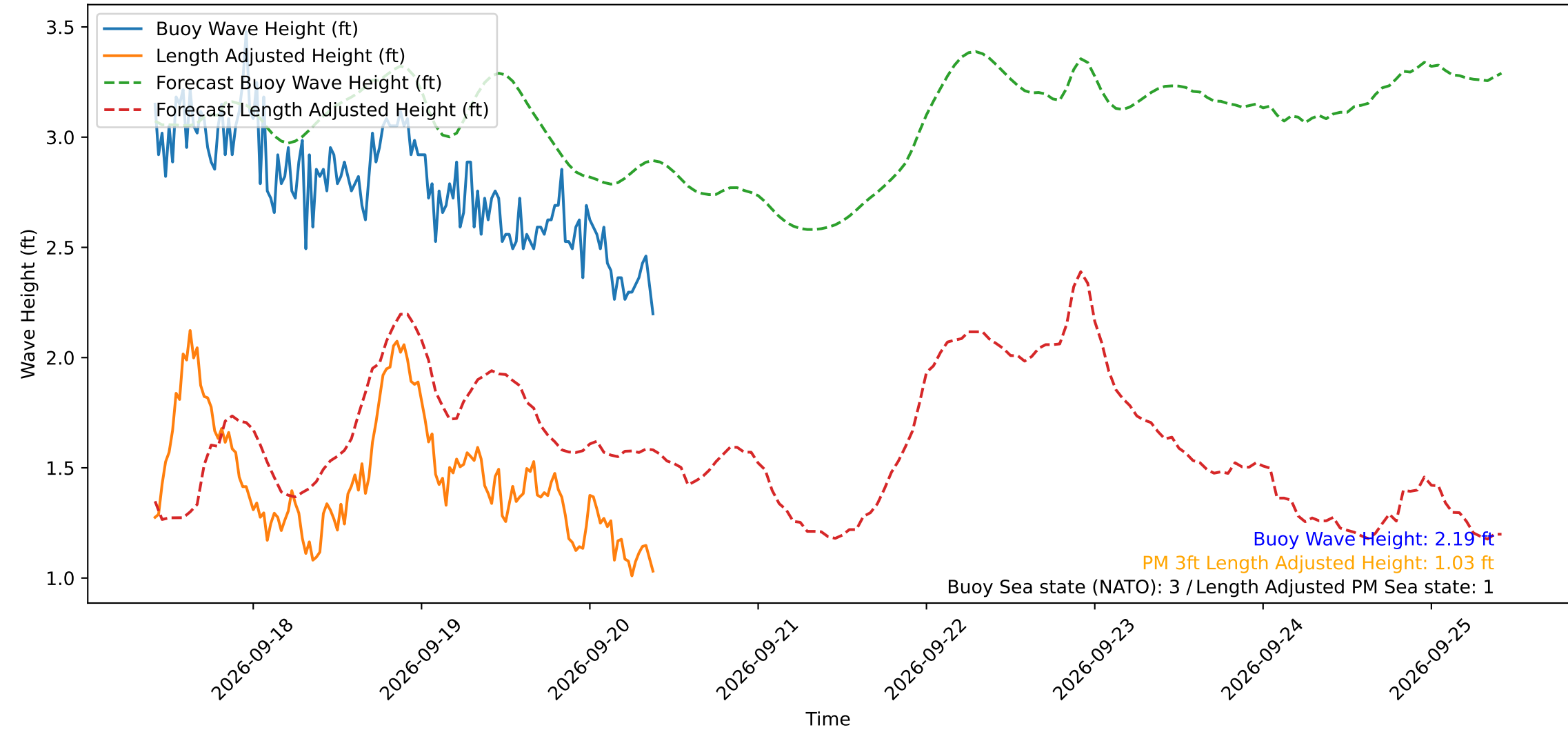
Wave Heights over Time for Green Beach at 2026-09-20 09:41:11
