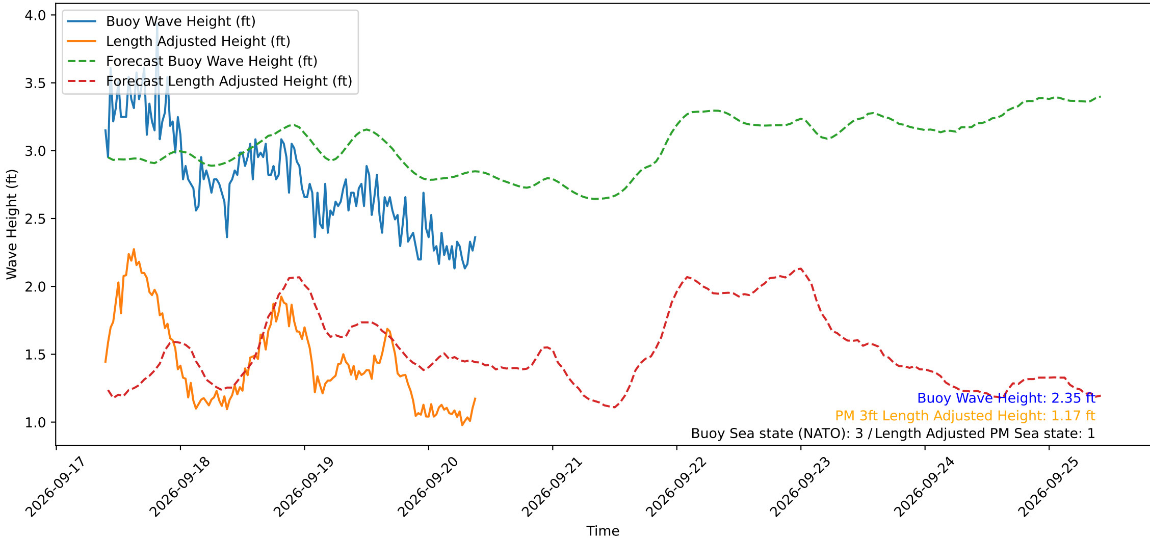
Wave Heights over Time for Oceanside Harbor at 2026-09-20 09:40:29
