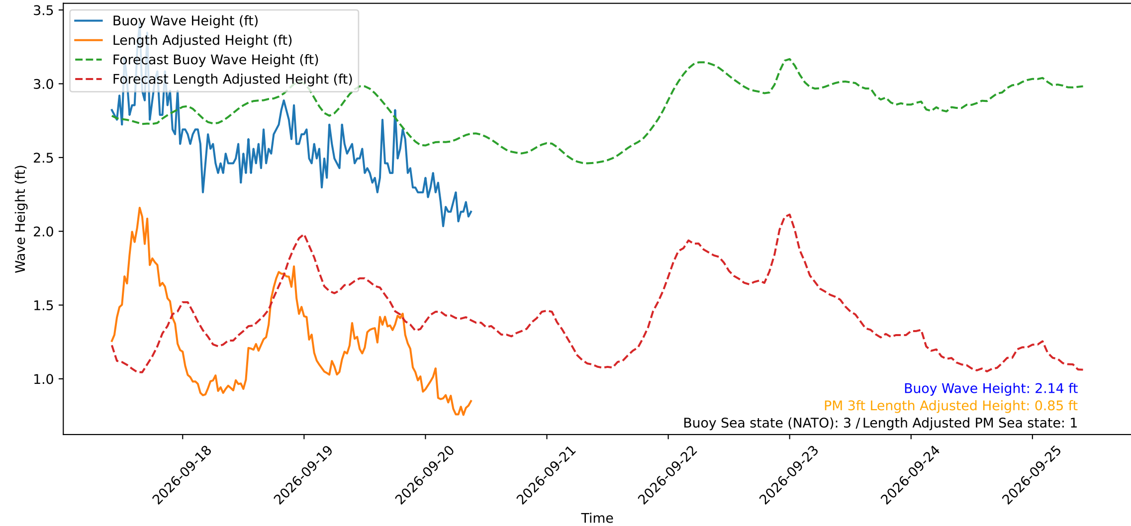
Wave Heights over Time for Red Beach at 2026-09-20 09:40:49
