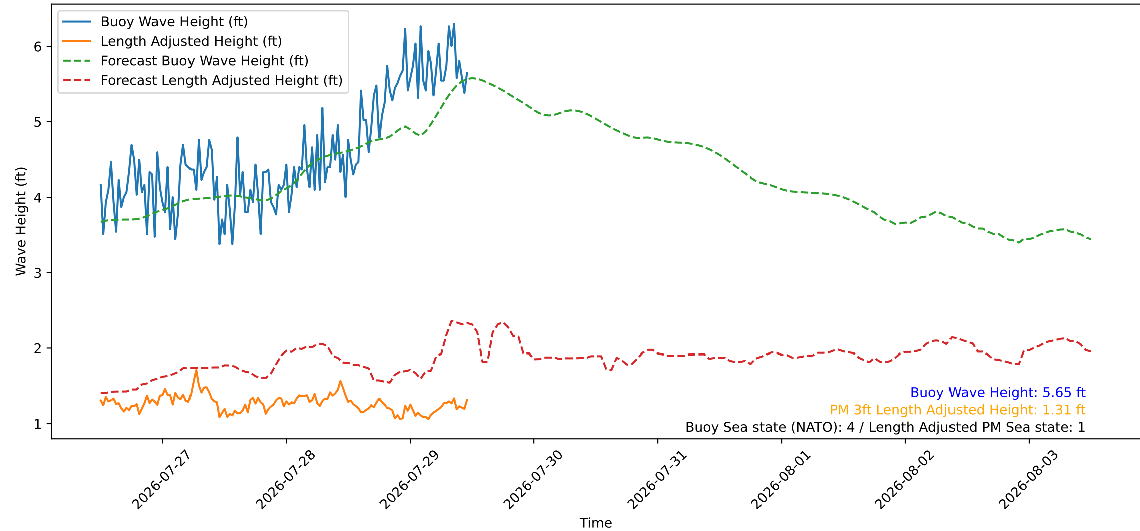
Wave Heights over Time for Green Beach at 2026-07-29 11:51:10
