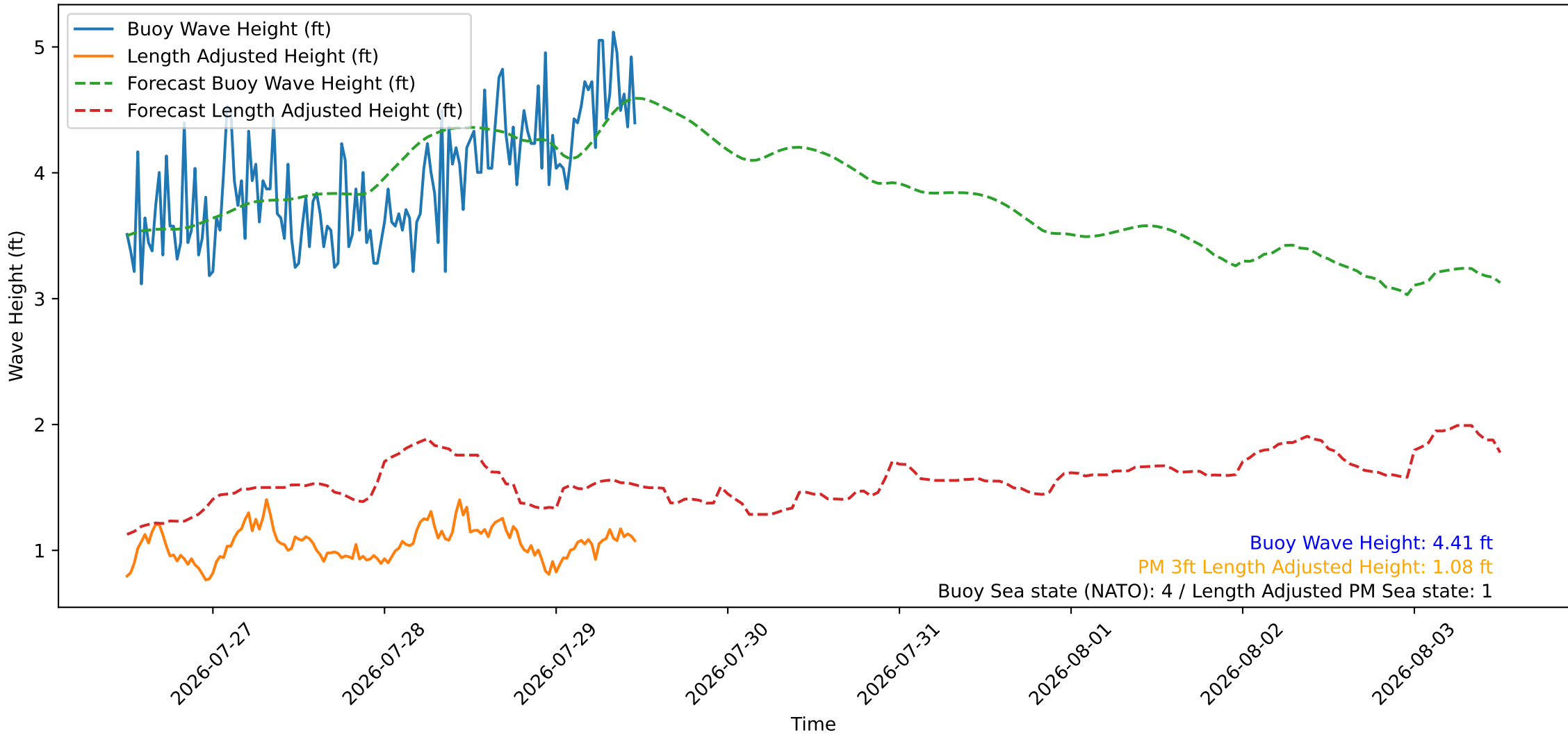
Wave Heights over Time for Red Beach at 2026-07-29 11:50:48
