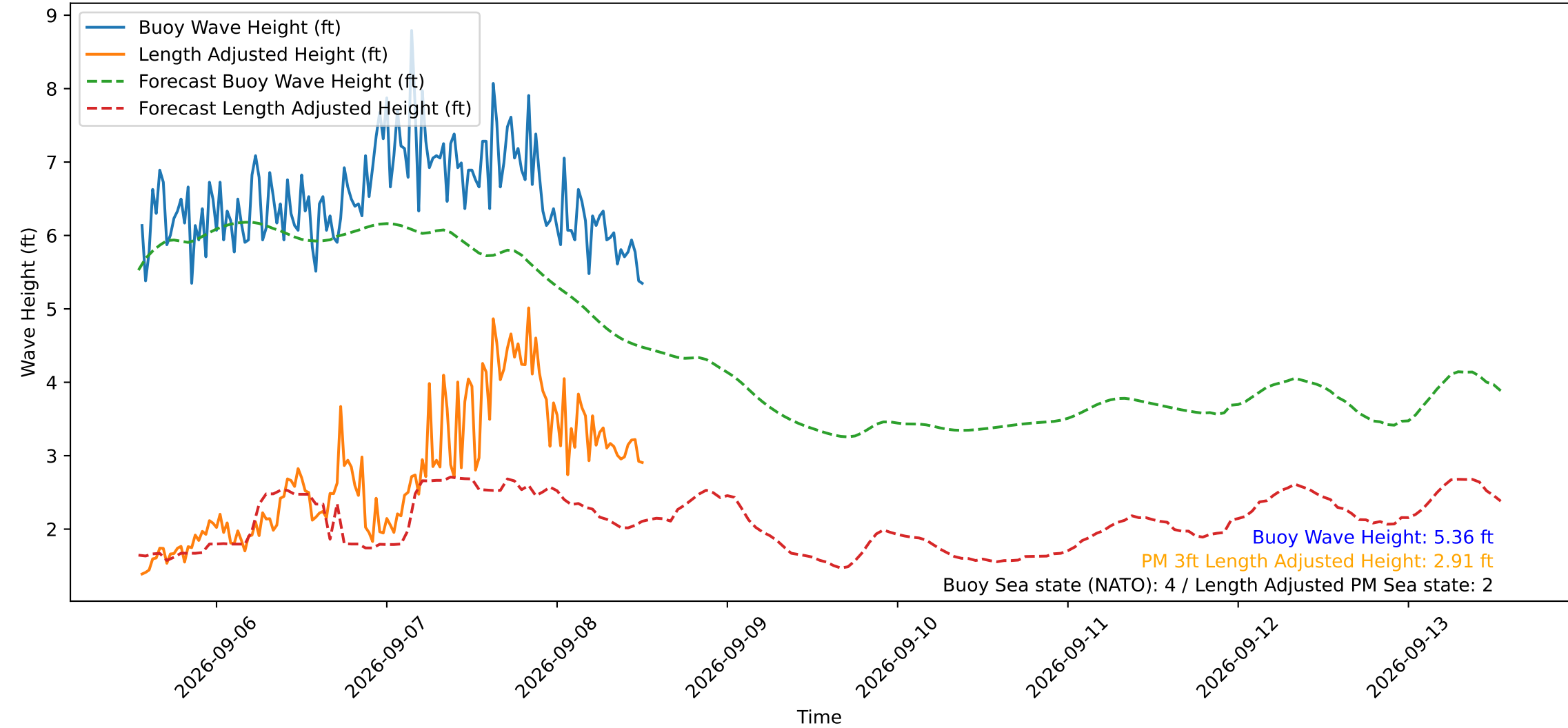
Wave Heights over Time for Green Beach at 2026-09-08 13:01:11
