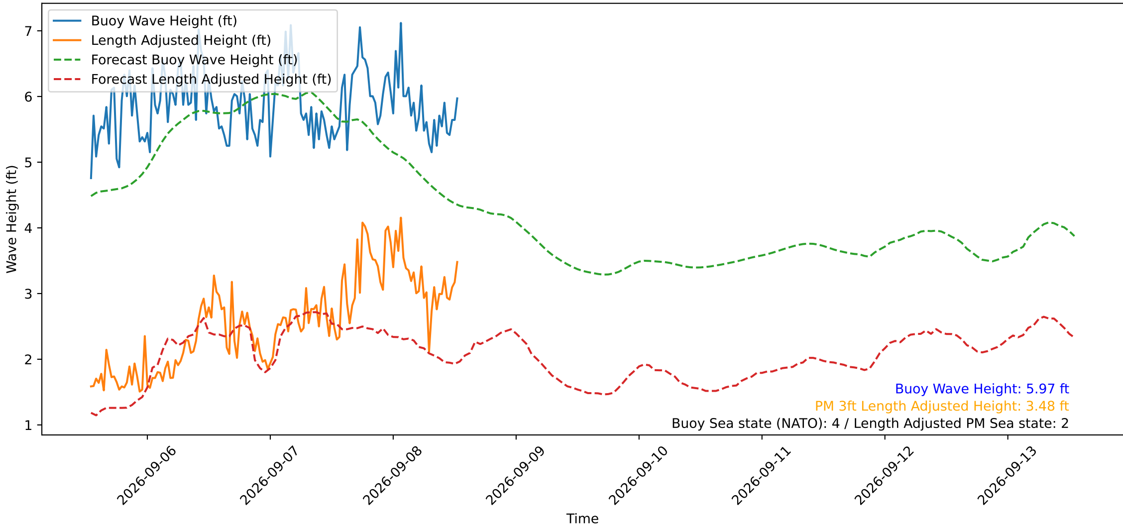
Wave Heights over Time for Oceanside Harbor at 2026-09-08 13:00:29
