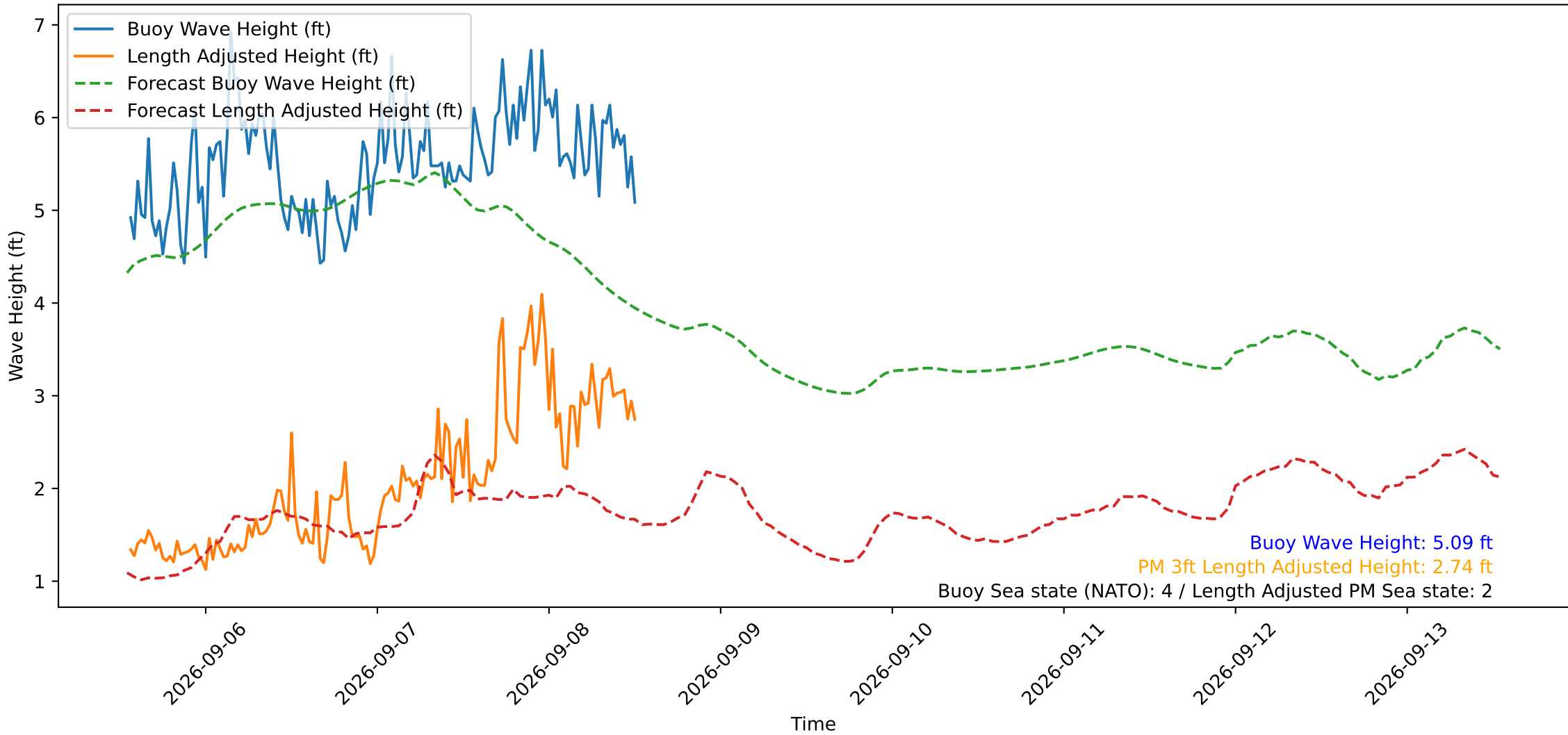
Wave Heights over Time for Red Beach at 2026-09-08 13:00:49
