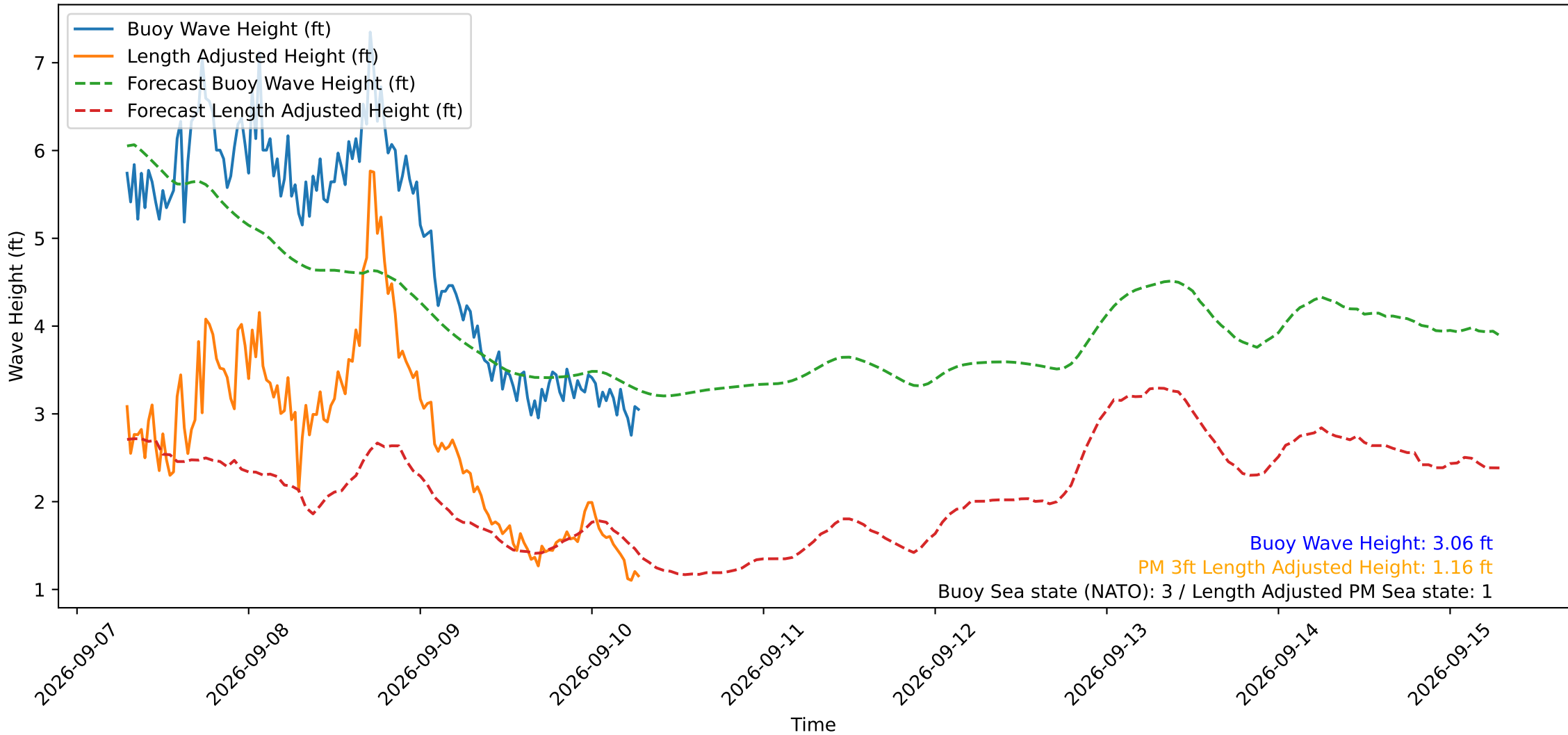
Wave Heights over Time for Oceanside Harbor at 2026-09-10 07:10:30
