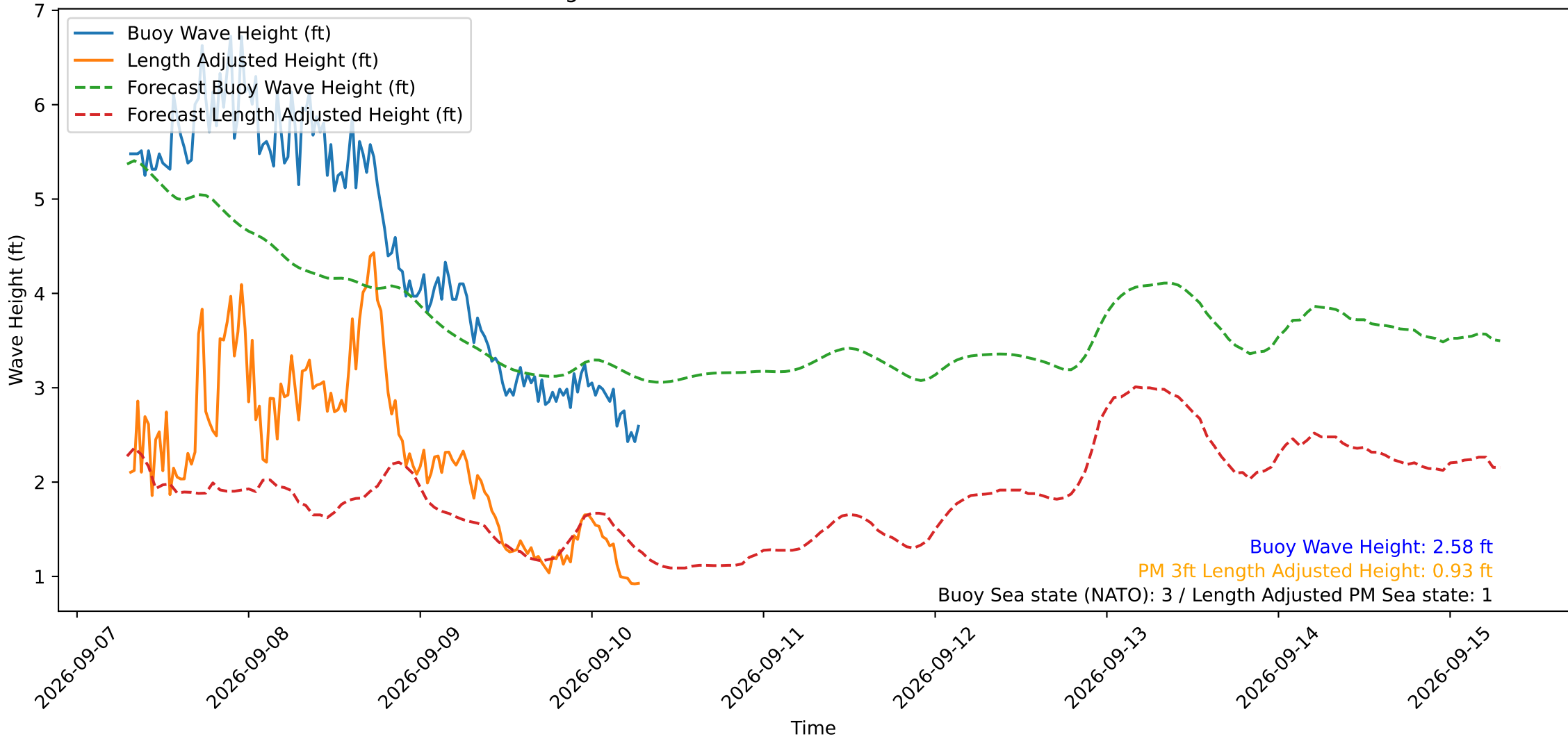
Wave Heights over Time for Red Beach at 2026-09-10 07:10:49
