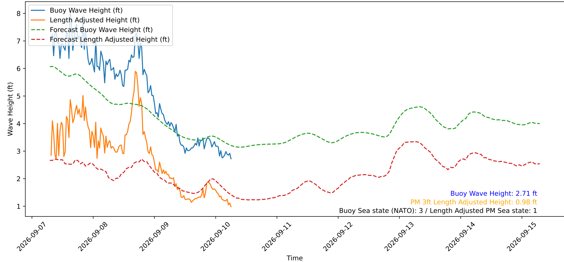
Wave Heights over Time for Green Beach at 2026-09-10 07:11:12
