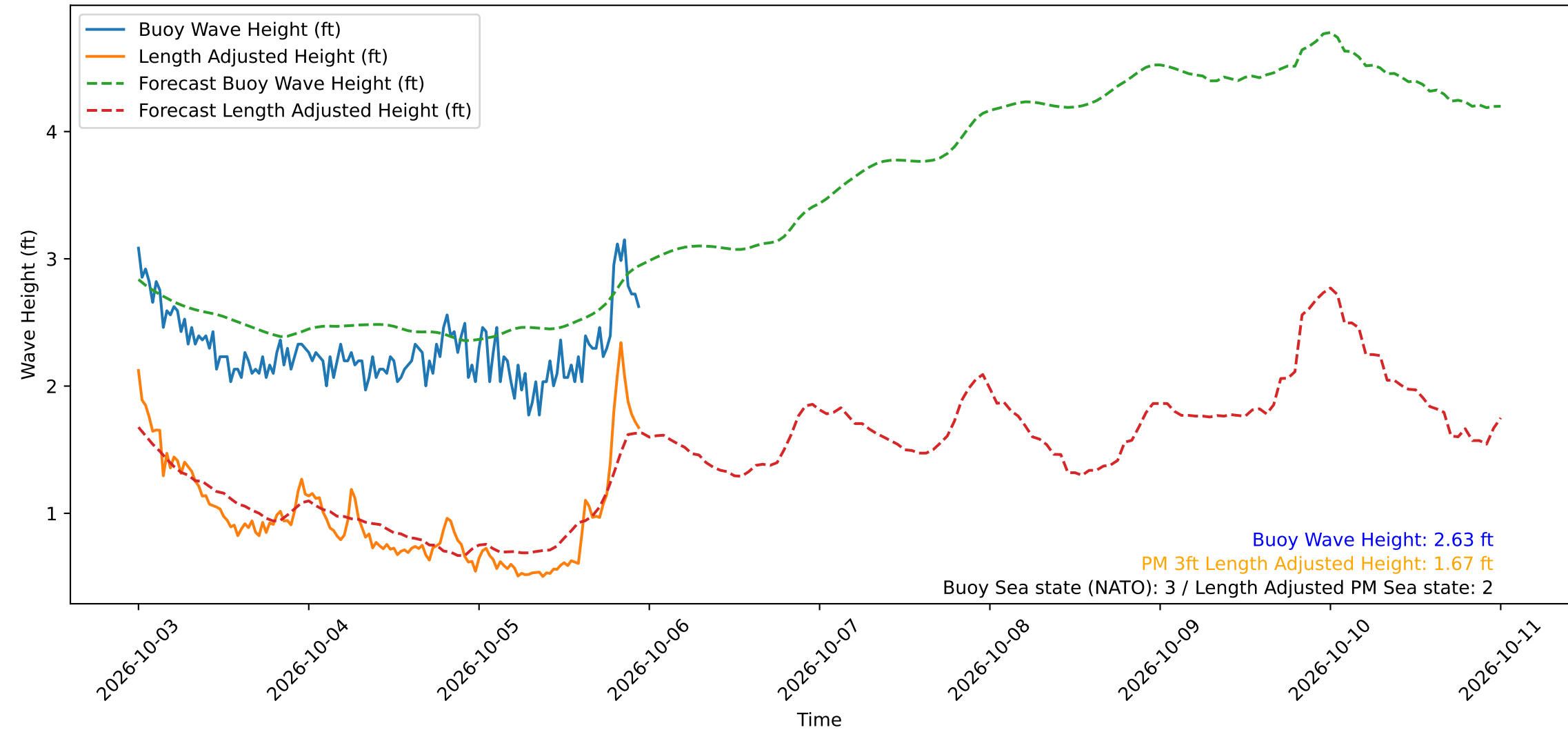
Wave Heights over Time for Green Beach at 2026-10-05 23:31:12
