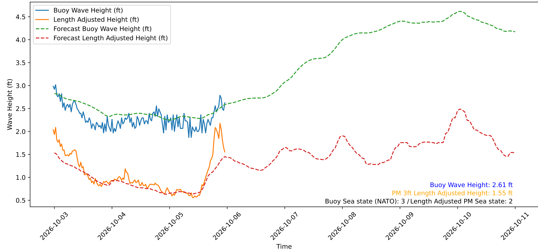
Wave Heights over Time for Oceanside Harbor at 2026-10-05 23:30:29
