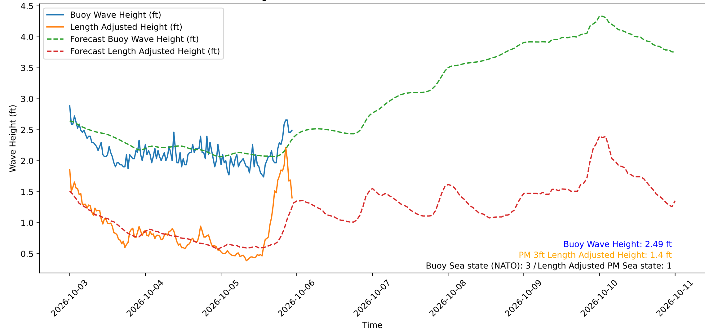
Wave Heights over Time for Red Beach at 2026-10-05 23:30:49
