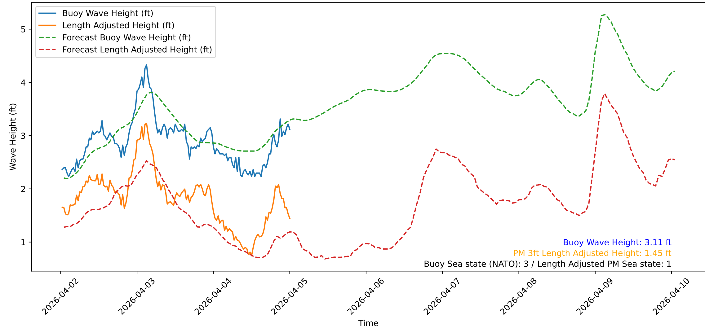
Wave Heights over Time for Green Beach at 2026-04-05 00:41:10
