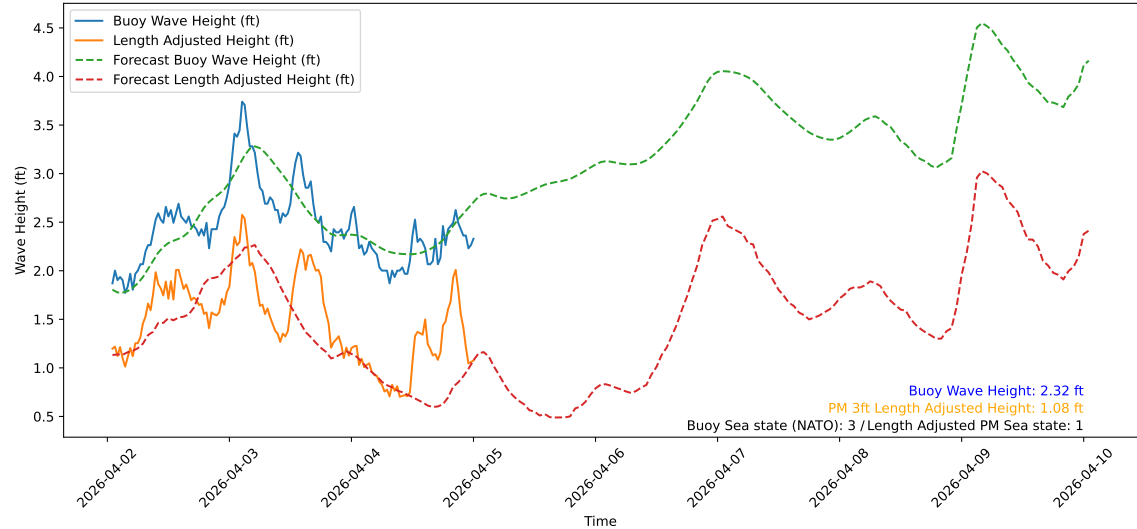
Wave Heights over Time for Red Beach at 2026-04-05 00:40:48
