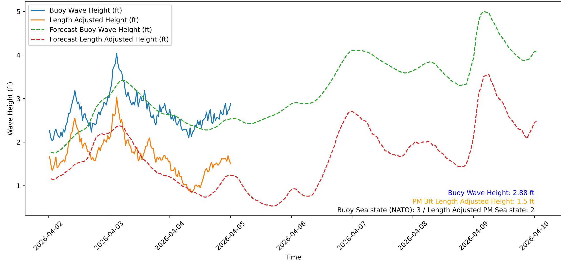
Wave Heights over Time for Oceanside Harbor at 2026-04-05 00:40:32
