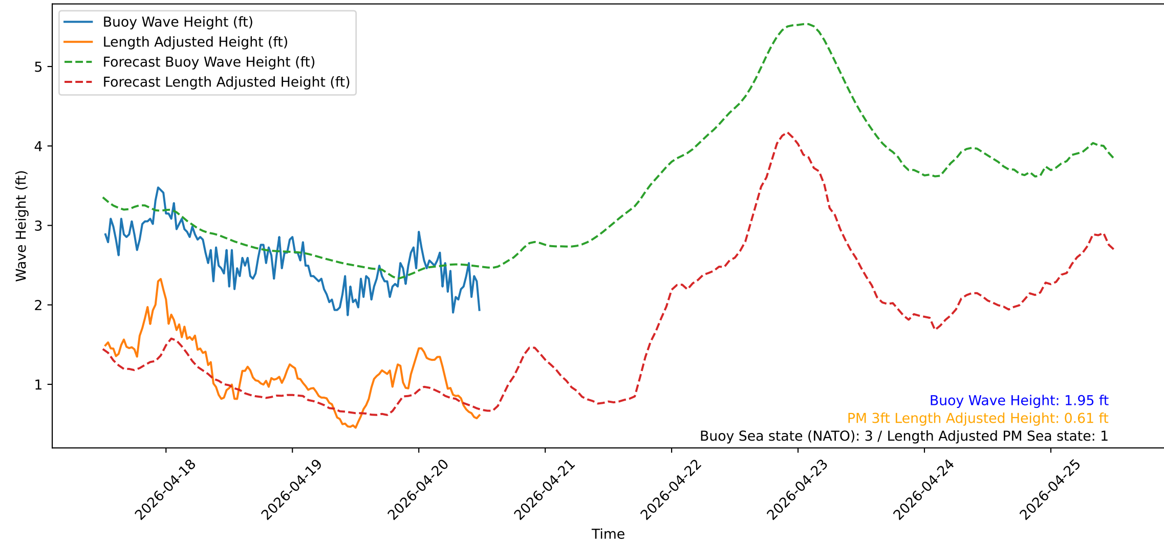
Wave Heights over Time for Green Beach at 2026-04-20 12:21:13
