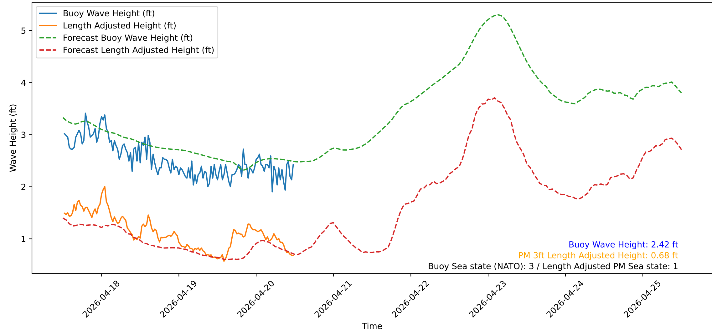
Wave Heights over Time for Oceanside Harbor at 2026-04-20 12:20:31
