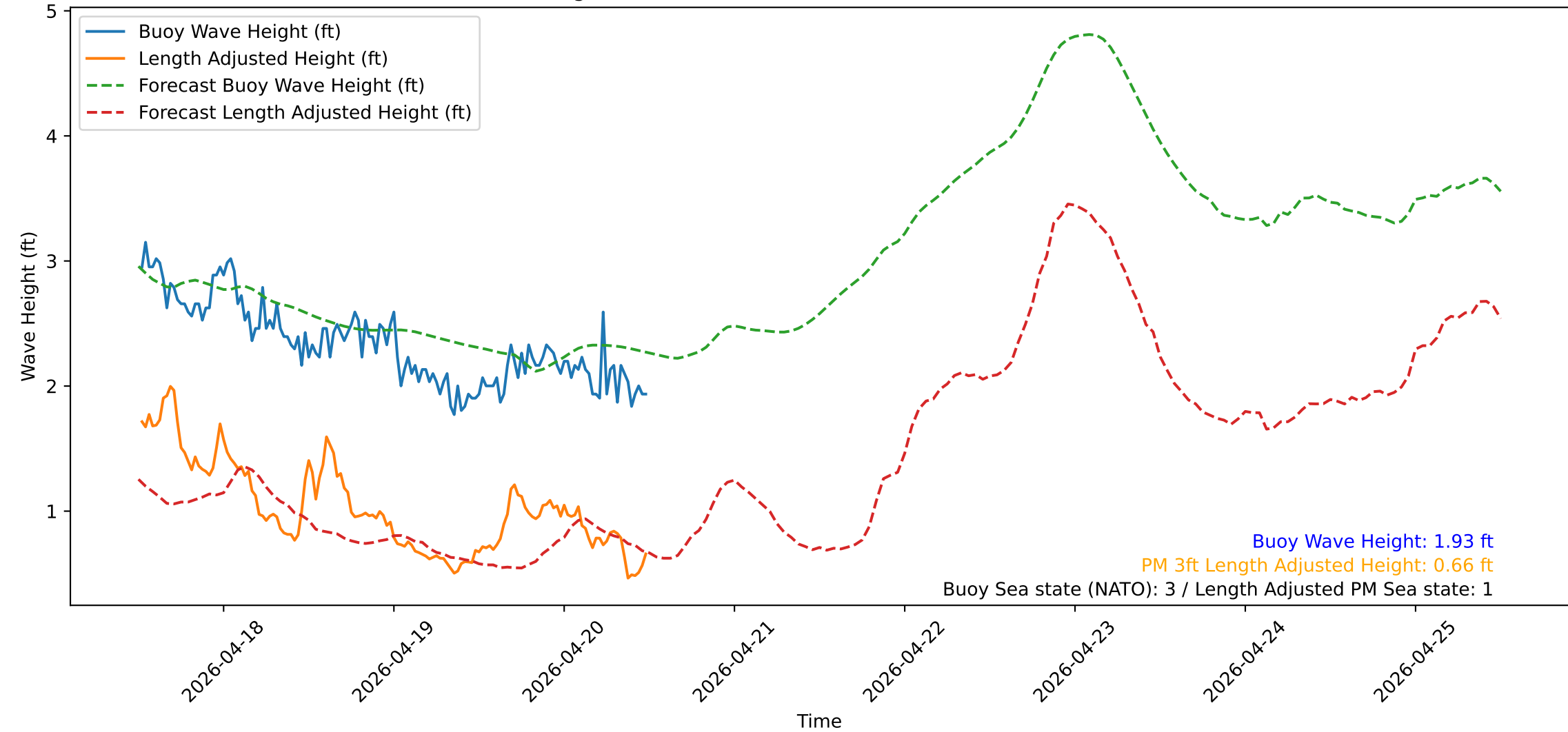
Wave Heights over Time for Red Beach at 2026-04-20 12:20:51
