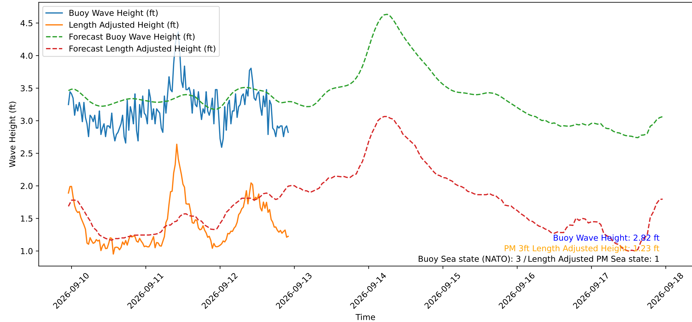
Wave Heights over Time for Oceanside Harbor at 2026-09-12 23:00:30
