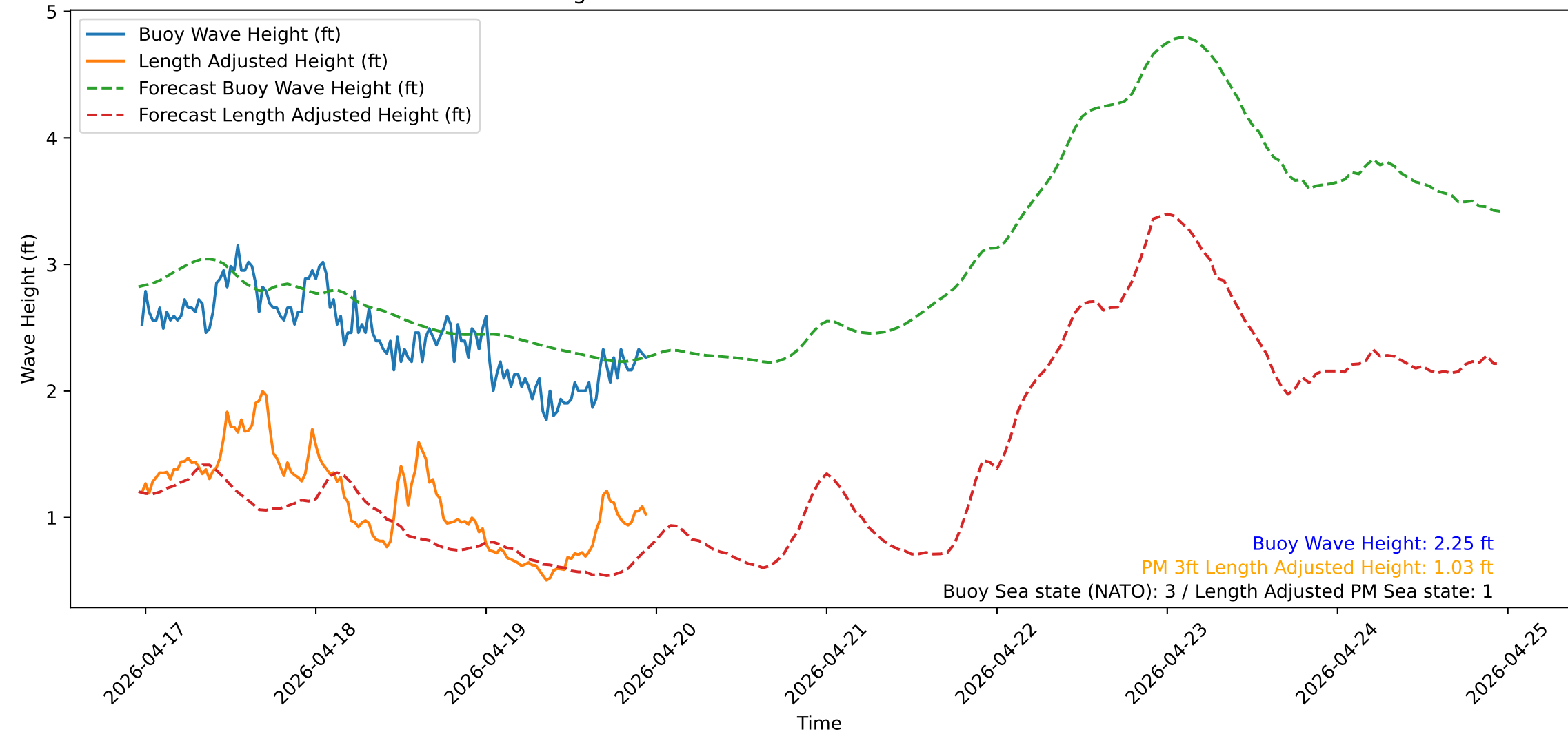
Wave Heights over Time for Red Beach at 2026-04-19 23:20:51
