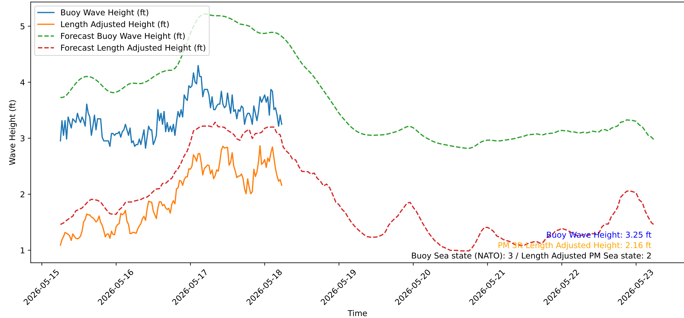
Wave Heights over Time for Oceanside Harbor at 2026-05-18 06:00:32
