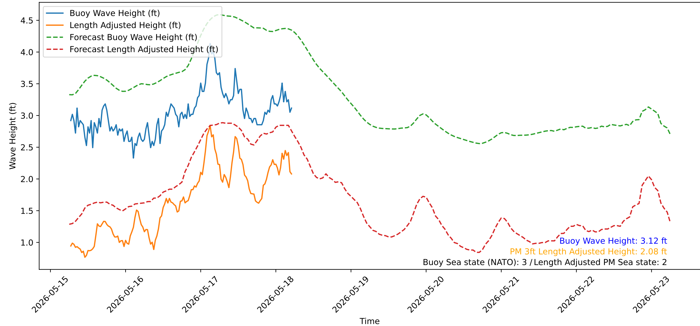
Wave Heights over Time for Red Beach at 2026-05-18 06:00:51
