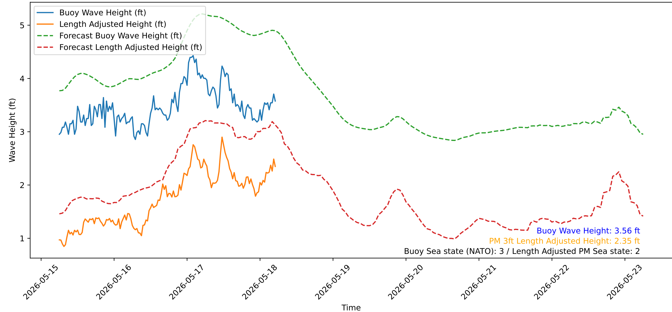
Wave Heights over Time for Green Beach at 2026-05-18 06:01:14
