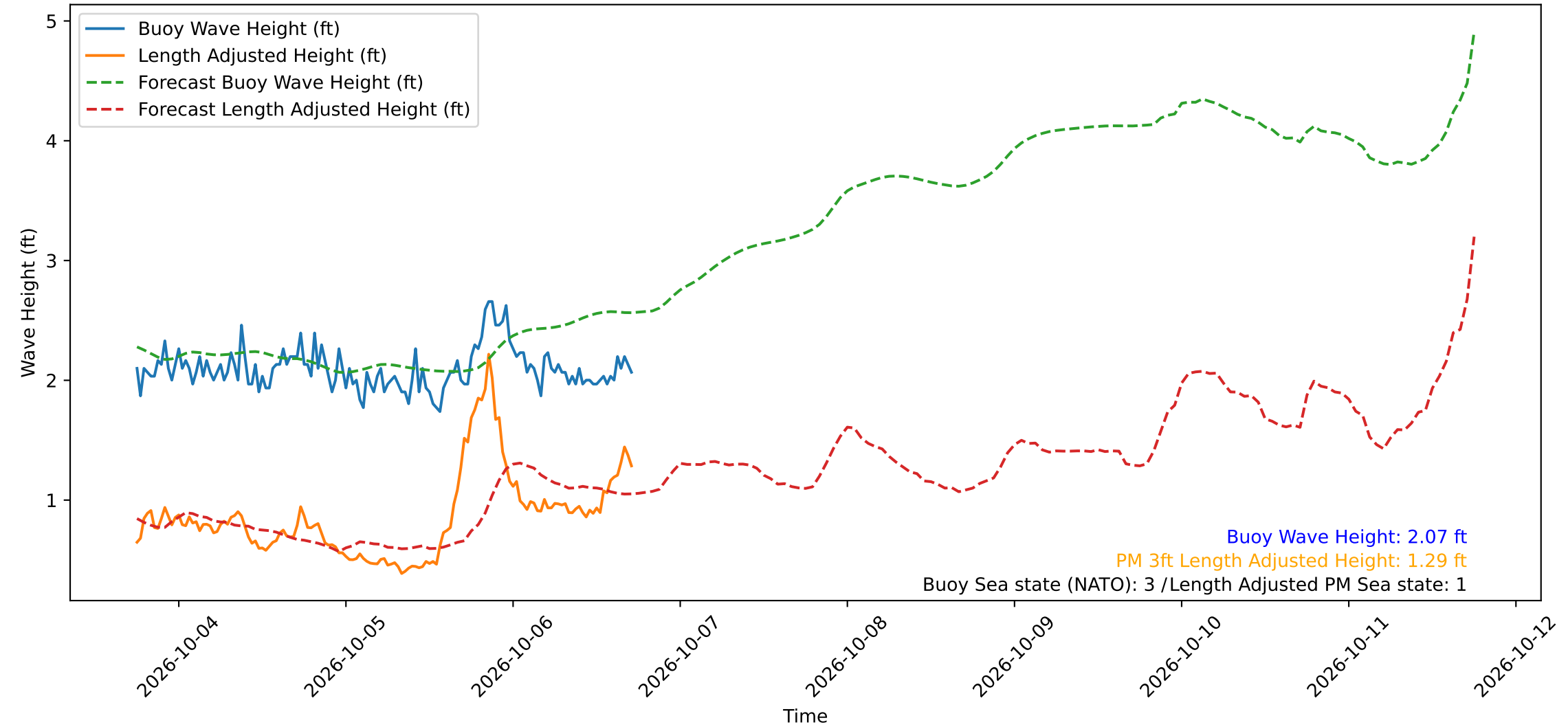
Wave Heights over Time for Red Beach at 2026-10-06 17:40:49
