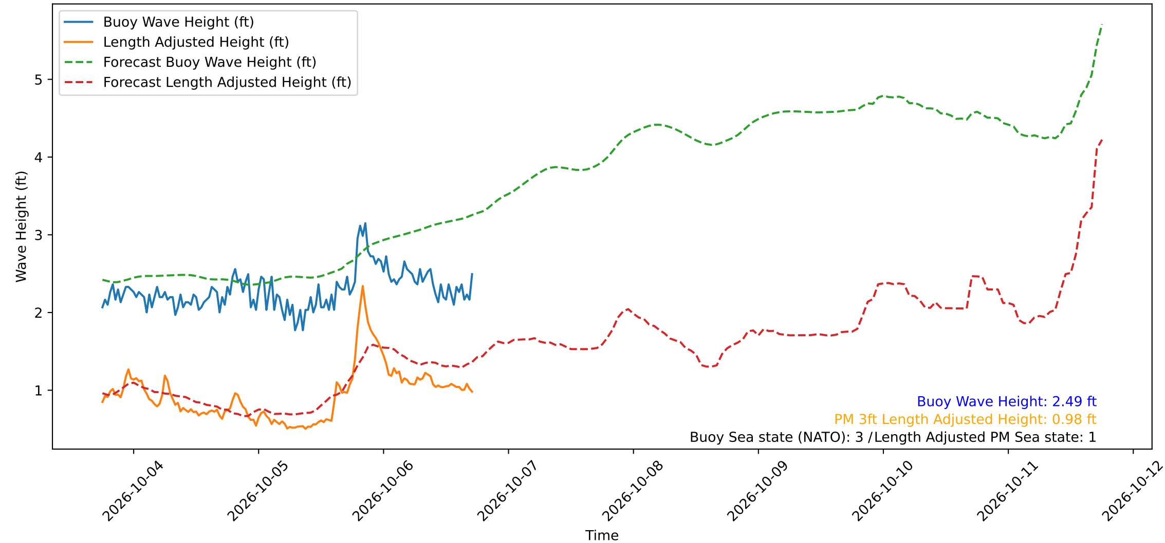
Wave Heights over Time for Green Beach at 2026-10-06 17:41:12
