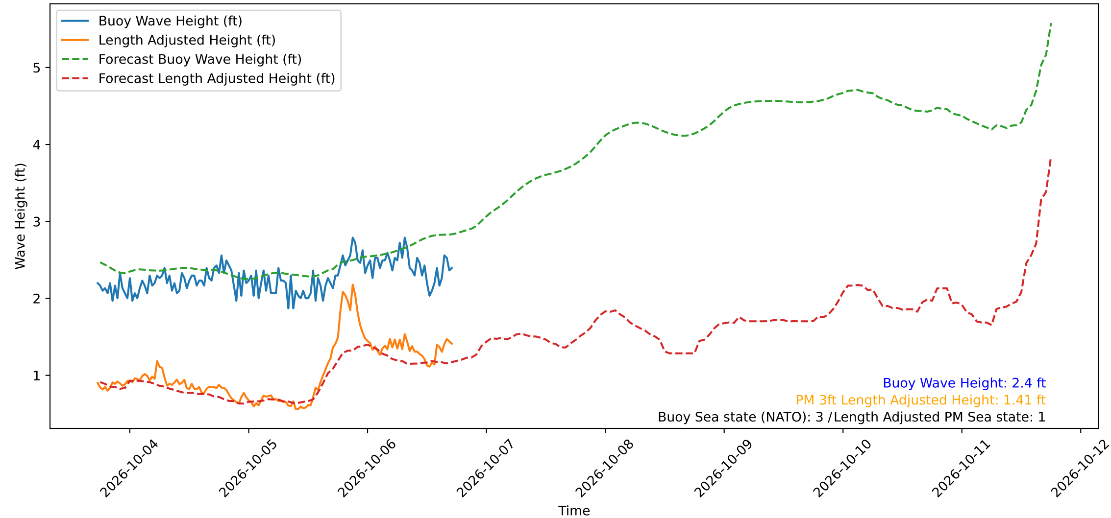
Wave Heights over Time for Oceanside Harbor at 2026-10-06 17:40:29
