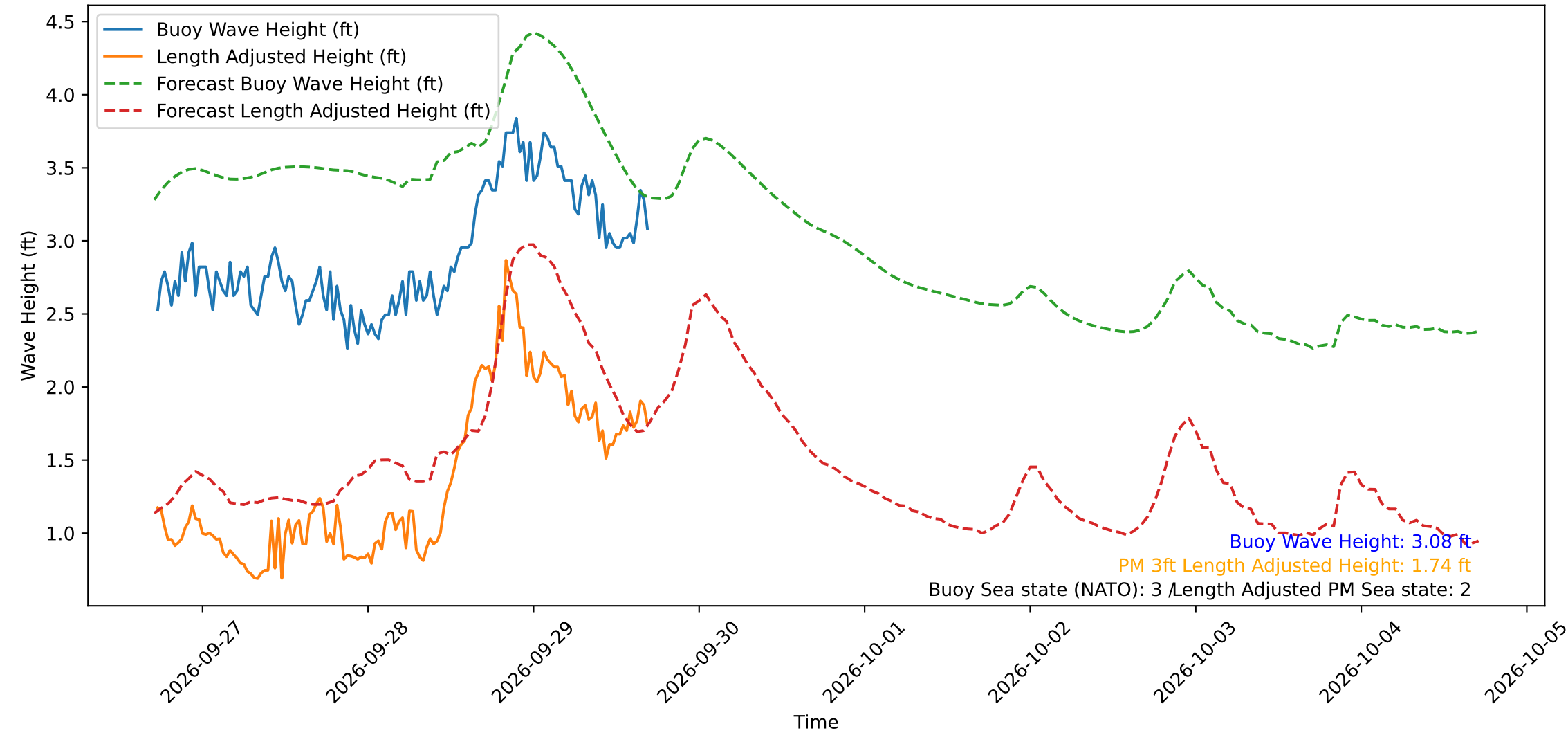
Wave Heights over Time for Red Beach at 2026-09-29 17:20:51
