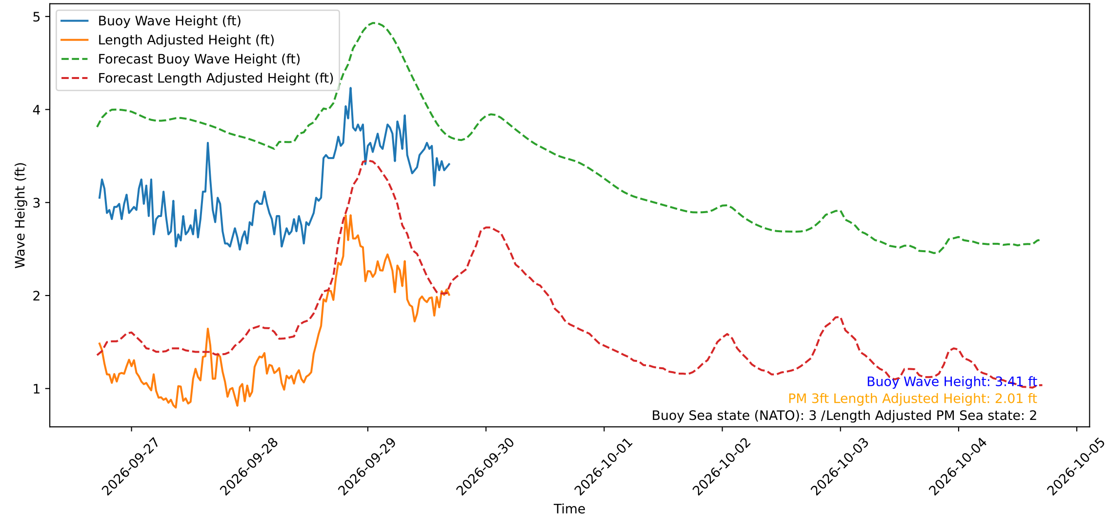
Wave Heights over Time for Oceanside Harbor at 2026-09-29 17:20:30
