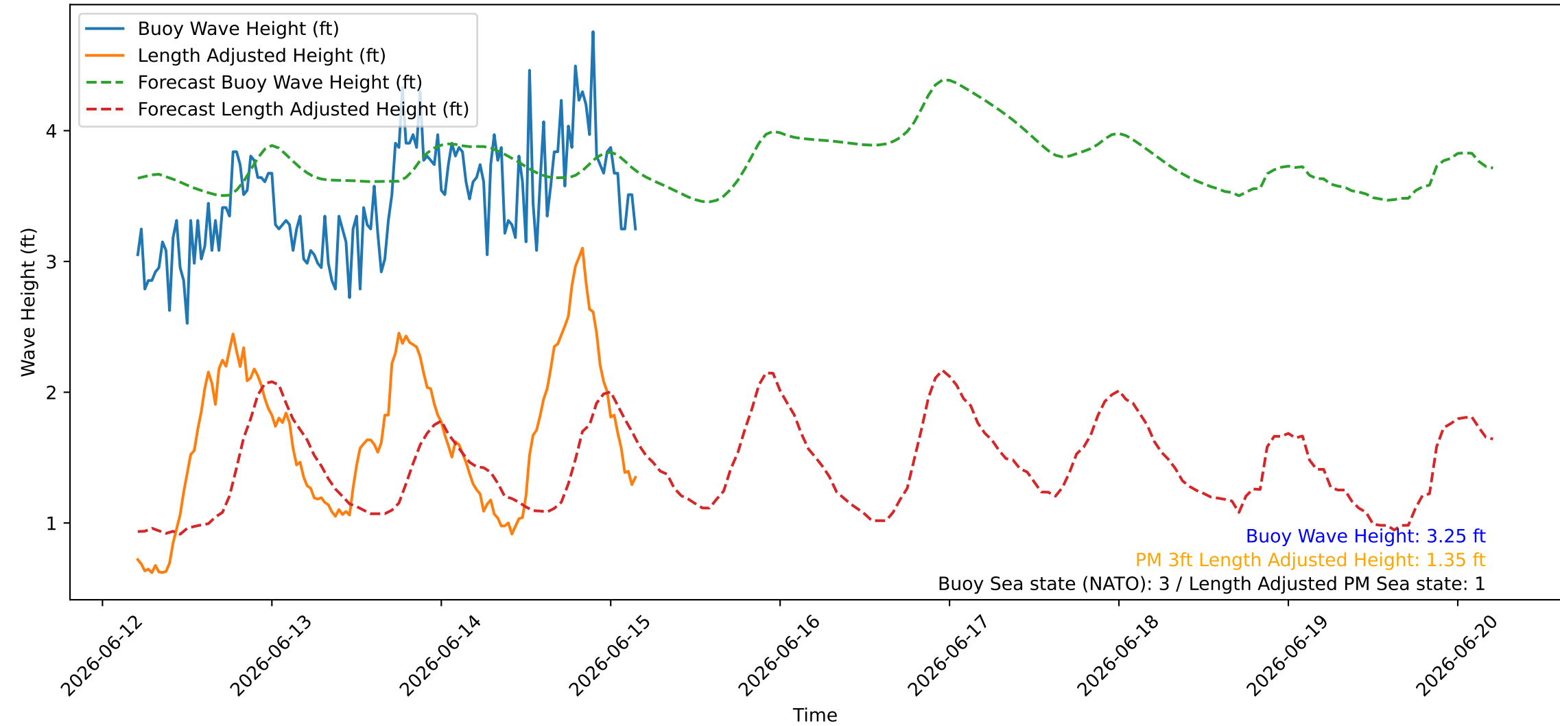
Wave Heights over Time for Red Beach at 2026-06-15 04:30:45
