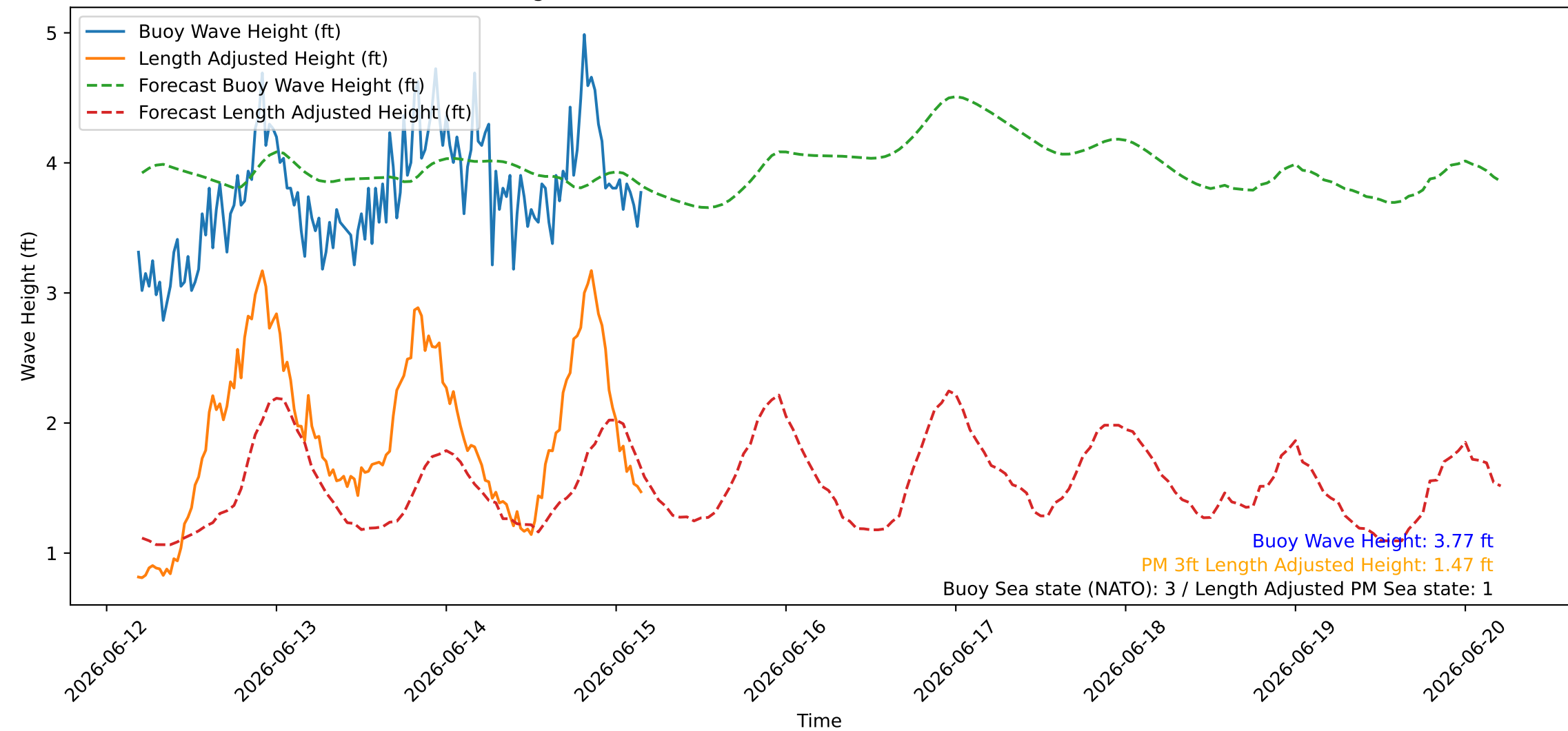
Wave Heights over Time for Oceanside Harbor at 2026-06-15 04:30:26
