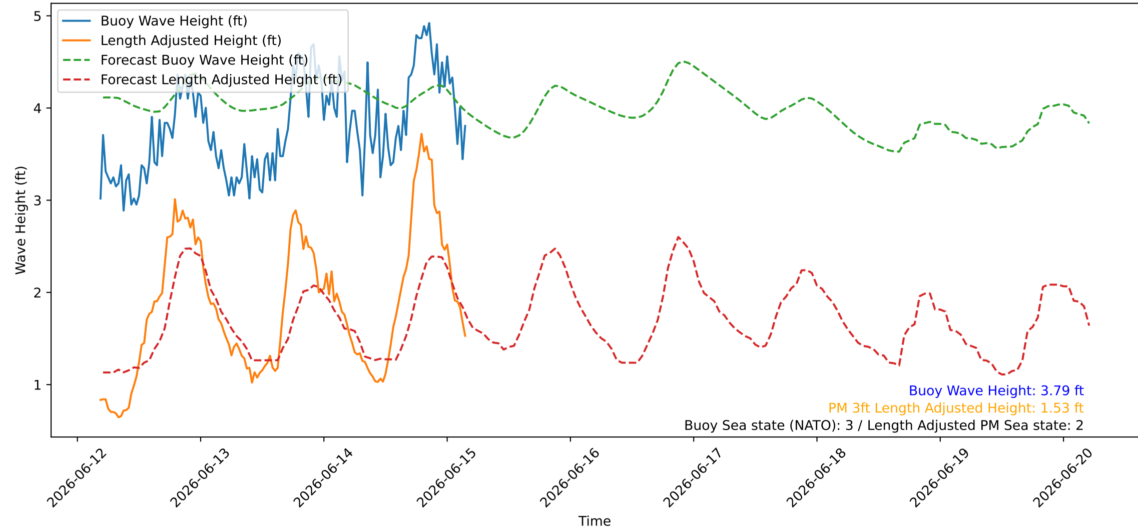
Wave Heights over Time for Green Beach at 2026-06-15 04:31:07
