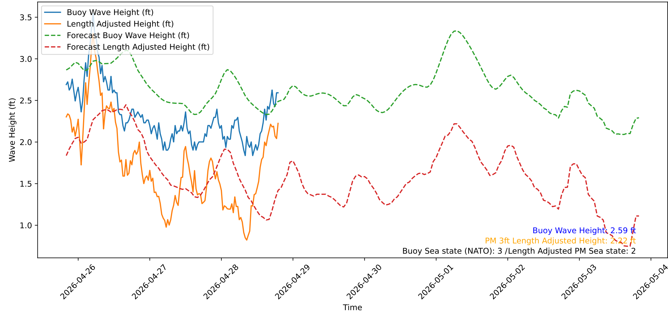
Wave Heights over Time for Red Beach at 2026-04-28 19:50:52
