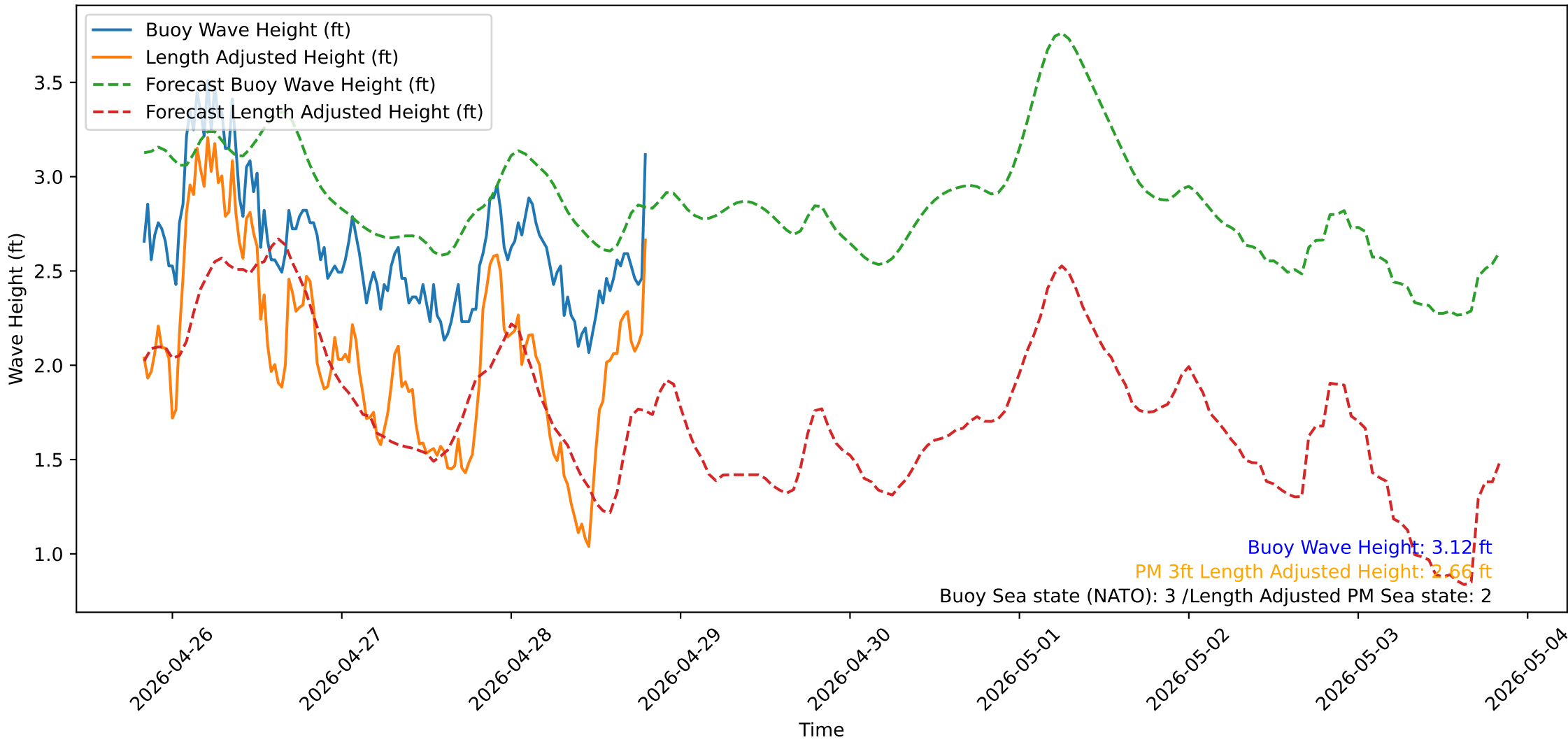
Wave Heights over Time for Green Beach at 2026-04-28 19:51:14
