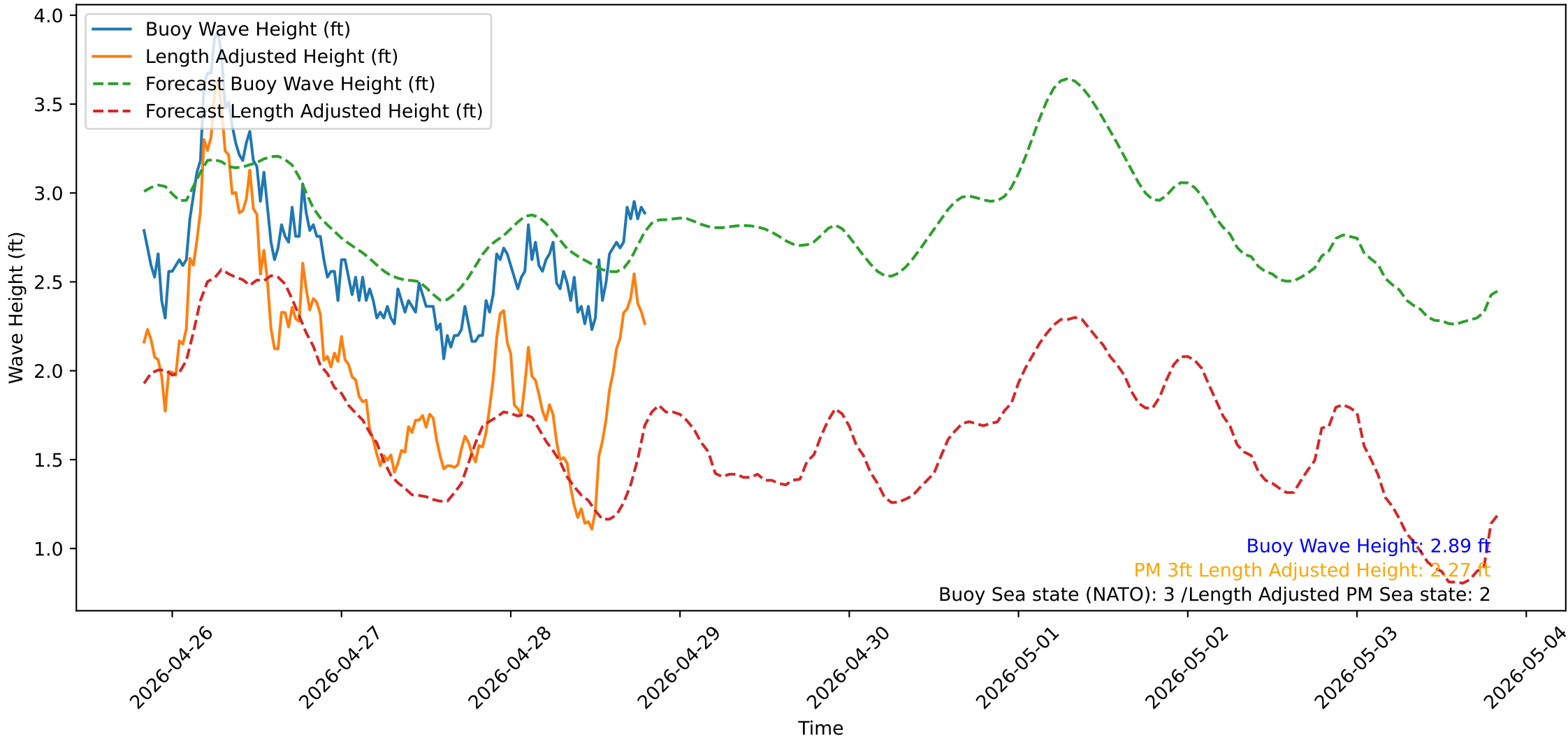
Wave Heights over Time for Oceanside Harbor at 2026-04-28 19:50:31
