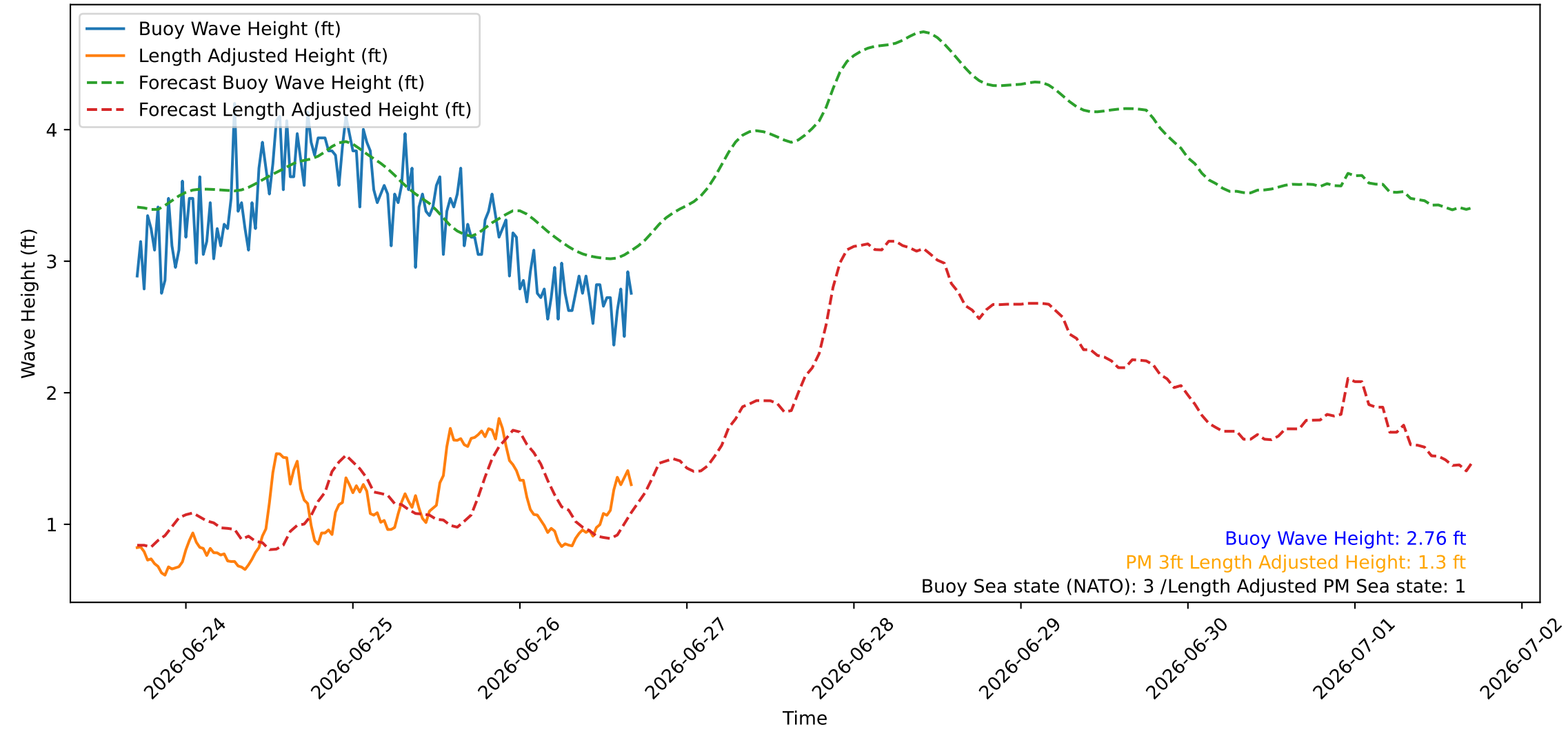
Wave Heights over Time for Green Beach at 2026-06-26 17:01:08
