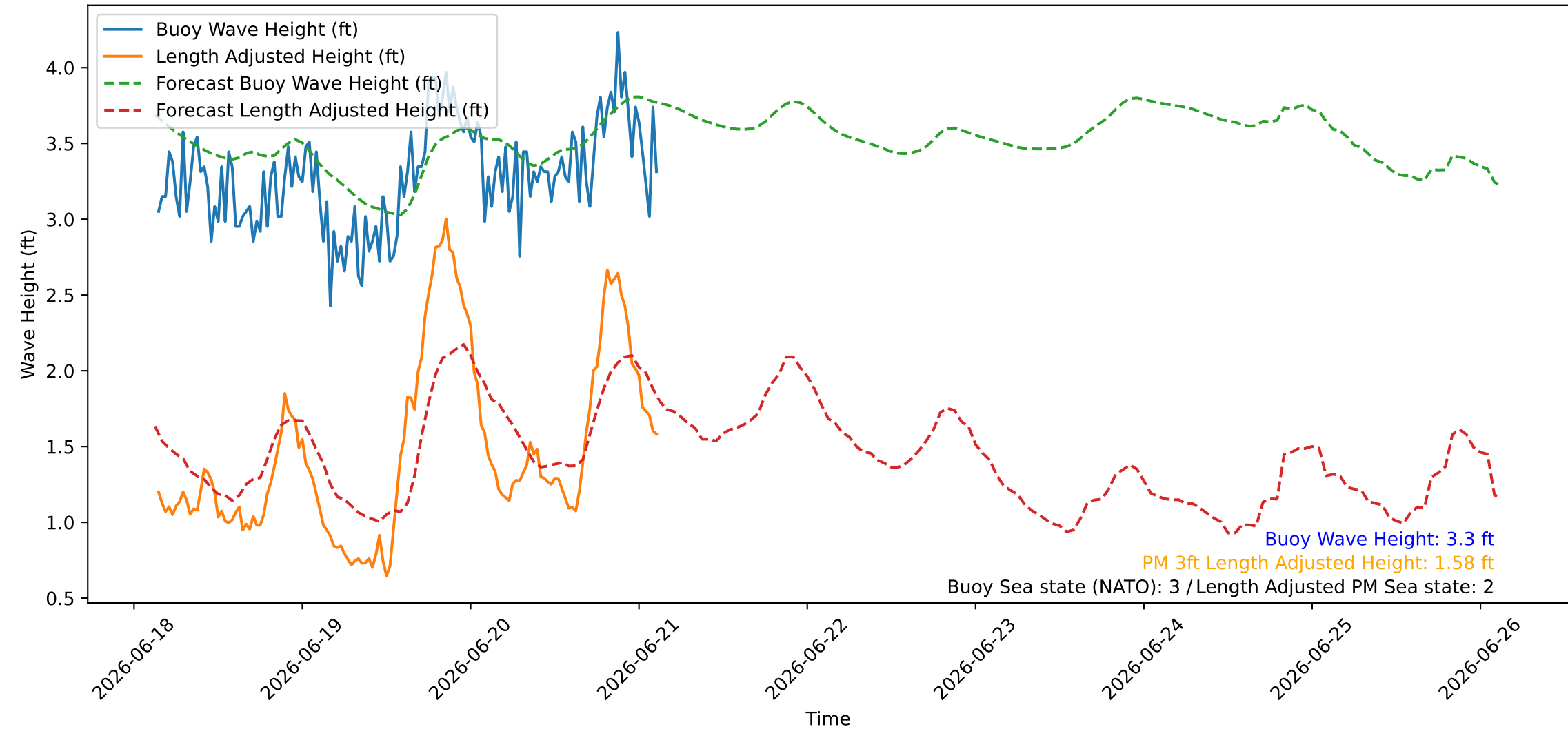
Wave Heights over Time for Green Beach at 2026-06-21 03:21:08
