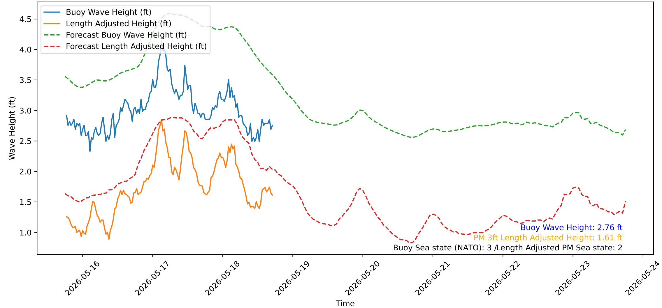
Wave Heights over Time for Red Beach at 2026-05-18 18:10:51
