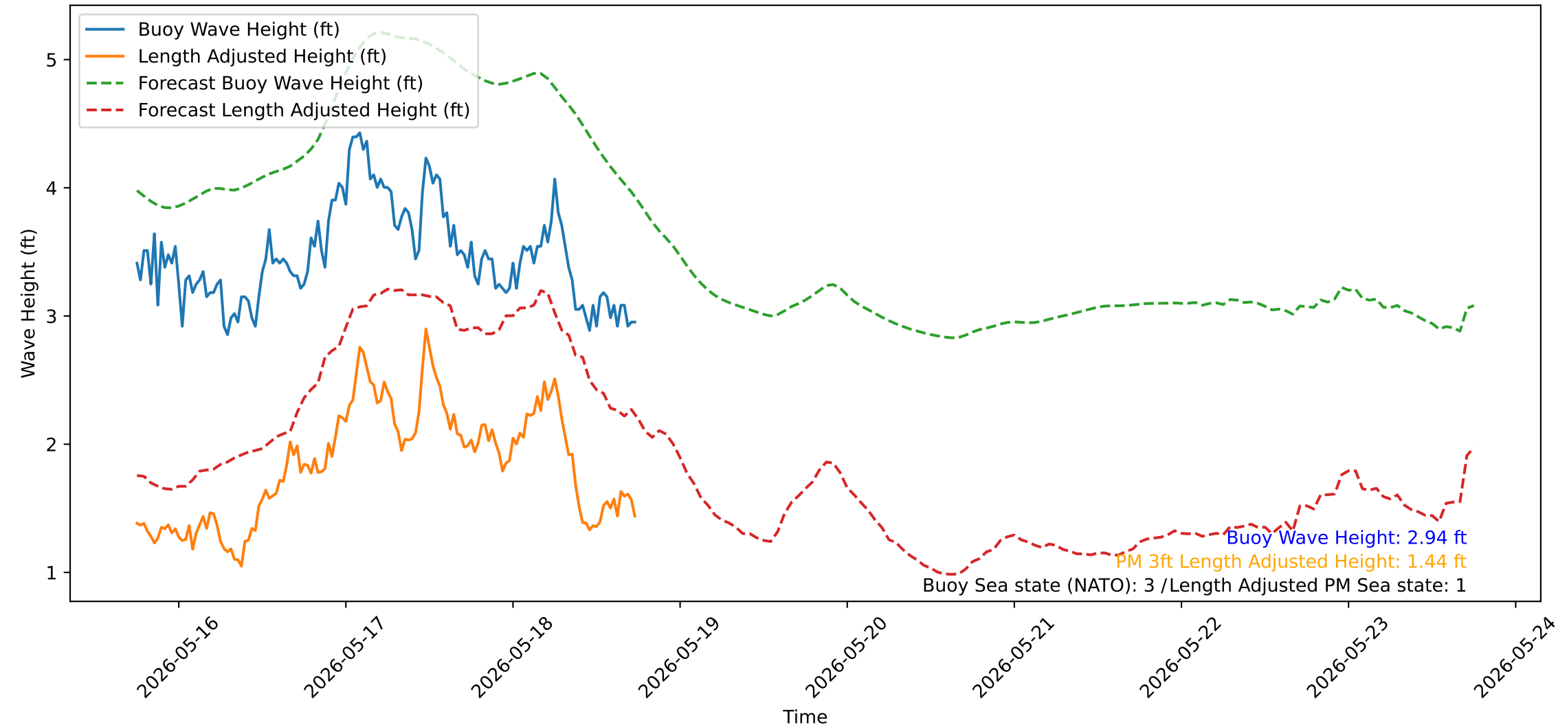
Wave Heights over Time for Green Beach at 2026-05-18 18:11:14
