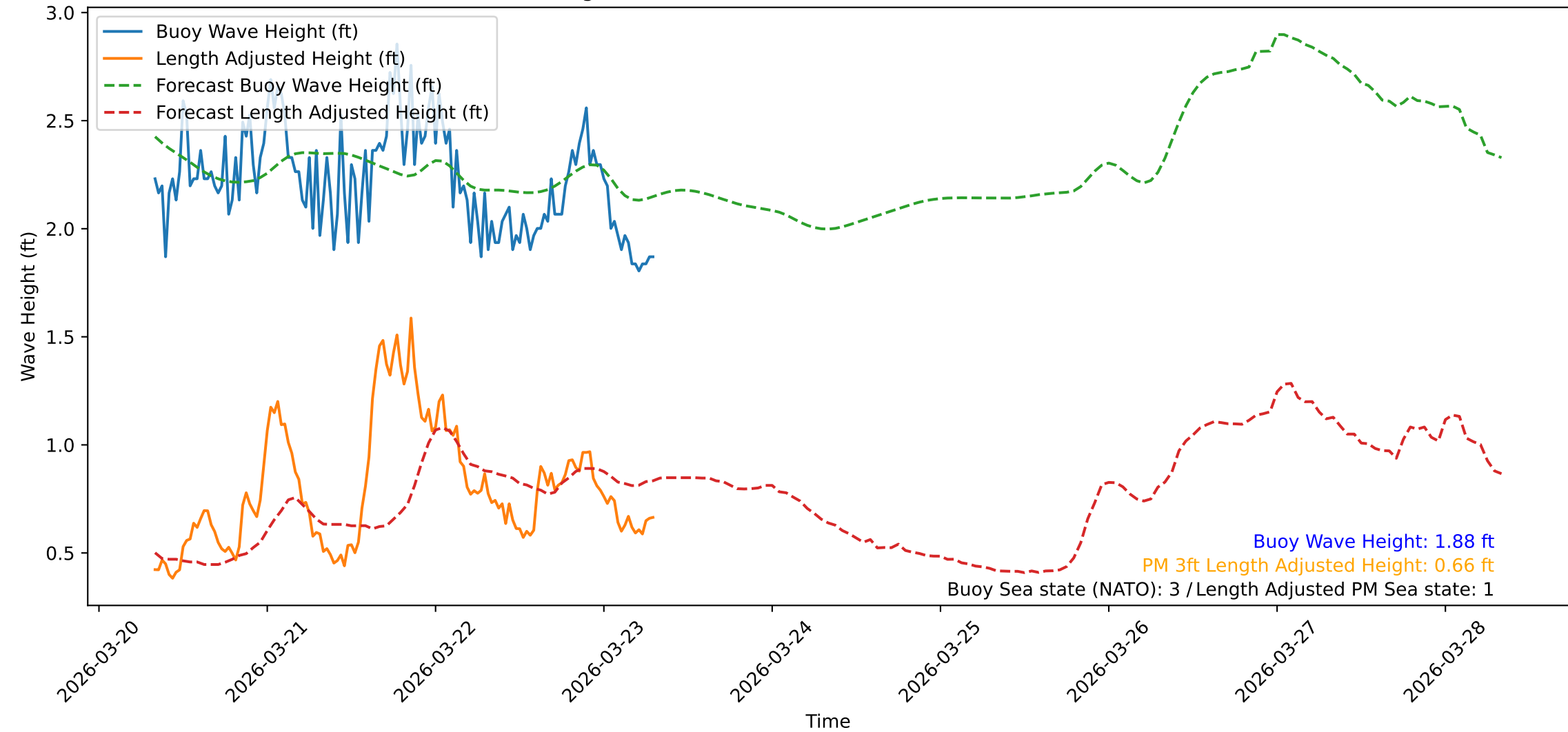
Wave Heights over Time for Red Beach at 2026-03-23 07:50:48
